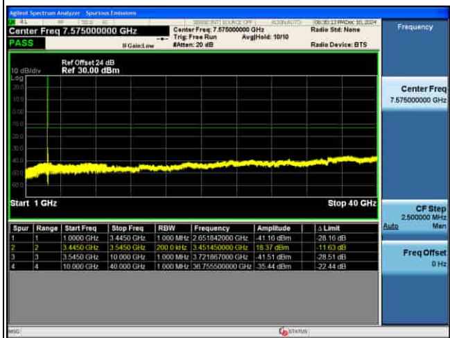
CSE_MIMO(ANT5)_n77(K)_30KHz_256QAM_90M CH633334_1RB@1_
