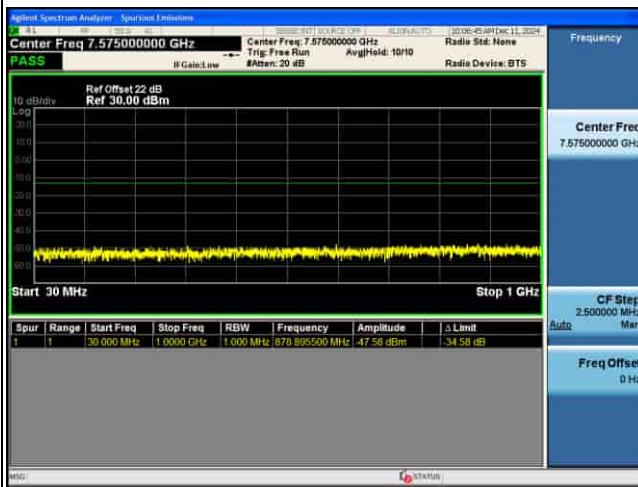
CSE_MIMO(ANT5)_n77(K)_30KHz_64QAM_80M CH634000_1RB@1_
