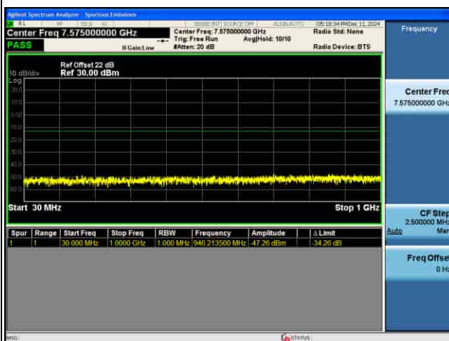
CSE_MIMO(ANT5)_n77(N)_30KHz_64QAM_20M CH664666_1RB@1_
