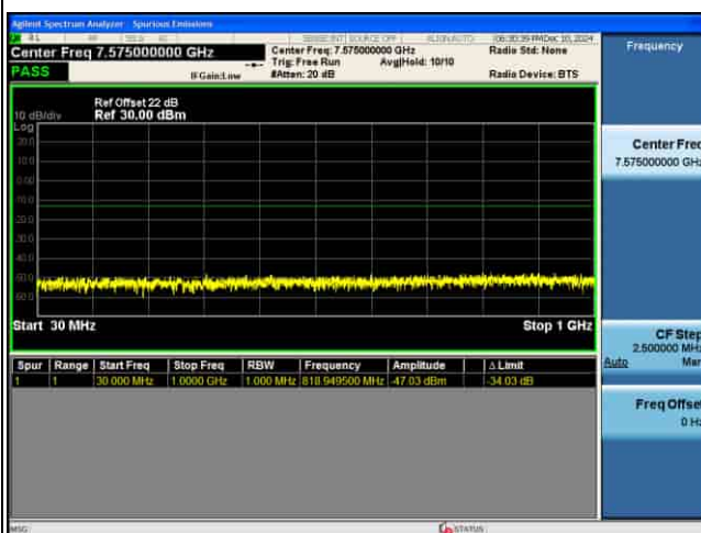
CSE_MIMO(ANT5)_n77(K)_30KHz_256QAM_90M CH633666_1RB@1
