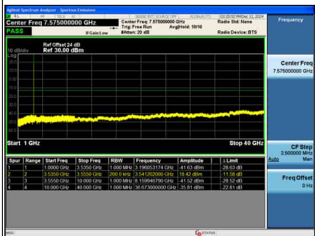
CSE_MIMO(ANT5)_n77(K)_30KHz_256QAM_10M CH636332_1RB@1_
