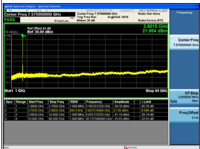
CSE_MIMO(ANT5)_n77(N)_30KHz_QPSK_80M CH662666_1RB@1_
