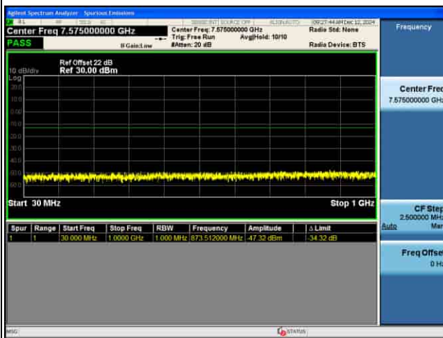
CSE_MIMO(ANT5)_n77(N)_30KHz_16QAM_90M CH656000_1RB@1_
