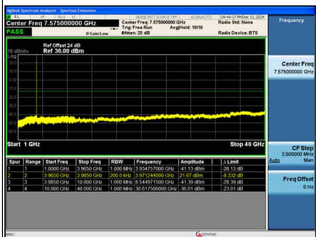
CSE_MIMO(ANT5)_n77(N)_30KHz_16QAM_10M CH665000_1RB@1_
