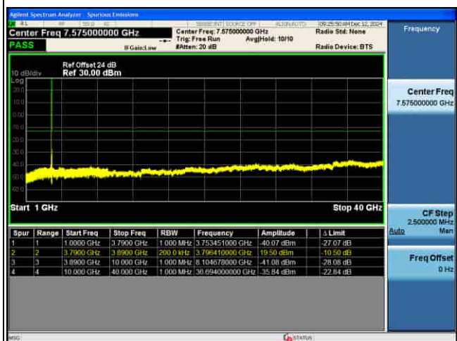
CSE_MIMO(ANT5)_n77(N)_30KHz_QPSK_90M CH662332_1RB@1_
