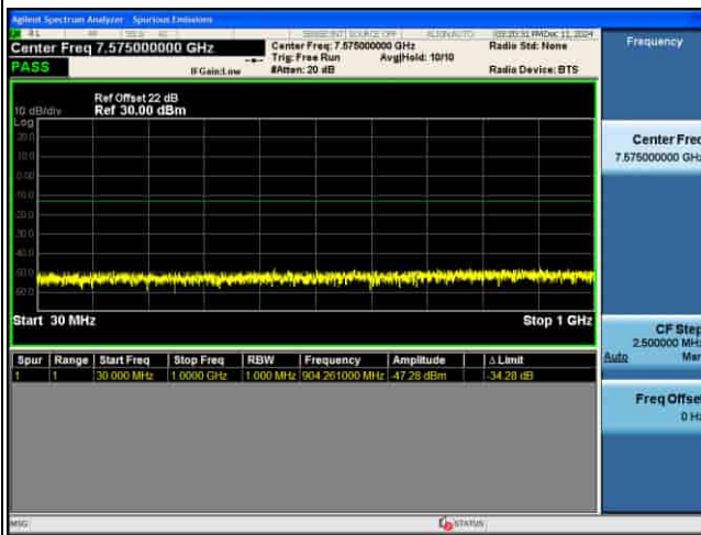
CSE_MIMO(ANT5)_n77(K)_30KHz_256QAM_10M CH633334_1RB@1
