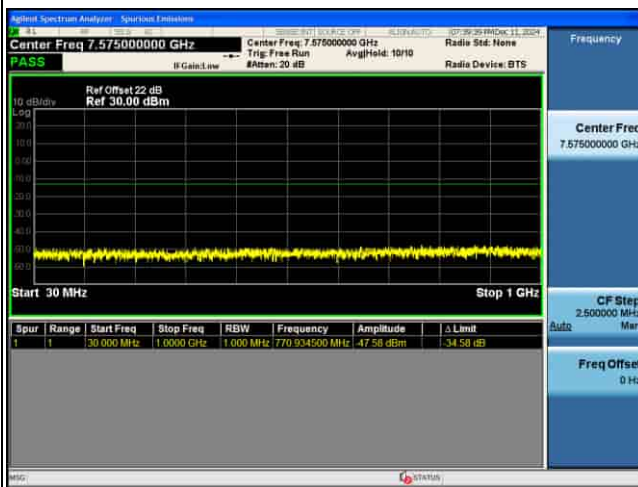
CSE_MIMO(ANT5)_n77(N)_30KHz_16QAM_70M CH656000_1RB@1_
