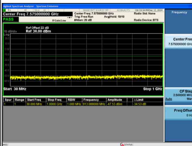
CSE_MIMO(ANT5)_n77(N)_30KHz_64QAM_40M CH664000_1RB@1_
