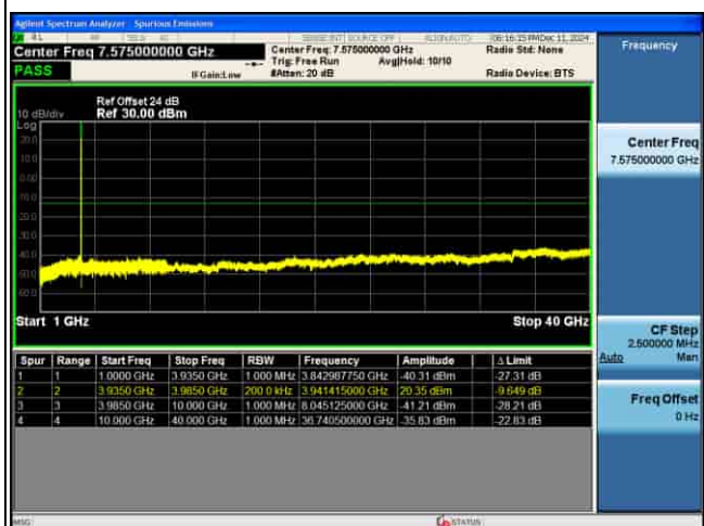
CSE_MIMO(ANT5)_n77(N)_30KHz_64QAM_40M CH664000_1RB@1_
