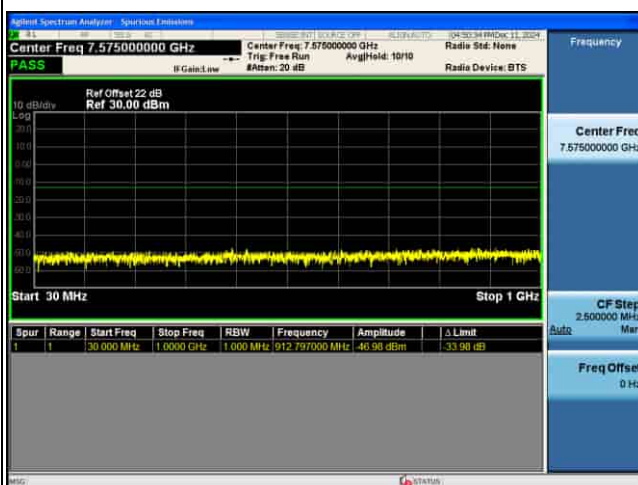
CSE_MIMO(ANT5)_n77(N)_30KHz_64QAM_10M CH665000_1RB@1_
