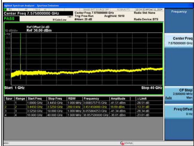
CSE_MIMO(ANT5)_n77(K)_30KHz_256QAM_70M CH633334_1RB@1_
