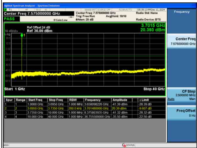
CSE_MIMO(ANT5)_n77(N)_30KHz_16QAM_30M CH656000_1RB@1_
