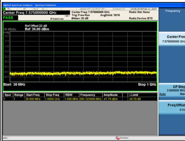
CSE_MIMO(ANT5)_n77(K)_30KHz_256QAM_60M CH633334_1RB@1
