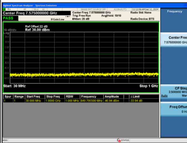
CSE_MIMO(ANT5)_n77(K)_30KHz_256QAM_50M CH633334_1RB@1
