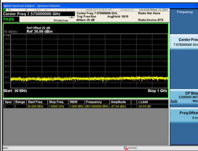
CSE_MIMO(ANT5)_n77(N)_30KHz_16QAM_10M CH656000_1RB@1_
