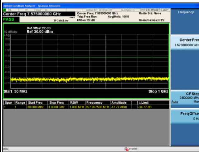
CSE_MIMO(ANT5)_n77(N)_30KHz_64QAM_15M CH656000_1RB@1_
