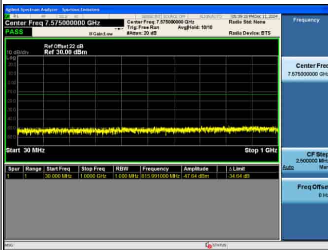
CSE_MIMO(ANT5)_n77(N)_30KHz_16QAM_30M CH656000_1RB@1_
