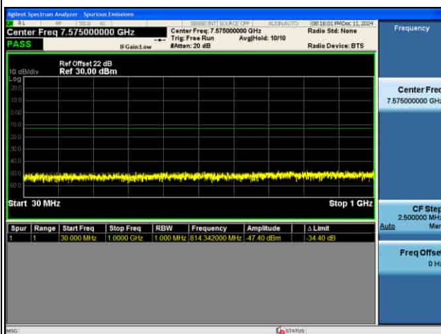
CSE_MIMO(ANT5)_n77(N)_30KHz_QPSK_80M CH662666_1RB@1_
