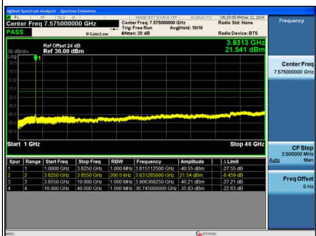
CSE_MIMO(ANT5)_n77(N)_30KHz_QPSK_20M CH664666_1RB@1_
