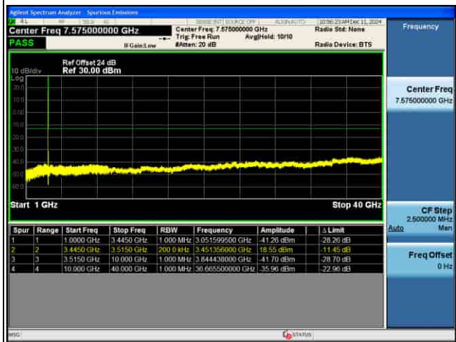
CSE_MIMO(ANT5)_n77(K)_30KHz_256QAM_60M CH633334_1RB@1_
