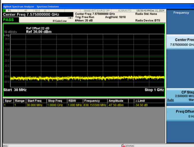
CSE_MIMO(ANT5)_n77(N)_30KHz_64QAM_30M CH664332_1RB@1_
