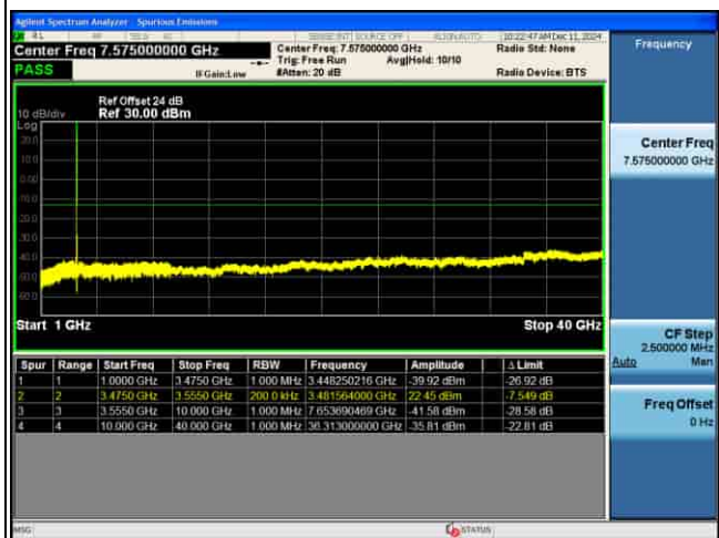
CSE_MIMO(ANT5)_n77(K)_30KHz_64QAM_80M CH632668_1RB@1_
