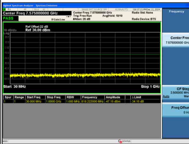
CSE_MIMO(ANT5)_n77(N)_30KHz_16QAM_50M CH656000_1RB@1_
