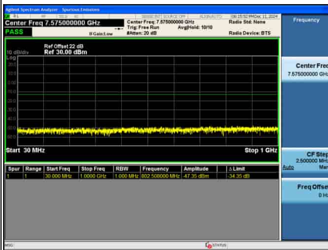
CSE_MIMO(ANT5)_n77(N)_30KHz_64QAM_40M CH656000_1RB@1_
