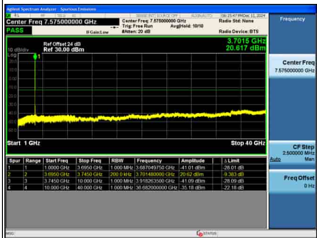
CSE_MIMO(ANT5)_n77(N)_30KHz_64QAM_40M CH656000_1RB@1_
