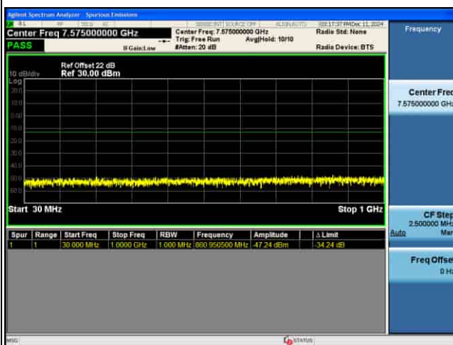
CSE_MIMO(ANT5)_n77(K)_30KHz_256QAM_20M CH636000_1RB@1
