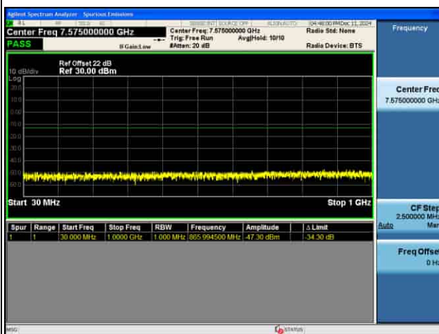
CSE_MIMO(ANT5)_n77(N)_30KHz_16QAM_10M CH665000_1RB@1_
