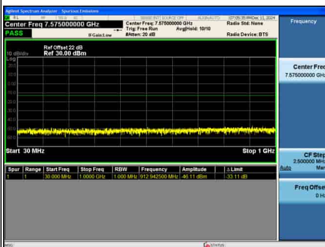
CSE_MIMO(ANT5)_n77(N)_30KHz_16QAM_60M CH663332_1RB@1_
