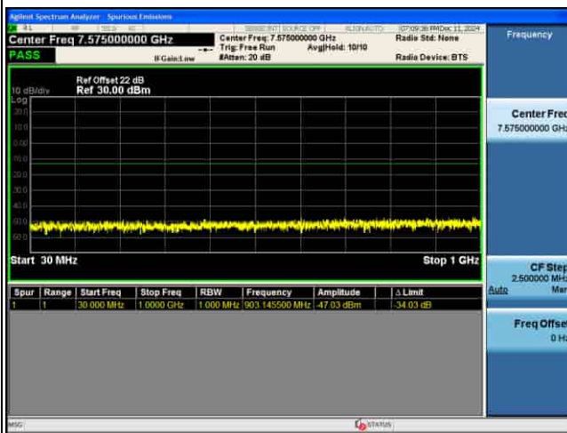
CSE_MIMO(ANT5)_n77(N)_30KHz_QPSK_60M CH656000_1RB@1_
