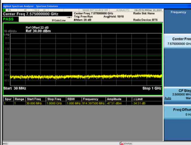
CSE_MIMO(ANT5)_n77(K)_30KHz_64QAM_100M CH633334_1RB@1_
