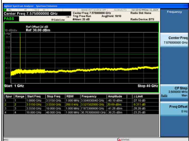
CSE_MIMO(ANT5)_n77(K)_30KHz_256QAM_30M CH635666_1RB@1_
