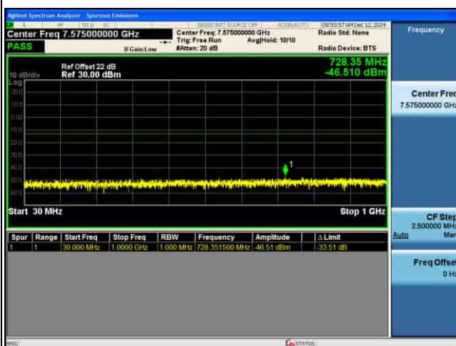
CSE_MIMO(ANT5)_n77(N)_30KHz_QPSK_90M CH662332_1RB@1_
