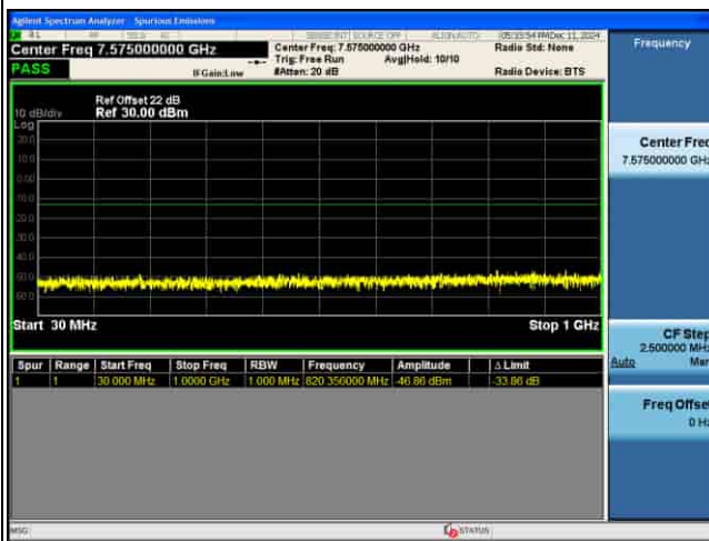
CSE_MIMO(ANT5)_n77(N)_30KHz_QPSK_30M CH656000_1RB@1_
