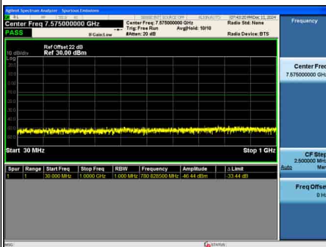
CSE_MIMO(ANT5)_n77(N)_30KHz_16QAM_70M CH663000_1RB@1_
