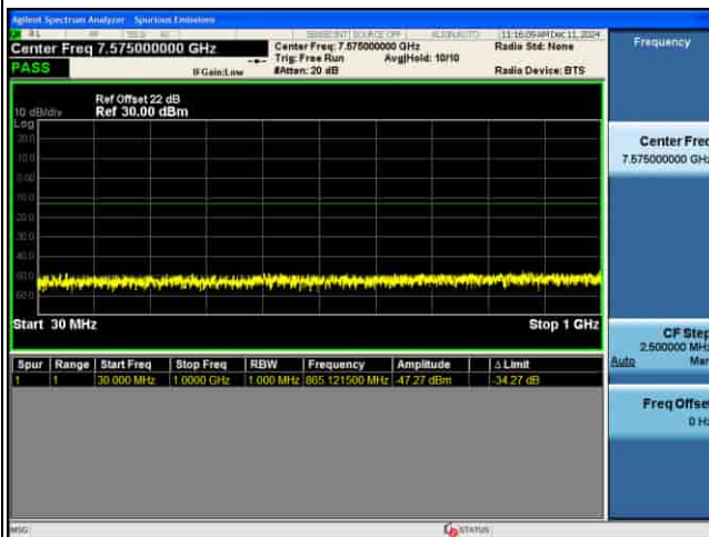
CSE_MIMO(ANT5)_n77(K)_30KHz_256QAM_50M CH635000_1RB@1
