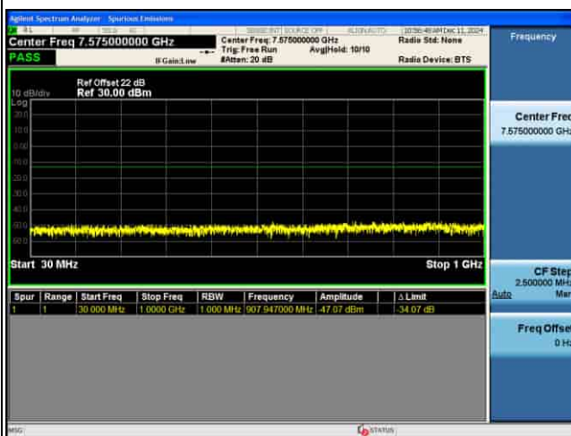
CSE_MIMO(ANT5)_n77(K)_30KHz_256QAM_60M CH634666_1RB@1
