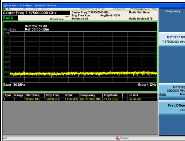
CSE_MIMO(ANT5)_n77(N)_30KHz_64QAM_30M CH656000_1RB@1_
