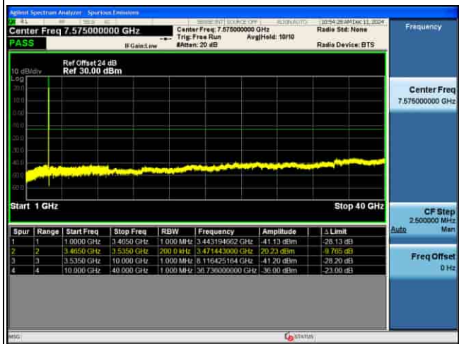
CSE_MIMO(ANT5)_n77(K)_30KHz_64QAM_60M CH634666_1RB@1_
