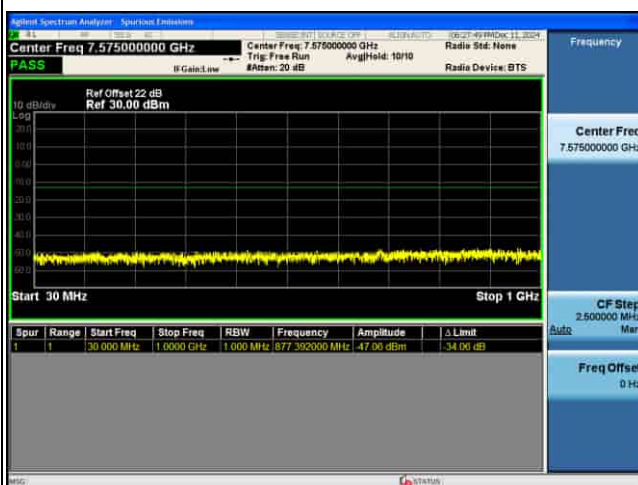
CSE_MIMO(ANT5)_n77(N)_30KHz_QPSK_40M CH664000_1RB@1_
