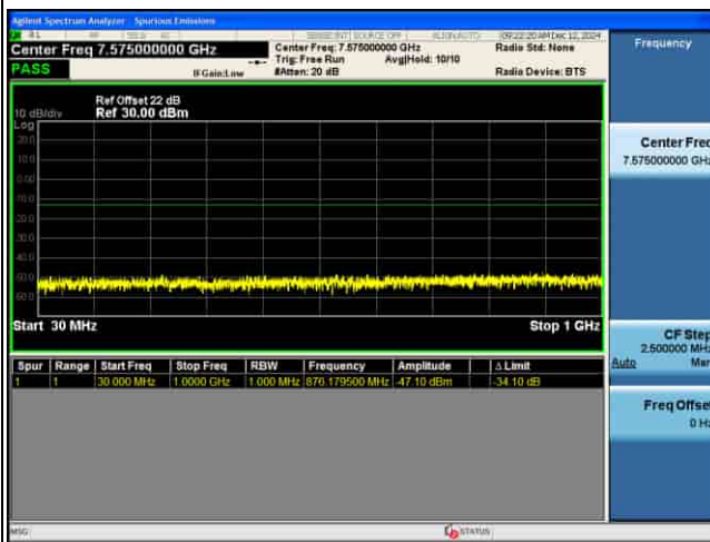
CSE_MIMO(ANT5)_n77(N)_30KHz_QPSK_90M CH656000_1RB@1_
