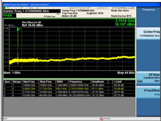
CSE_MIMO(ANT5)_n77(N)_30KHz_QPSK_70M CH656000_1RB@1_
