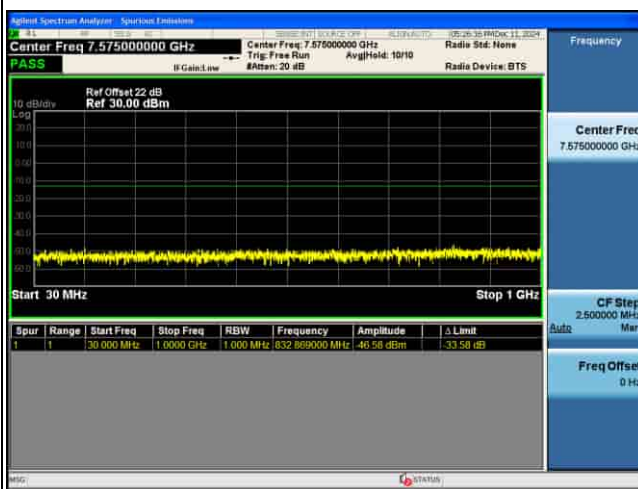
CSE_MIMO(ANT5)_n77(N)_30KHz_QPSK_20M CH656000_1RB@1_
