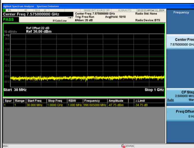
CSE_MIMO(ANT5)_n77(K)_30KHz_64QAM_70M CH632334_1RB@1_
