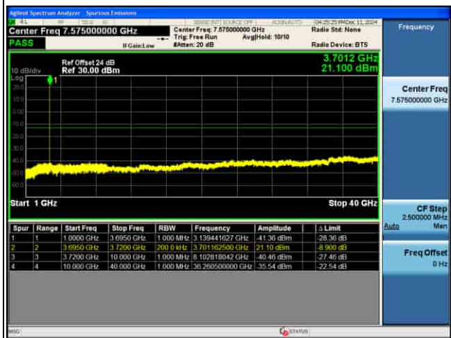
CSE_MIMO(ANT5)_n77(N)_30KHz_16QAM_15M CH656000_1RB@1_
