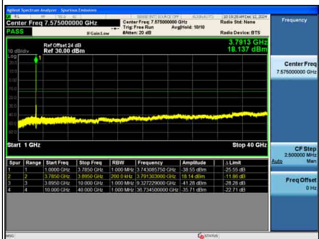
CSE_MIMO(ANT5)_n77(N)_30KHz_16QAM_100M CH662000_1RB@1_
