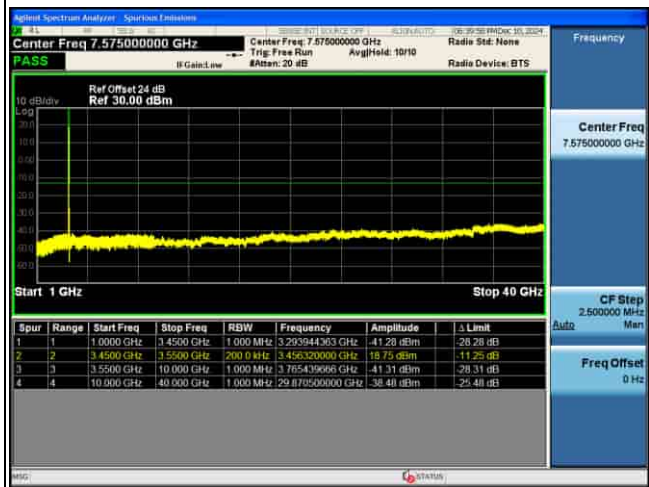
CSE_MIMO(ANT5)_n77(K)_30KHz_64QAM_90M CH633666_1RB@1_
