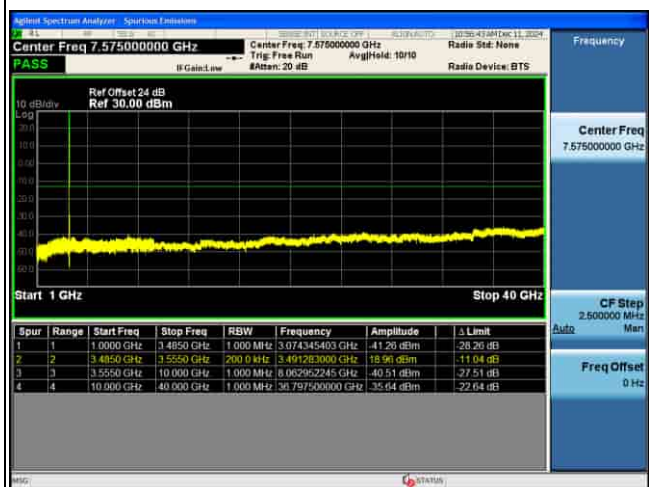
CSE_MIMO(ANT5)_n77(K)_30KHz_256QAM_60M CH634666_1RB@1_
