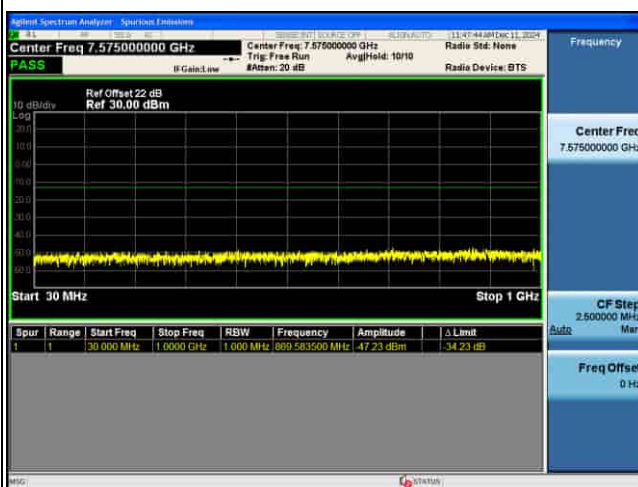
CSE_MIMO(ANT5)_n77(K)_30KHz_256QAM_40M CH635332_1RB@1
