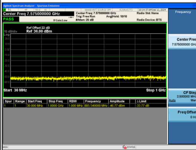
CSE_MIMO(ANT5)_n77(K)_30KHz_256QAM_70M CH633334_1RB@1
