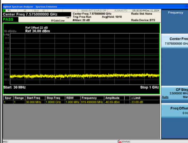
CSE_MIMO(ANT5)_n77(N)_30KHz_QPSK_20M CH664666_1RB@1_
