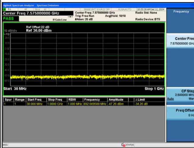
CSE_MIMO(ANT5)_n77(K)_30KHz_64QAM_70M CH634332_1RB@1_
