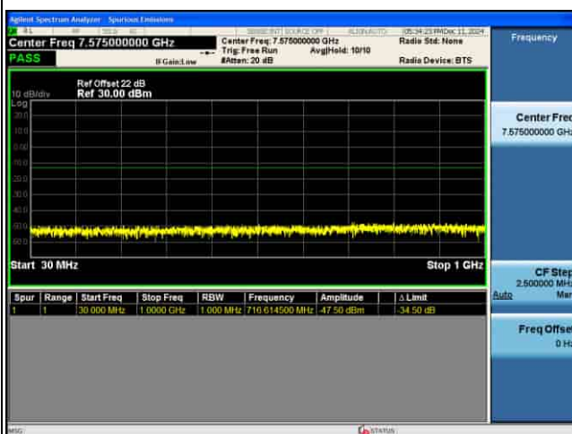
CSE_MIMO(ANT5)_n77(N)_30KHz_QPSK_30M CH664332_1RB@1_
