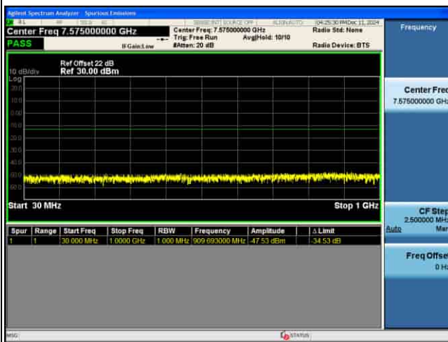
CSE_MIMO(ANT5)_n77(N)_30KHz_16QAM_15M CH656000_1RB@1_
