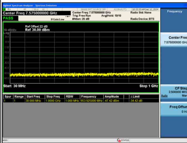
CSE_MIMO(ANT5)_n77(N)_30KHz_16QAM_100M CH656000_1RB@1
