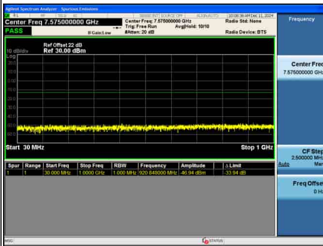
CSE_MIMO(ANT5)_n77(K)_30KHz_256QAM_80M CH633334_1RB@1
