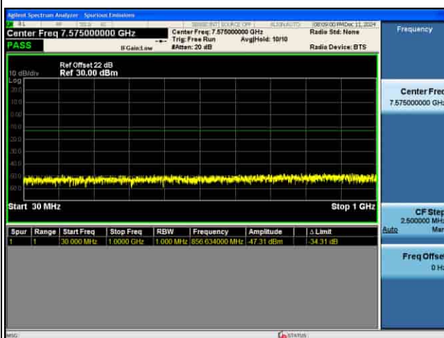
CSE_MIMO(ANT5)_n77(N)_30KHz_16QAM_80M CH662666_1RB@1_
