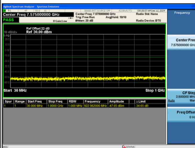
CSE_MIMO(ANT5)_n77(N)_30KHz_16QAM_90M CH662332_1RB@1_
