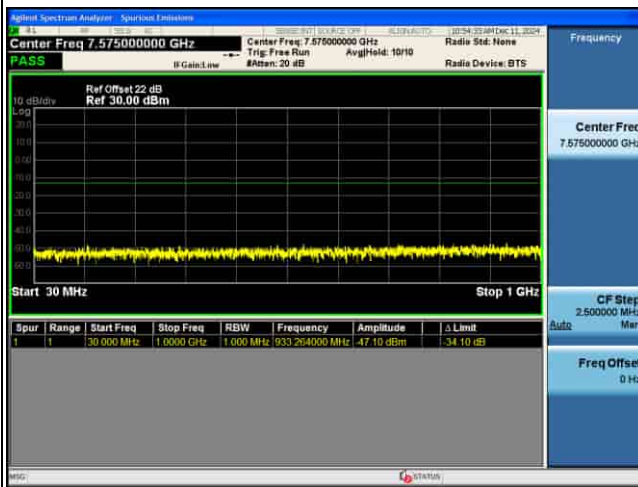
CSE_MIMO(ANT5)_n77(K)_30KHz_64QAM_60M CH634666_1RB@1_
