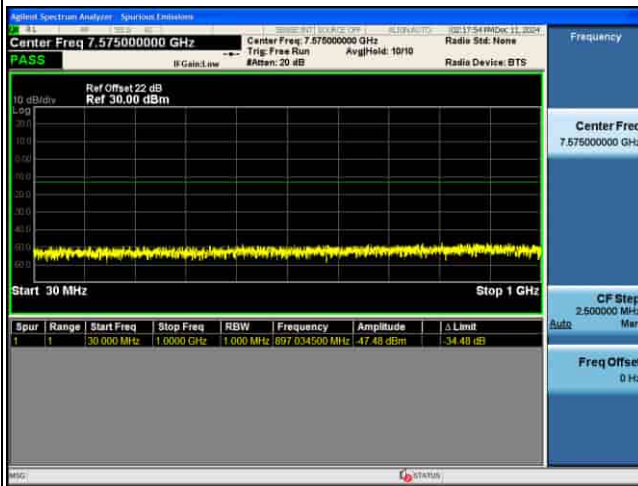
CSE_MIMO(ANT5)_n77(K)_30KHz_256QAM_30M CH633334_1RB@1
