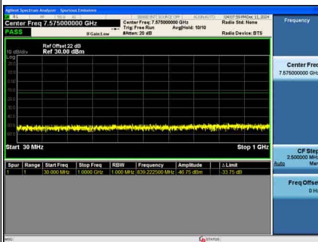
CSE_MIMO(ANT5)_n77(K)_30KHz_256QAM_15M CH636166_1RB@1
