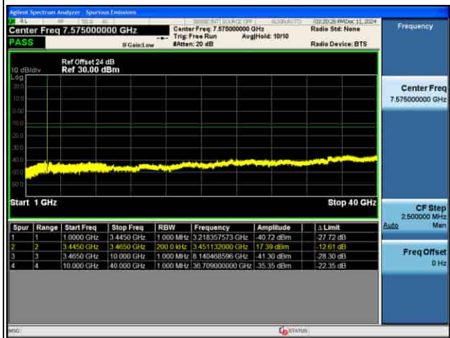
CSE_MIMO(ANT5)_n77(K)_30KHz_256QAM_10M CH633334_1RB@1_
