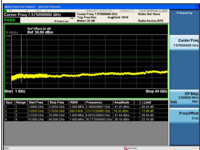
CSE_MIMO(ANT5)_n77(K)_30KHz_256QAM_40M CH635332_1RB@1_
