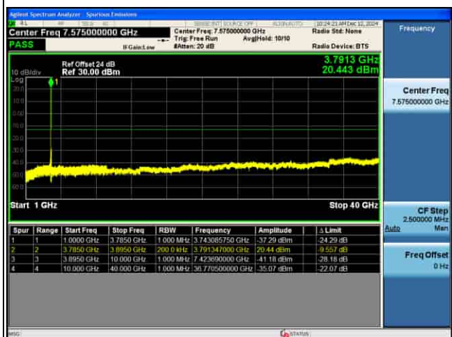
CSE_MIMO(ANT5)_n77(N)_30KHz_QPSK_100M CH662000_1RB@1_
