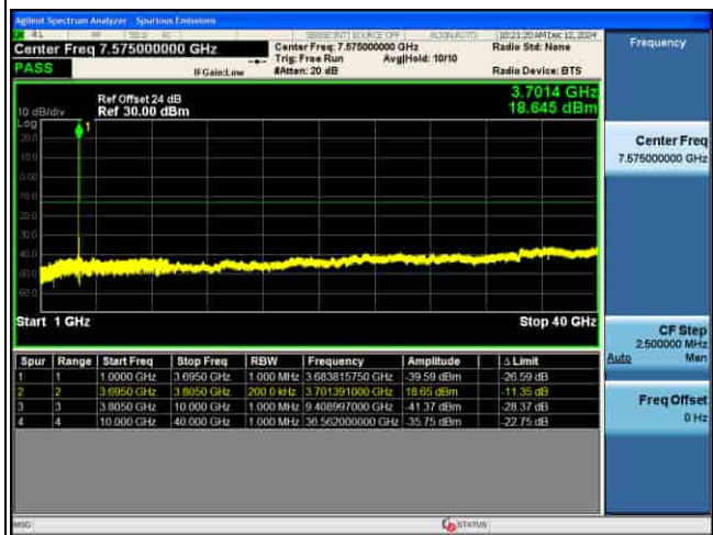
CSE_MIMO(ANT5)_n77(N)_30KHz_QPSK_100M CH656000_1RB@1_
