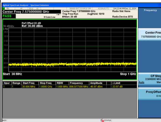
CSE_MIMO(ANT5)_n77(N)_30KHz_64QAM_15M CH664832_1RB@1_
