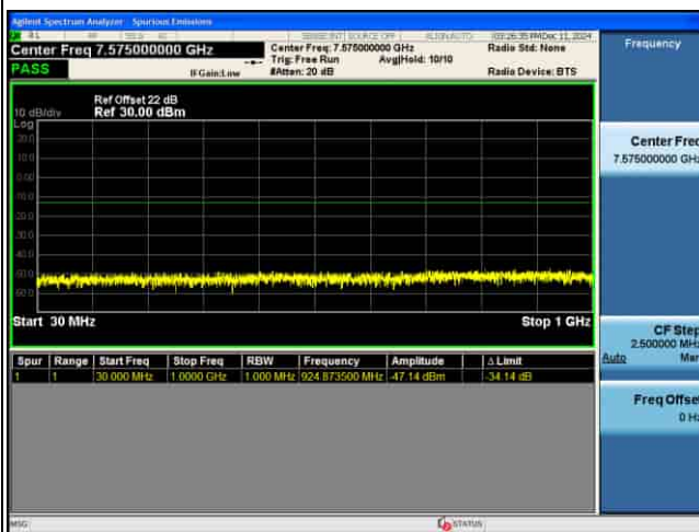
CSE_MIMO(ANT5)_n77(K)_30KHz_256QAM_10M CH636332_1RB@1
