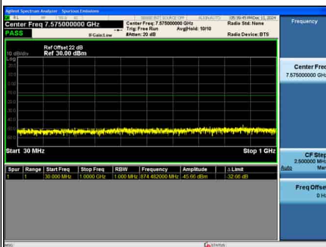
CSE_MIMO(ANT5)_n77(N)_30KHz_16QAM_30M CH664332_1RB@1_
