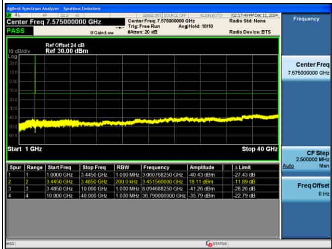
CSE_MIMO(ANT5)_n77(K)_30KHz_256QAM_30M CH633334_1RB@1_
