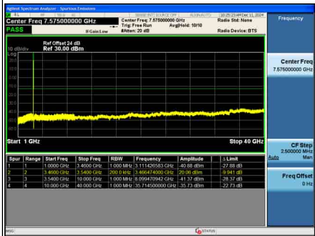
CSE_MIMO(ANT5)_n77(K)_30KHz_64QAM_70M CH634332_1RB@1_
