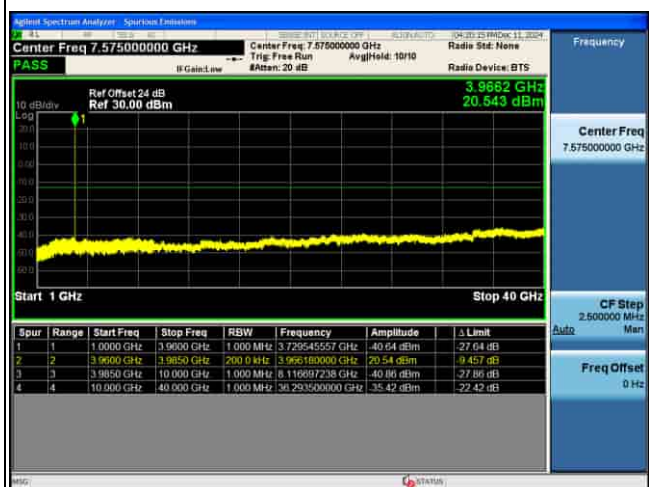
CSE_MIMO(ANT5)_n77(N)_30KHz_64QAM_15M CH664832_1RB@1_
