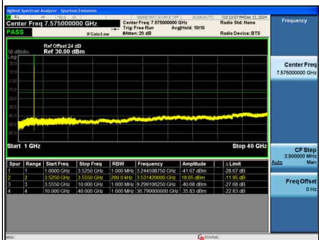
CSE_MIMO(ANT5)_n77(K)_30KHz_256QAM_20M CH636000_1RB@1_
