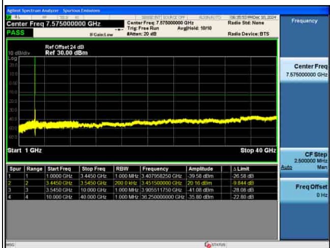
CSE_MIMO(ANT5)_n77(K)_30KHz_64QAM_90M CH633000_1RB@1_
