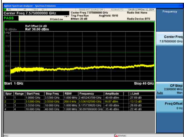
CSE_MIMO(ANT5)_n77(K)_30KHz_256QAM_15M CH636166_1RB@1_
