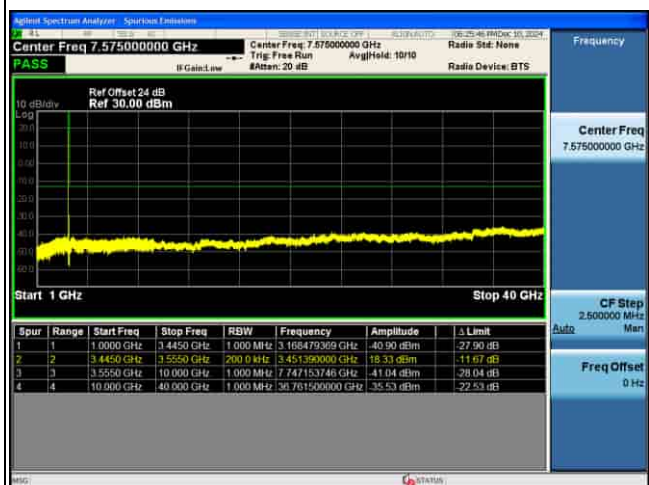
CSE_MIMO(ANT5)_n77(K)_30KHz_64QAM_100M CH633334_1RB@1_
