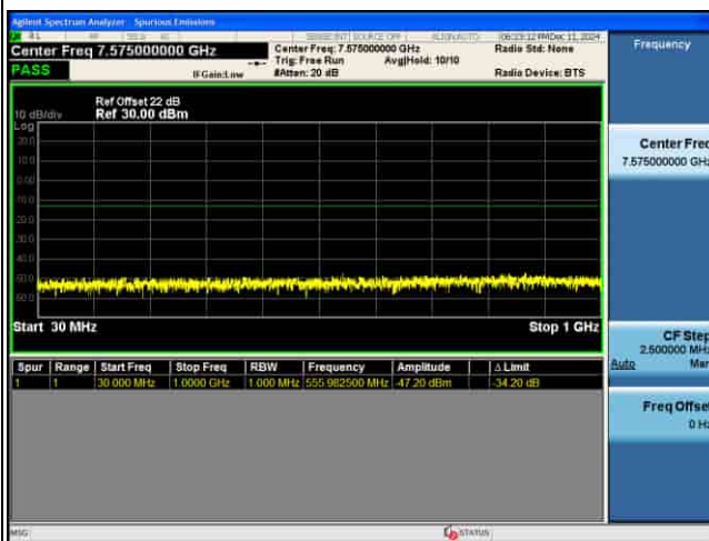
CSE_MIMO(ANT5)_n77(N)_30KHz_16QAM_40M CH664000_1RB@1_
