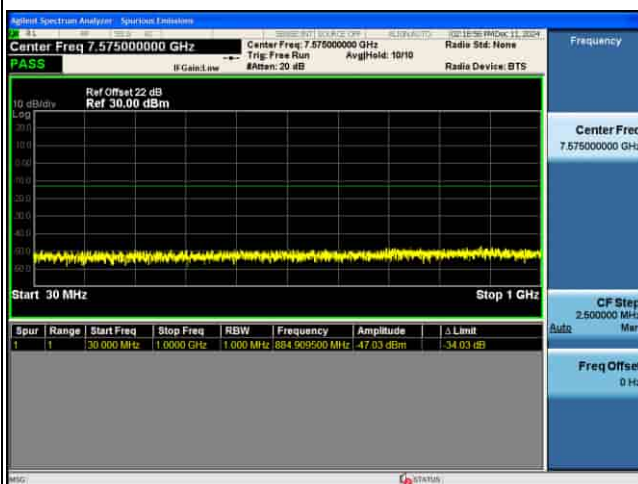
CSE_MIMO(ANT5)_n77(K)_30KHz_256QAM_30M CH635666_1RB@1
