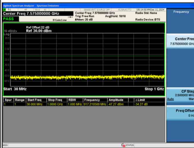
CSE_MIMO(ANT5)_n77(N)_30KHz_64QAM_20M CH656000_1RB@1_
