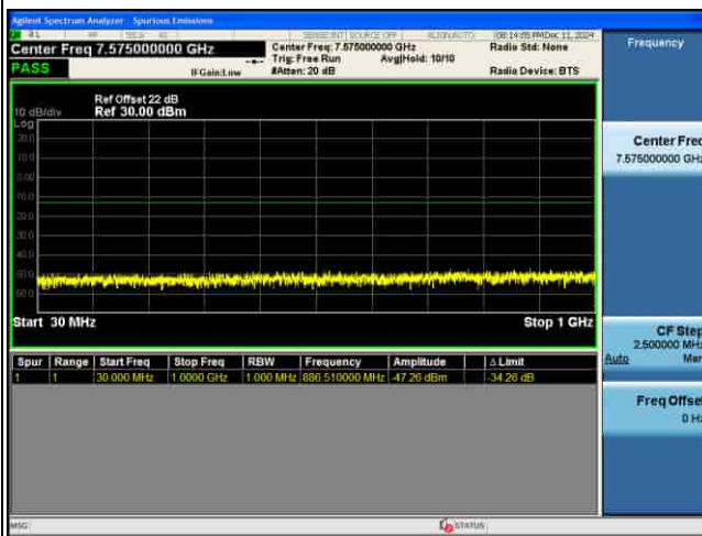
CSE_MIMO(ANT5)_n77(N)_30KHz_QPSK_80M CH656000_1RB@1_
