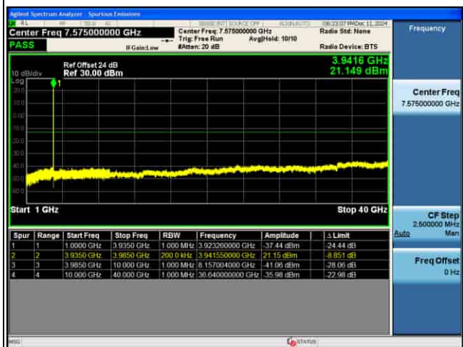
CSE_MIMO(ANT5)_n77(N)_30KHz_16QAM_40M CH664000_1RB@1_
