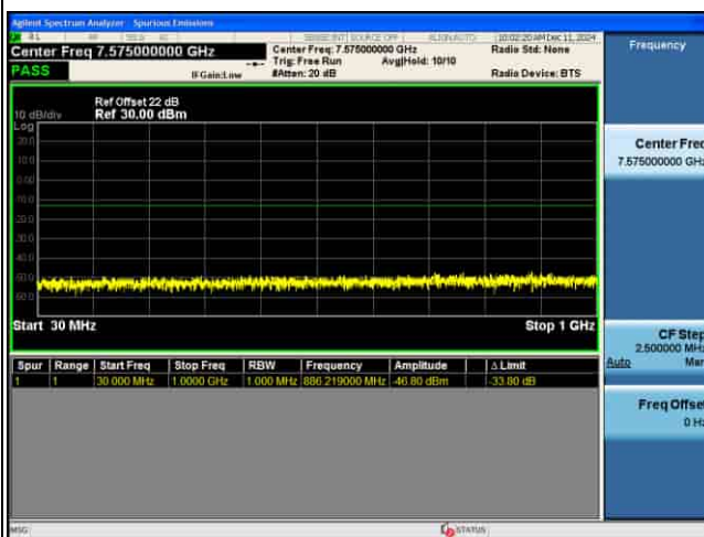
CSE_MIMO(ANT5)_n77(K)_30KHz_64QAM_80M CH632668_1RB@1_
