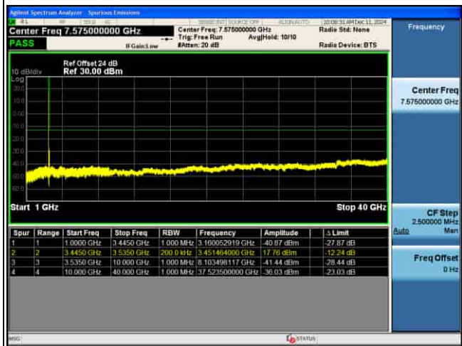
CSE_MIMO(ANT5)_n77(K)_30KHz_256QAM_80M CH633334_1RB@1_
