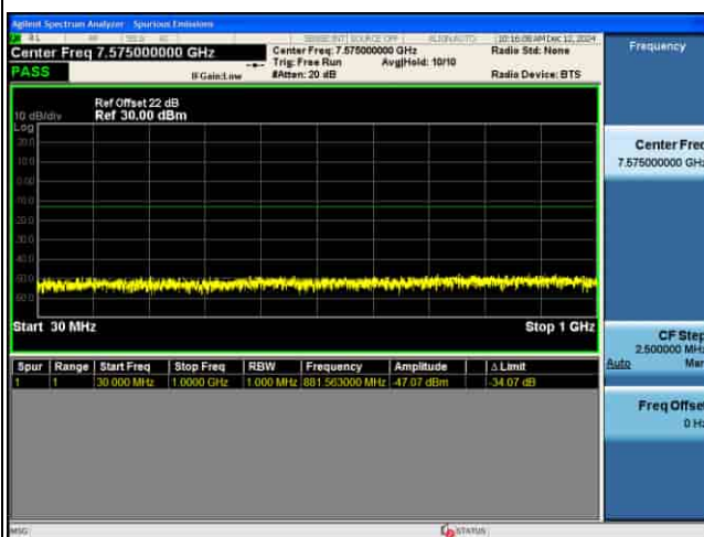
CSE_MIMO(ANT5)_n77(N)_30KHz_16QAM_100M CH662000_1RB@1
