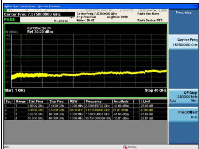
CSE_MIMO(ANT5)_n77(K)_30KHz_64QAM_70M CH632334_1RB@1_
