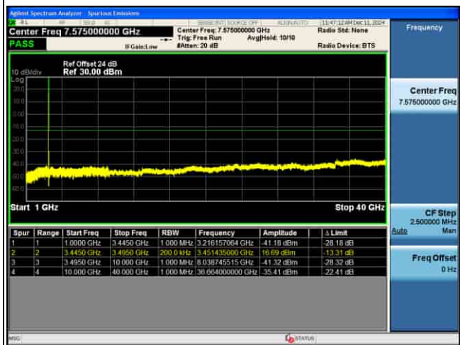
CSE_MIMO(ANT5)_n77(K)_30KHz_256QAM_40M CH633334_1RB@1_
