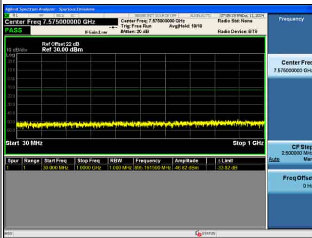
CSE_MIMO(ANT5)_n77(N)_30KHz_16QAM_60M CH656000_1RB@1_
