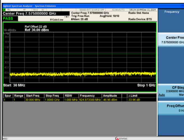
CSE_MIMO(ANT5)_n77(N)_30KHz_16QAM_20M CH664666_1RB@1_
