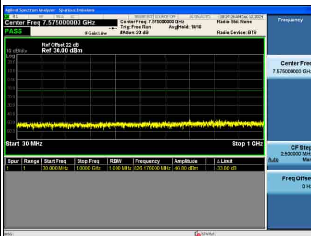
CSE_MIMO(ANT5)_n77(N)_30KHz_QPSK_100M CH662000_1RB@1_
