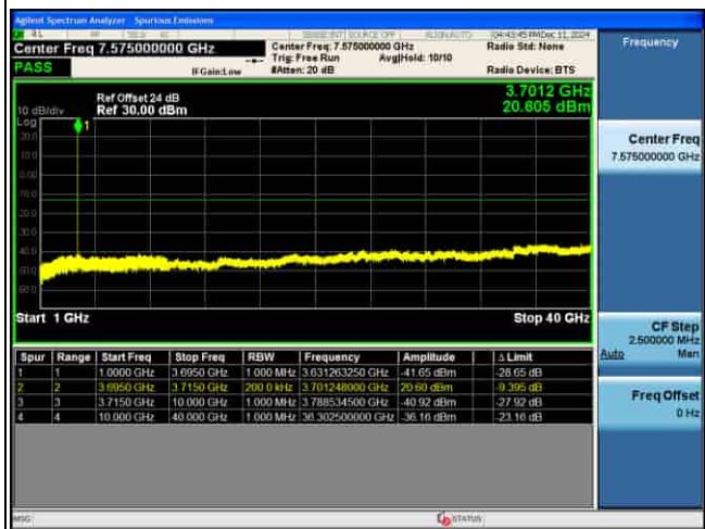
CSE_MIMO(ANT5)_n77(N)_30KHz_16QAM_10M CH656000_1RB@1_
