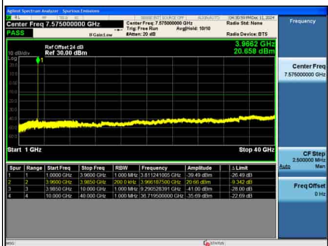
CSE_MIMO(ANT5)_n77(N)_30KHz_QPSK_15M CH664832_1RB@1_
