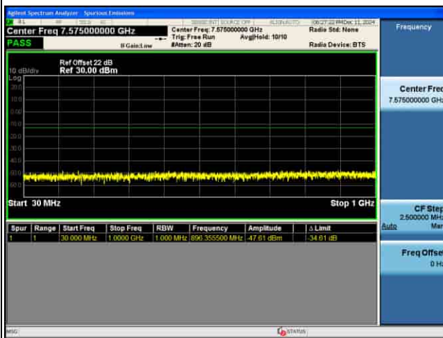
CSE_MIMO(ANT5)_n77(N)_30KHz_QPSK_40M CH656000_1RB@1_
