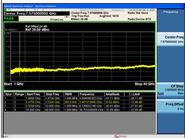
CSE_MIMO(ANT5)_n77(K)_30KHz_256QAM_70M CH634332_1RB@1_
