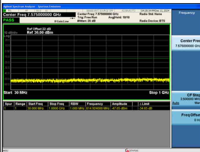
CSE_MIMO(ANT5)_n77(N)_30KHz_16QAM_15M CH664832_1RB@1_
