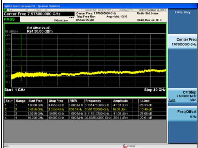
CSE_MIMO(ANT5)_n77(K)_30KHz_256QAM_50M CH635000_1RB@1_
