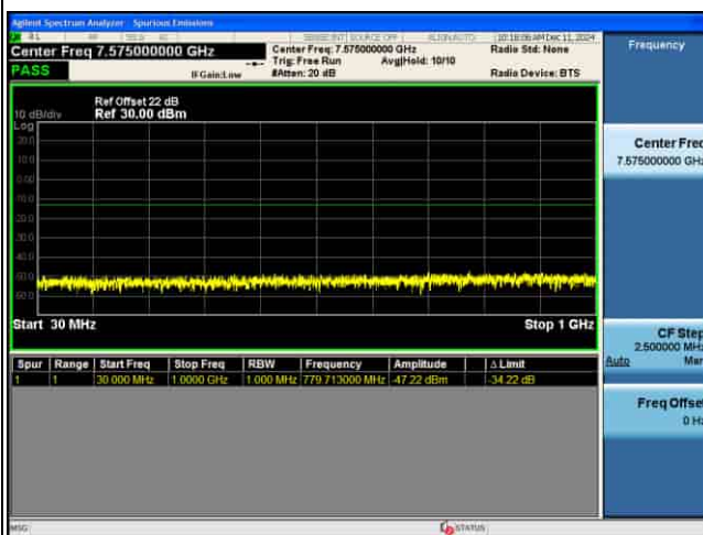
CSE_MIMO(ANT5)_n77(K)_30KHz_256QAM_70M CH634332_1RB@1
