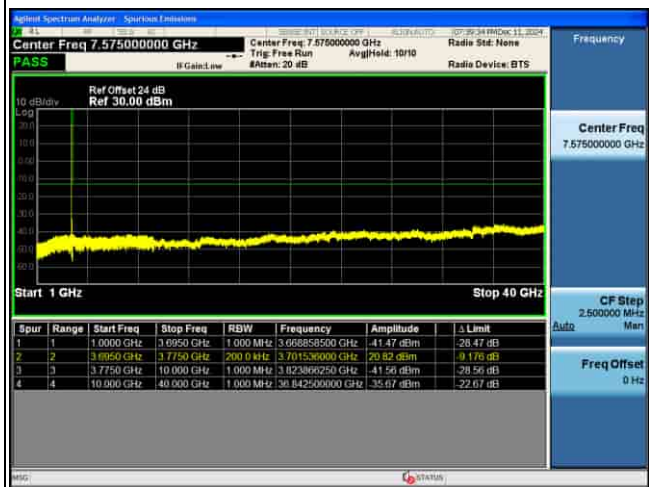
CSE_MIMO(ANT5)_n77(N)_30KHz_16QAM_70M CH656000_1RB@1_
