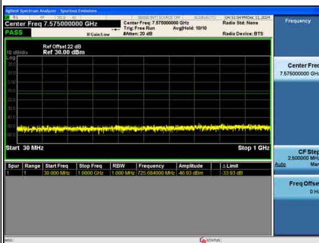
CSE_MIMO(ANT5)_n77(N)_30KHz_QPSK_15M CH664832_1RB@1_
