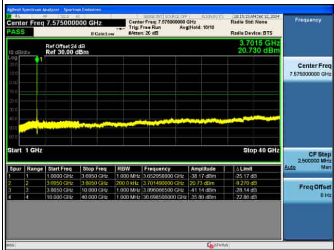
CSE_MIMO(ANT5)_n77(N)_30KHz_16QAM_100M CH656000_1RB@1_
