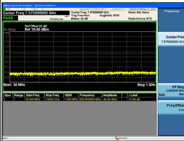
CSE_MIMO(ANT5)_n77(N)_30KHz_16QAM_80M CH656000_1RB@1_
