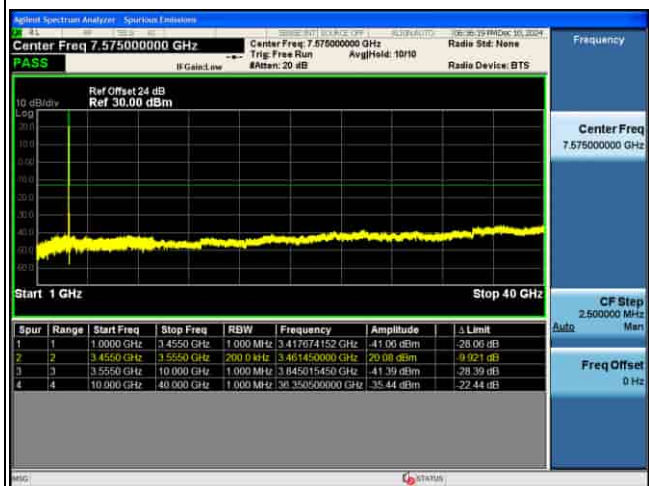
CSE_MIMO(ANT5)_n77(K)_30KHz_64QAM_100M CH633334_1RB@1_
