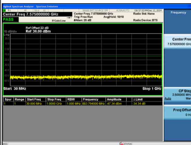
CSE_MIMO(ANT5)_n77(N)_30KHz_16QAM_50M CH663666_1RB@1_
