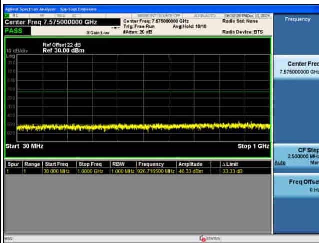
CSE_MIMO(ANT5)_n77(N)_30KHz_QPSK_50M CH656000_1RB@1_
