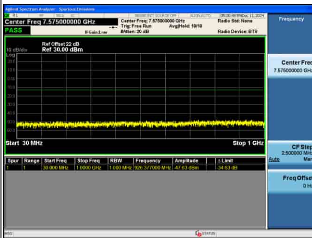
CSE_MIMO(ANT5)_n77(N)_30KHz_16QAM_20M CH656000_1RB@1_
