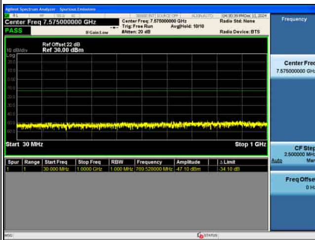
CSE_MIMO(ANT5)_n77(N)_30KHz_QPSK_15M CH656000_1RB@1_
