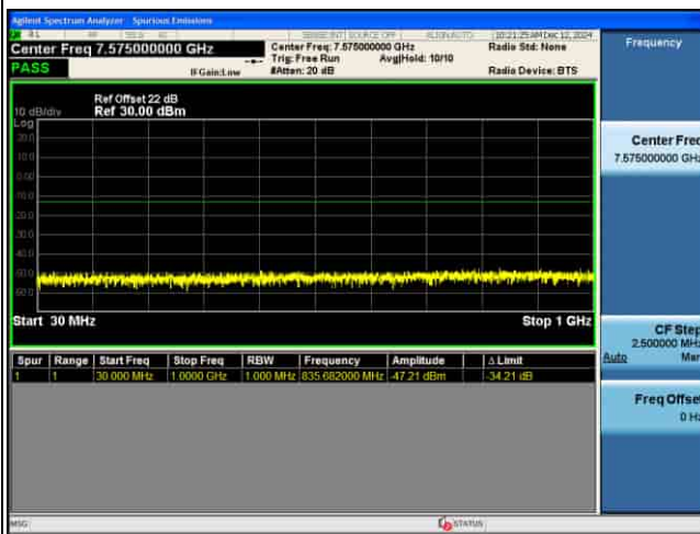
CSE_MIMO(ANT5)_n77(N)_30KHz_QPSK_100M CH656000_1RB@1_
