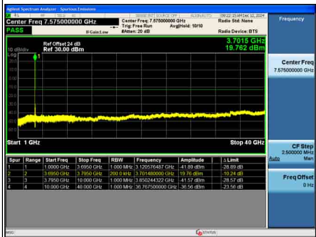
CSE_MIMO(ANT5)_n77(N)_30KHz_QPSK_90M CH656000_1RB@1_
