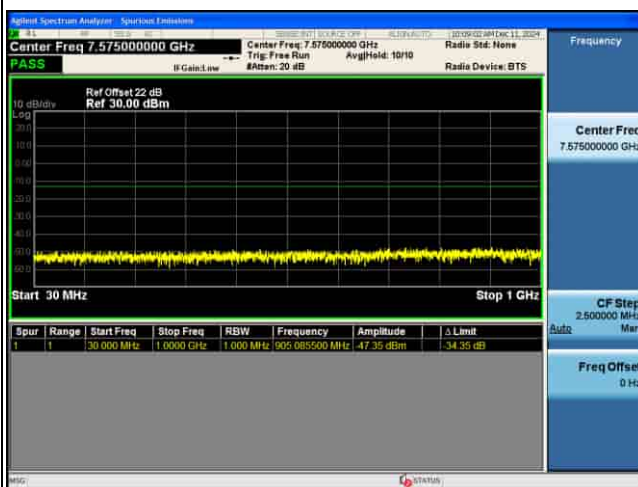
CSE_MIMO(ANT5)_n77(K)_30KHz_256QAM_80M CH634000_1RB@1
