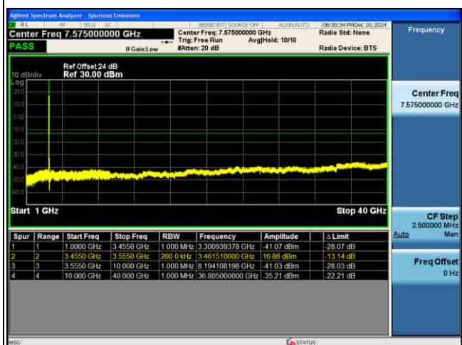
CSE_MIMO(ANT5)_n77(K)_30KHz_256QAM_90M CH633666_1RB@1_
