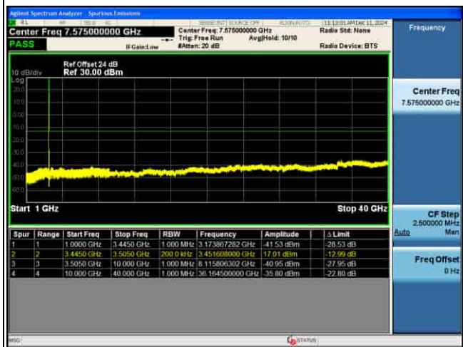
CSE_MIMO(ANT5)_n77(K)_30KHz_256QAM_50M CH633334_1RB@1_
