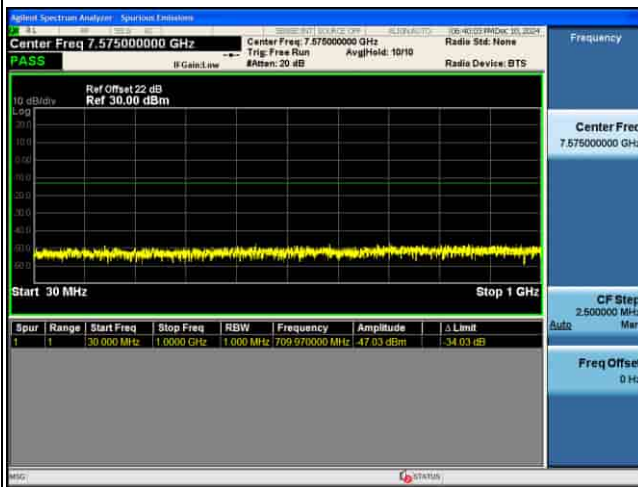
CSE_MIMO(ANT5)_n77(K)_30KHz_64QAM_90M CH633666_1RB@1_
