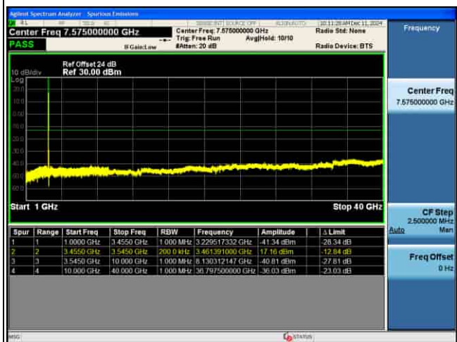
CSE_MIMO(ANT5)_n77(K)_30KHz_256QAM_80M CH634000_1RB@1_
