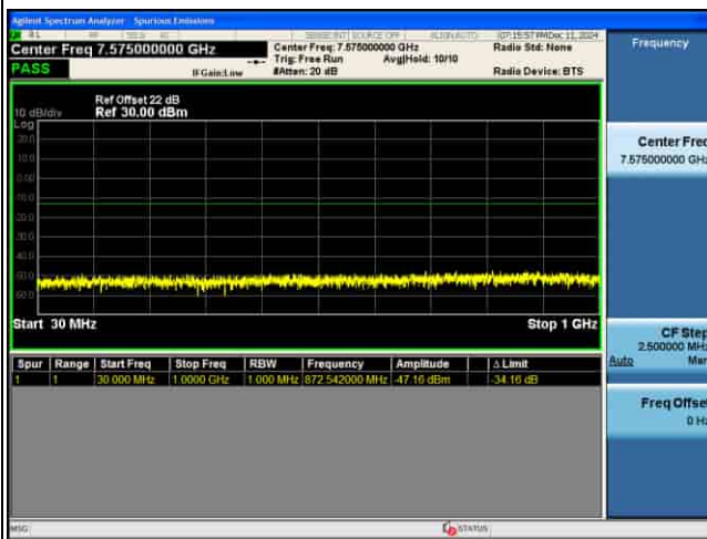
CSE_MIMO(ANT5)_n77(N)_30KHz_QPSK_70M CH656000_1RB@1_
