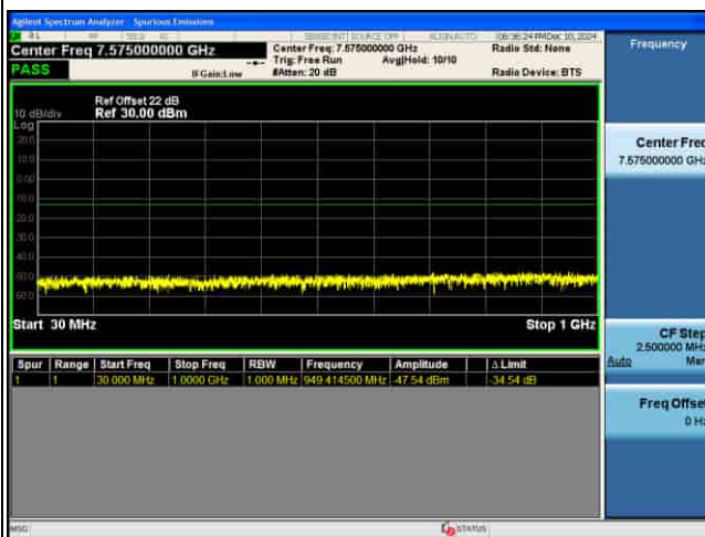
CSE_MIMO(ANT5)_n77(K)_30KHz_64QAM_100M CH633334_1RB@1_
