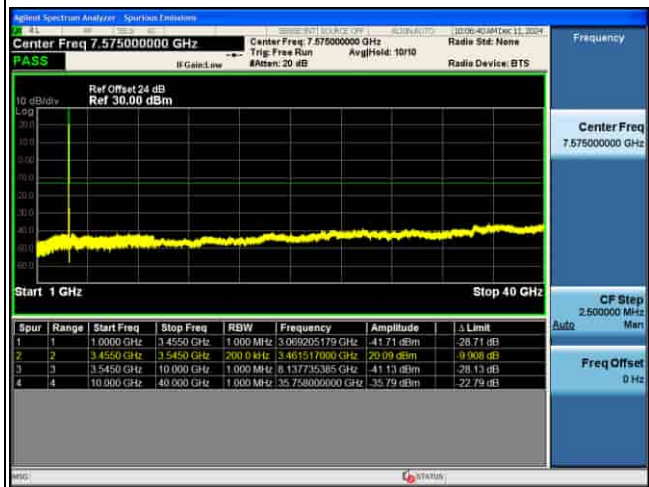
CSE_MIMO(ANT5)_n77(K)_30KHz_64QAM_80M CH634000_1RB@1_
