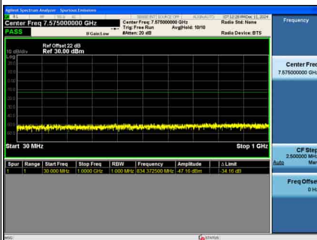
CSE_MIMO(ANT5)_n77(N)_30KHz_QPSK_60M CH663332_1RB@1_
