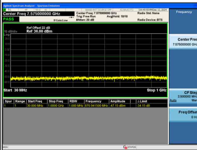
CSE_MIMO(ANT5)_n77(N)_30KHz_64QAM_10M CH656000_1RB@1_
