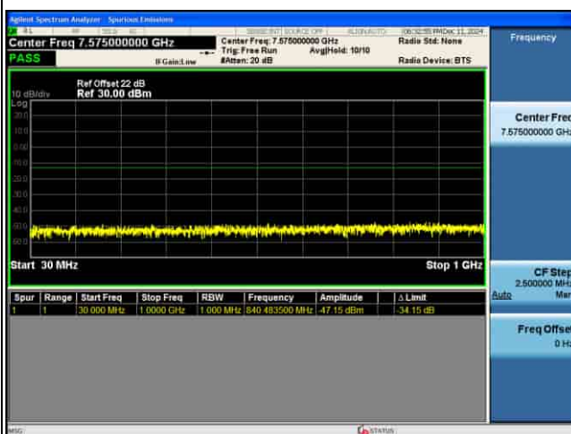
CSE_MIMO(ANT5)_n77(N)_30KHz_QPSK_50M CH663666_1RB@1_
