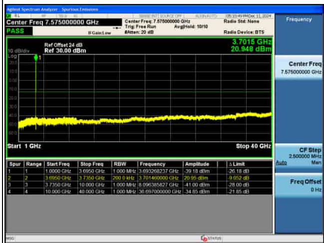
CSE_MIMO(ANT5)_n77(N)_30KHz_QPSK_30M CH656000_1RB@1_
