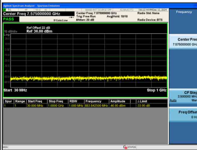
CSE_MIMO(ANT5)_n77(N)_30KHz_16QAM_40M CH656000_1RB@1_
