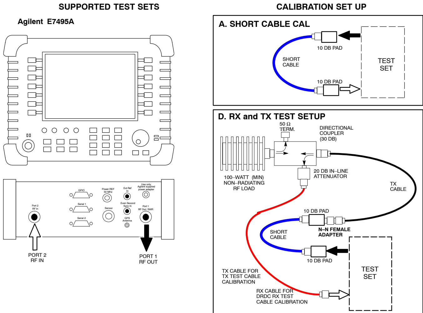
Figure 3-15: CDMA2000 1X Cable Calibration Test Setup – Agilent E7495A
