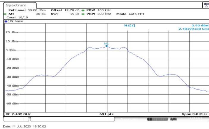
BLE_1M_Ant2_2402_0-Reference
