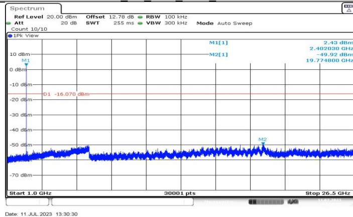
BLE_1M_Ant2_2402_1000-26500
