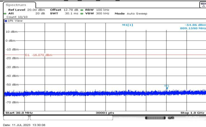
BLE_1M_Ant2_2402_30-1000
