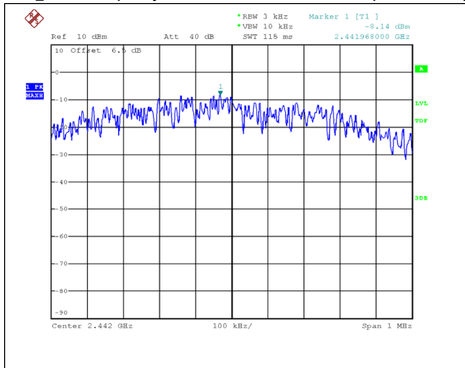
BLE _ Middle frequency Peak Power Spectral Density
