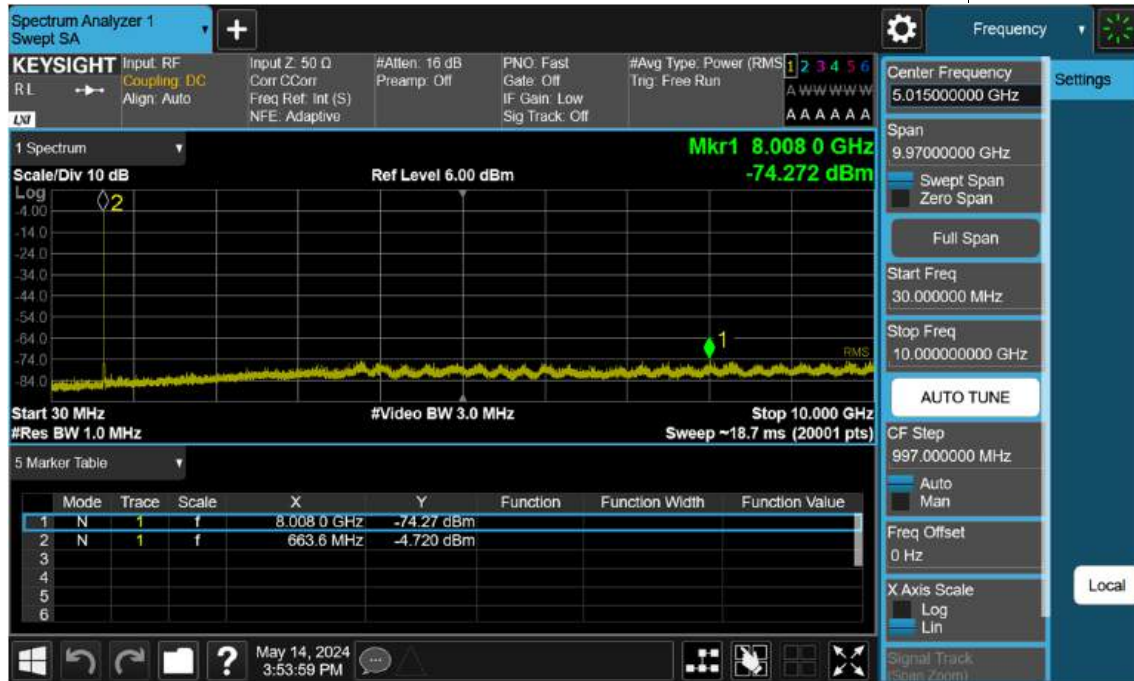
Sub6 n71. Conducted Spurious Plot _ (133100ch_5 MHz_BPSK_RB 1_1)
