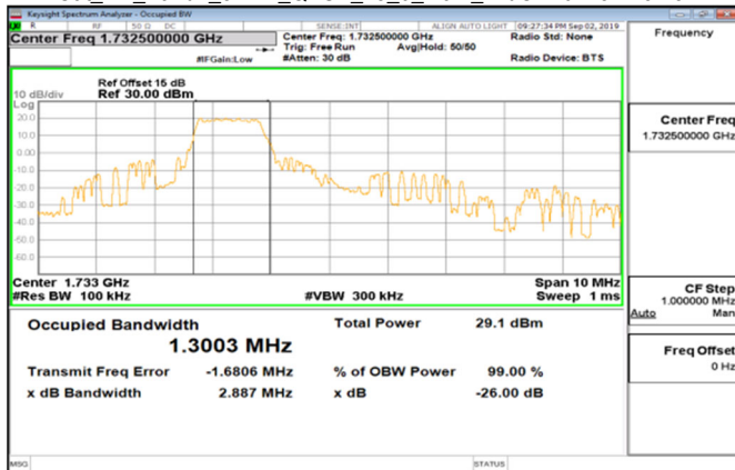
Cat_M1_Band4_5MHz_QPSK_25_0_Main_MidCH20175-1732.5
