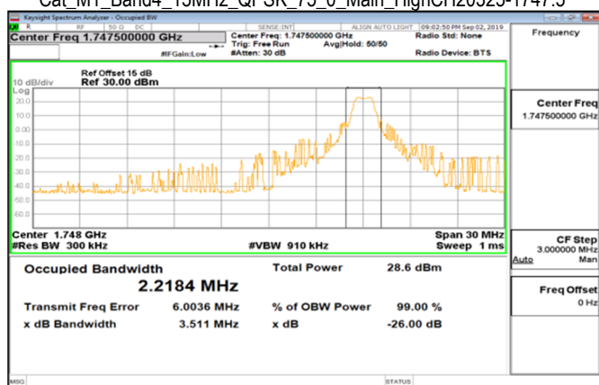
Cat_M1_Band4_15MHz_QPSK_75_0_Main_HighCH20325-1747.5
