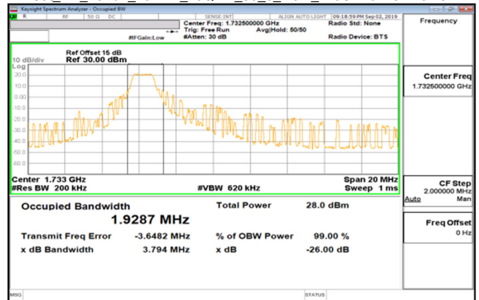
Cat_M1_Band4_10MHz_16QAM_50_0_Main_MidCH20175-1732.5
