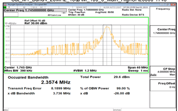
Cat M1_Band4_20MHz_16QAM_100_0_Main_HighCH20300-1745
