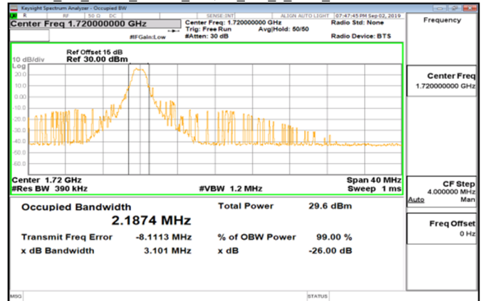
Cat M1_Band4_20MHz_16QAM_100_0_Main_LowCH20050-1720
