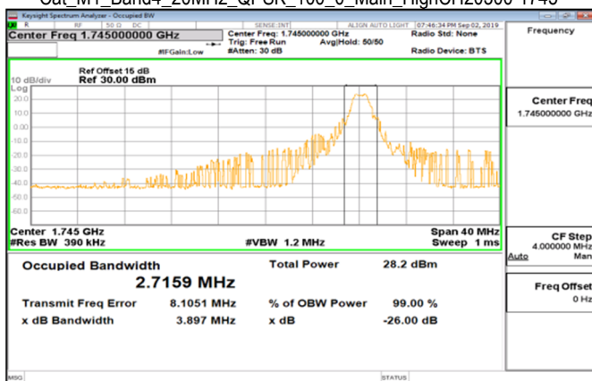
Cat M1_Band4_20MHz_QPSK_100_0_Main_HighCH20300-1745
