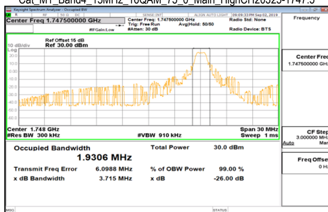
Cat_M1_Band4_15MHz_16QAM_75_0_Main_HighCH20325-1747.5
