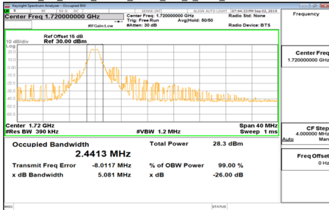
Cat M1_Band4_20MHz_QPSK_100_0_Main_LowCH20050-1720
