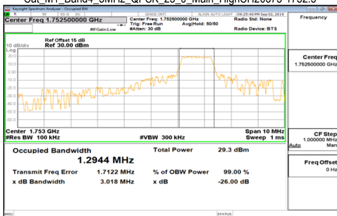
Cat_M1_Band4_5MHz_QPSK_25_0_Main_HighCH20375-1752.5
