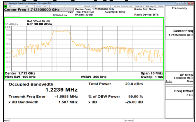
Cat_M1_Band4_5MHz_16QAM_25_0_Main_LowCH19975-1712.5
