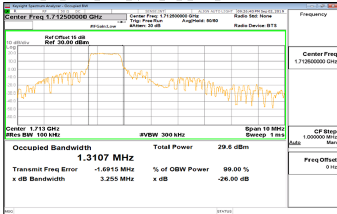
Cat_M1_Band4_5MHz_QPSK_25_0_Main_LowCH19975-1712.5
