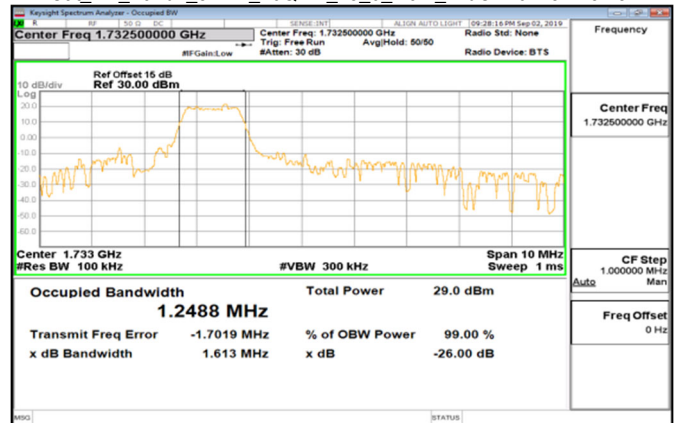
Cat_M1_Band4_5MHz_16QAM_25_0_Main_MidCH20175-1732.5
