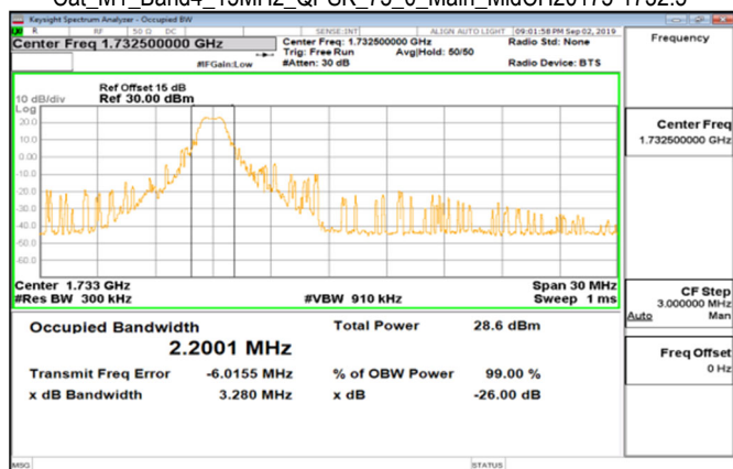
Cat_M1_Band4_15MHz_QPSK_75_0_Main_MidCH20175-1732.5
