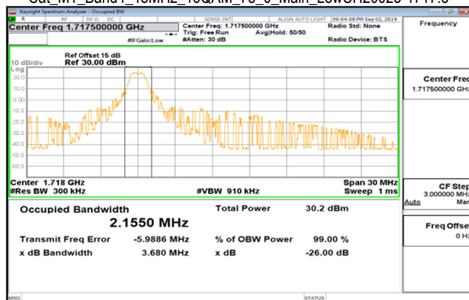
Cat_M1_Band4_15MHz_16QAM_75_0_Main_LowCH20025-1717.5
