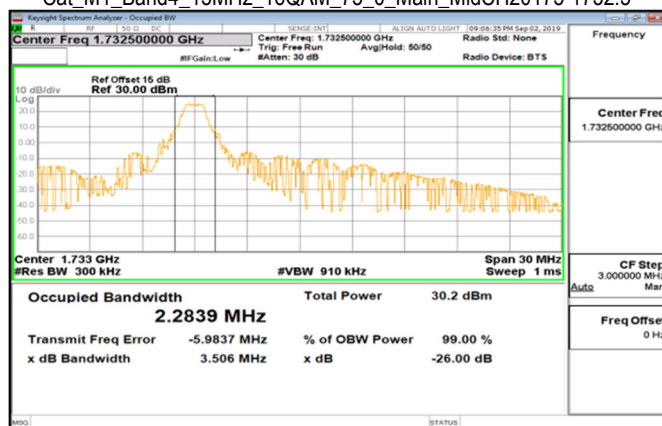
Cat_M1_Band4_15MHz_16QAM_75_0_Main_MidCH20175-1732.5
