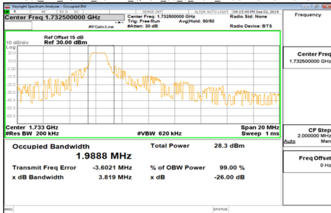
Cat_M1_Band4_10MHz_QPSK_50_0_Main_MidCH20175-1732.5
