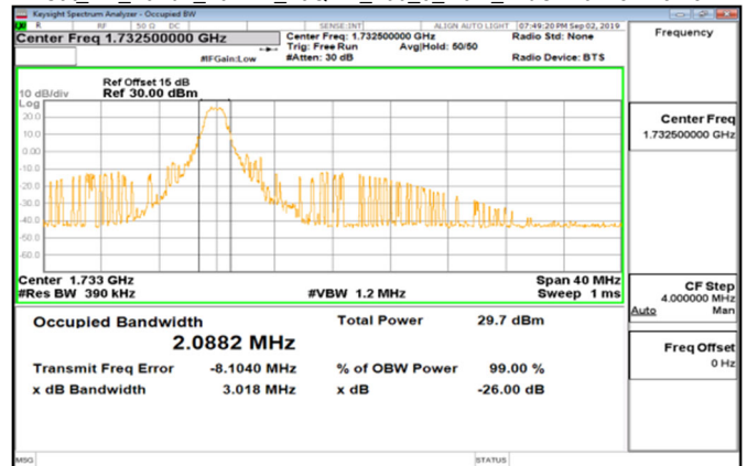
Cat M1_Band4_20MHz_16QAM_100_0_Main_MidCH20175-1732.5
