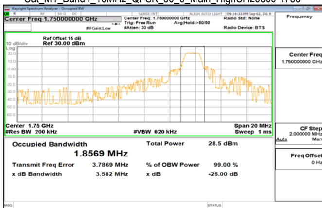
Cat_M1_Band4_10MHz_QPSK_50_0_Main_HighCH20350-1750
