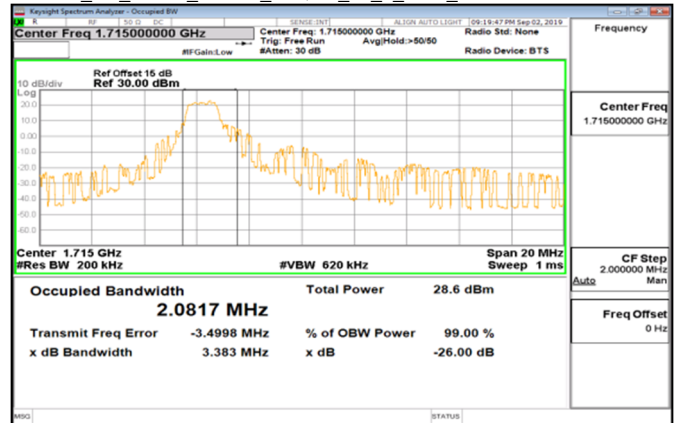
Cat_M1_Band4_10MHz_16QAM_50_0_Main_LowCH20000-1715
