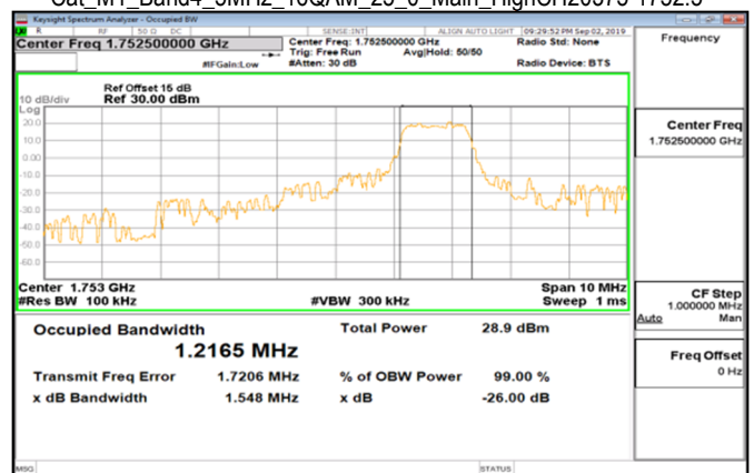
Cat_M1_Band4_5MHz_16QAM_25_0_Main_HighCH20375-1752.5
