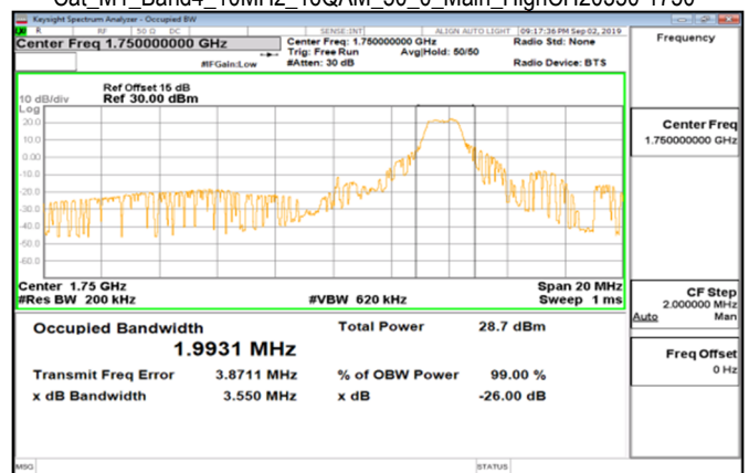
Cat_M1_Band4_10MHz_16QAM_50_0_Main_HighCH20350-1750
