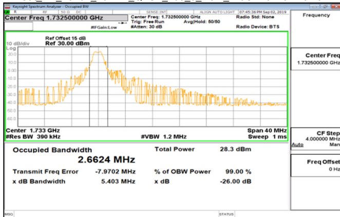
Cat M1_Band4_20MHz_QPSK_100_0_Main_MidCH20175-1732.5
