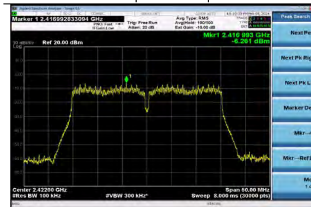
802.11n40 | Channel 3 | MCS7
