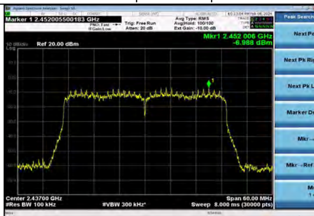
802.11ax40 | Channel 6 | MCS9
