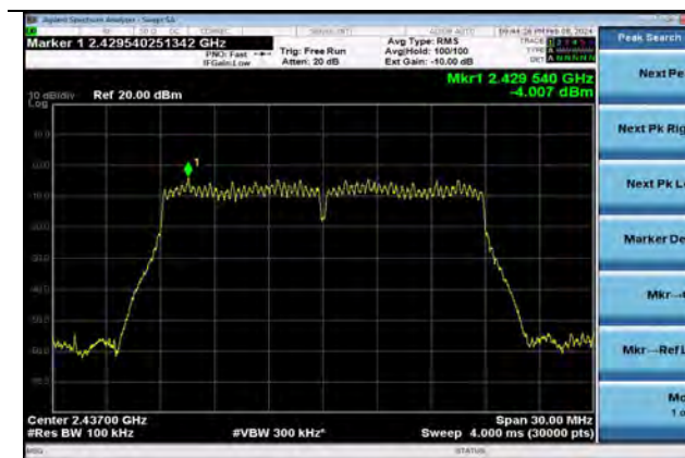
802.11n20 | Channel 6 | MCS7
