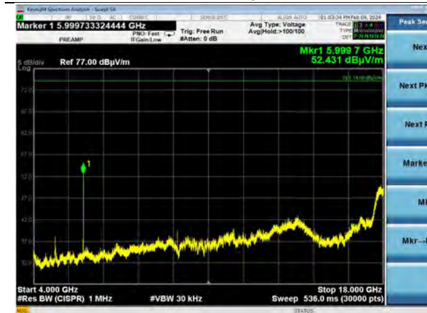
802.11ax20 | Channel 6 | MCS0 4000-18000 MHz | Vertical
