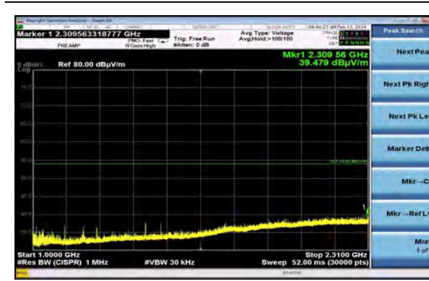
802.11ax40 | Channel 3 | MCS0 | RU38 1000-2310 MHz | Vertical
