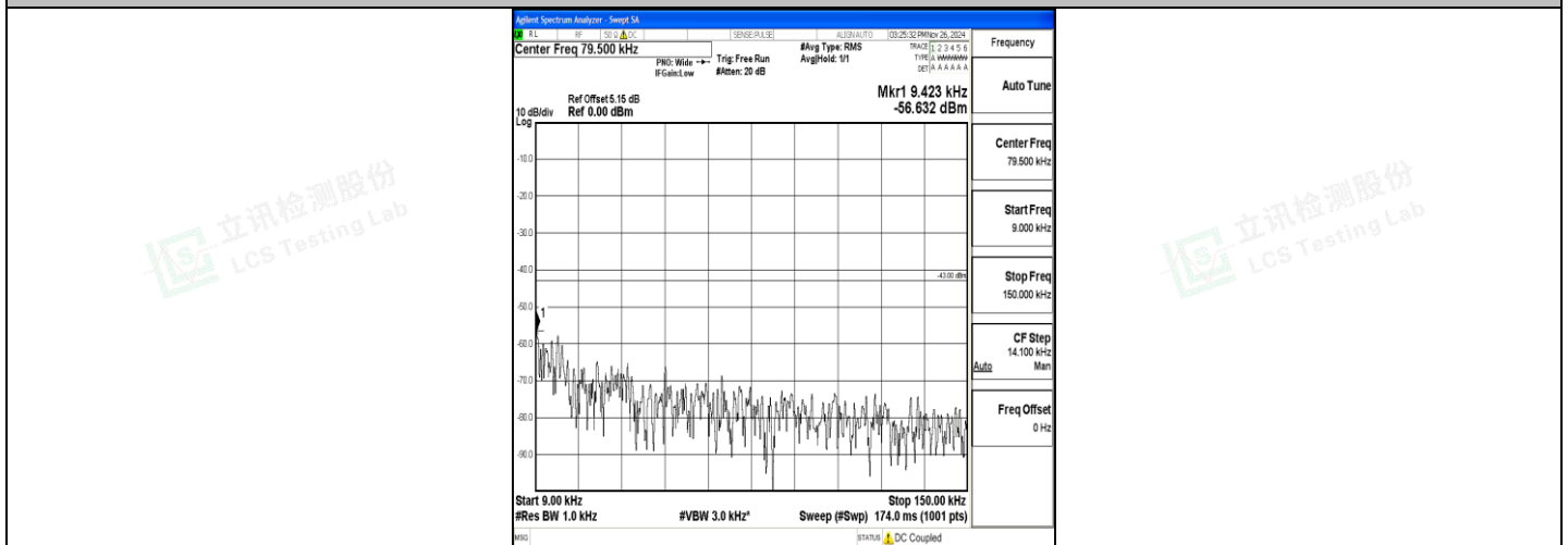
Band4_10MHz_16QAM_20175_1RB#0_0.009~0.15_0.009~0.15
