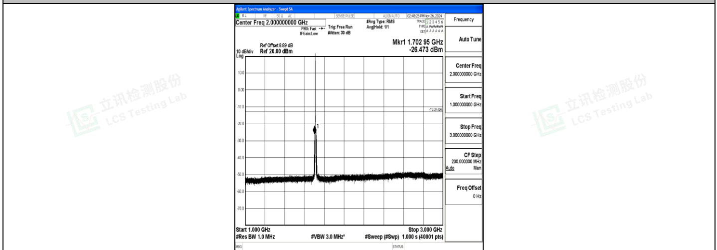
Band4_3MHz_QPSK_19965_1RB#0_1000~3000_1000~3000
