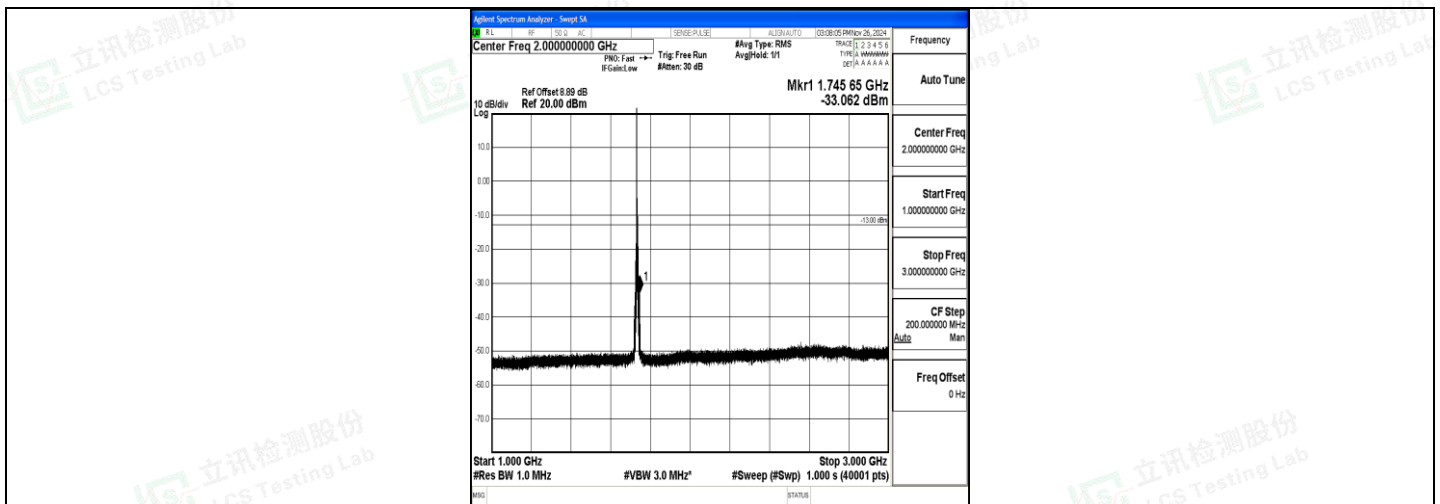
Band4_5MHz_QPSK_20175_1RB#0_1000~3000_1000~3000
