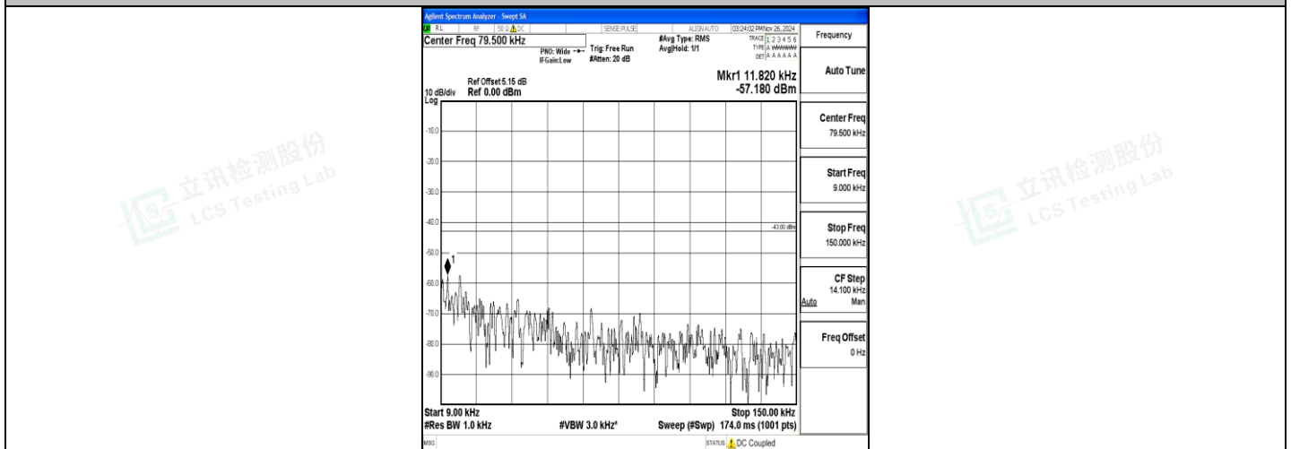
Band4_10MHz_QPSK_20000_1RB#0_0.009~0.15_0.009~0.15
