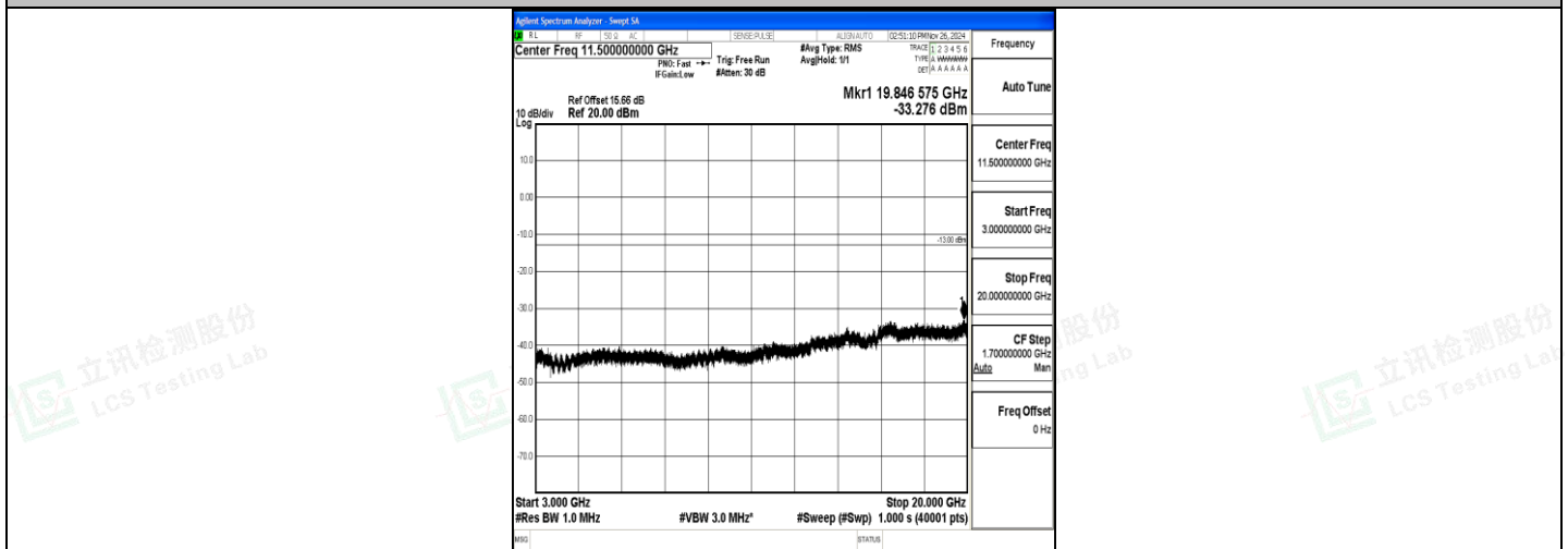
Band4_3MHz_16QAM_20385_1RB#0_3000~20000_3000~20000
