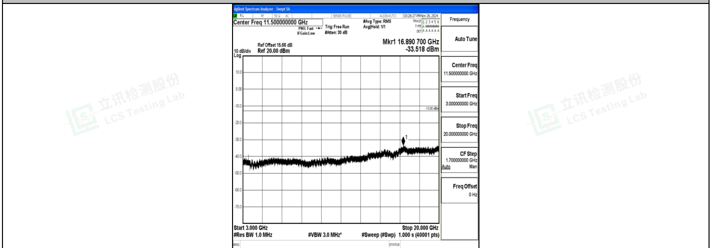
Band4_10MHz_QPSK_20350_1RB#0_3000~20000_3000~20000
