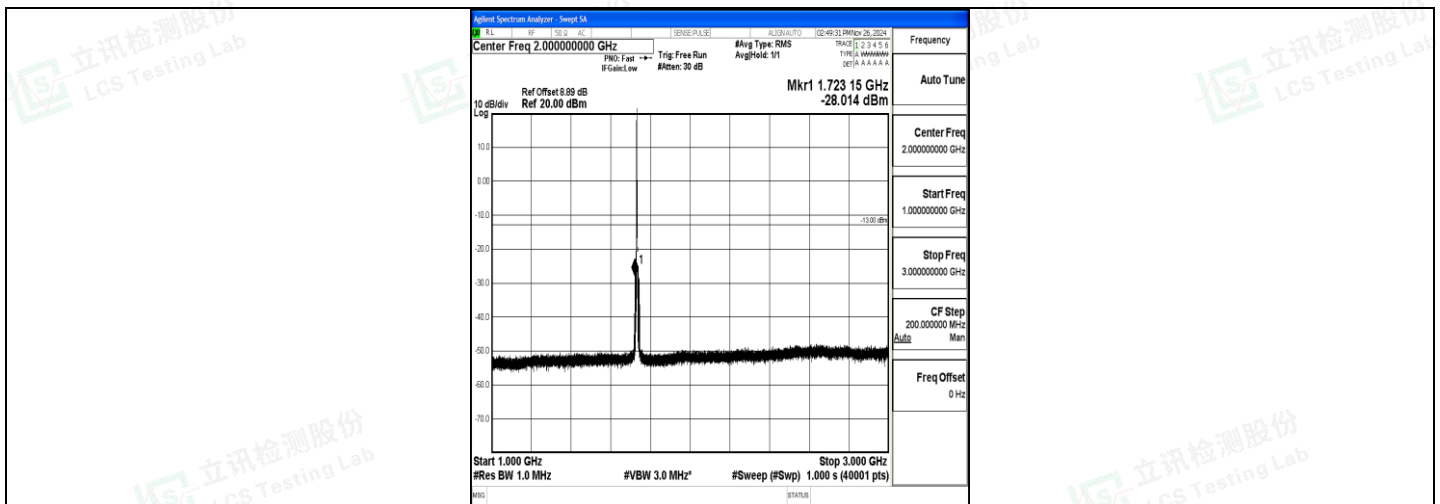
Band4_3MHz_QPSK_20175_1RB#0_1000~3000_1000~3000
