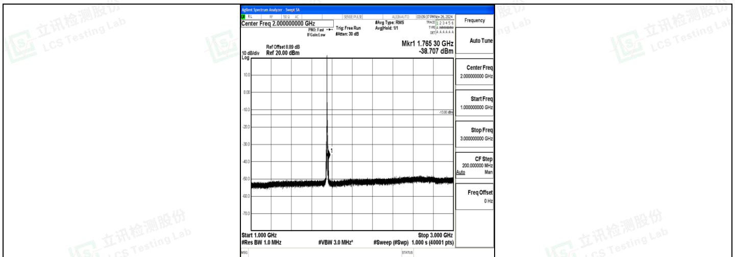
Band4_5MHz_16QAM_20375_1RB#0_1000~3000_1000~3000
