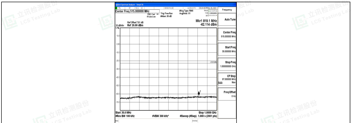
Band4_10MHz_16QAM_20000_1RB#0_30~1000_30~1000
