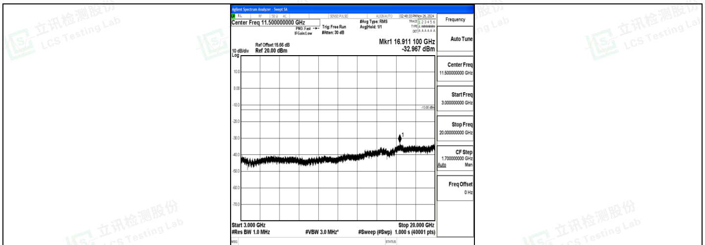
Band4_3MHz_QPSK_19965_1RB#0_3000~20000_3000~20000
