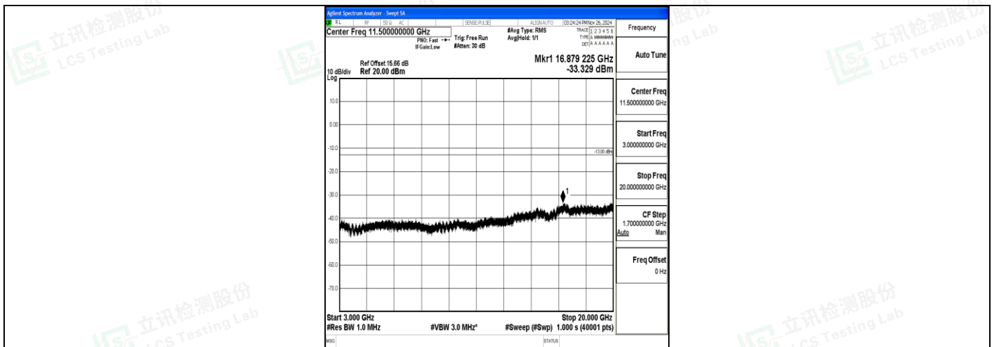
Band4_10MHz_QPSK_20000_1RB#0_3000~20000_3000~20000
