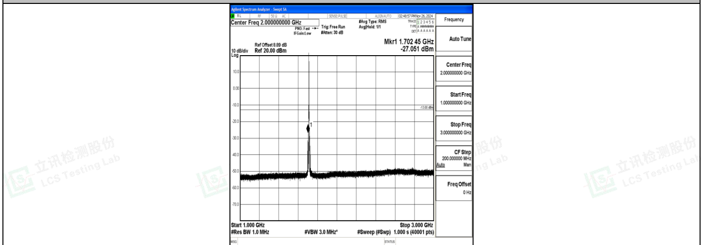
Band4_3MHz_16QAM_19965_1RB#0_1000~3000_1000~3000
