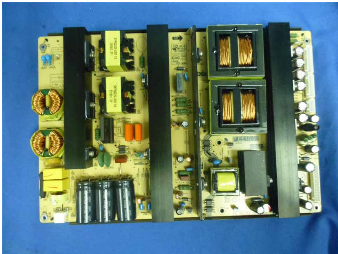
Figure 22 Frontside of the Power Board
