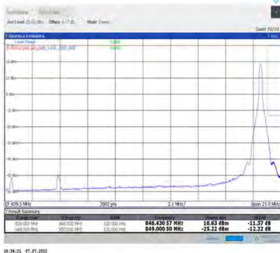
1-N26-824-849--15-20-H-5-CP-QPSK-Edge_1RB_Right-1@105-Ant1-seegraph-PASS-see graph
