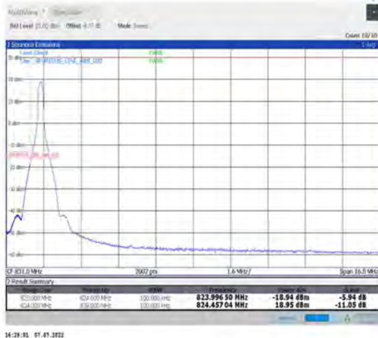
1-N26-824-849--15-15-L-4-CP-QPSK-Edge_1RB_Left-1@0-Ant1-seegraph-PASS-see graph
