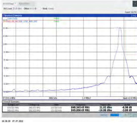
1-N26-824-849--15-10-H-2-DFT-PI2BPSK-Edge_1RB_Right-1@51-Ant1-seegraph-PASS-see graph
