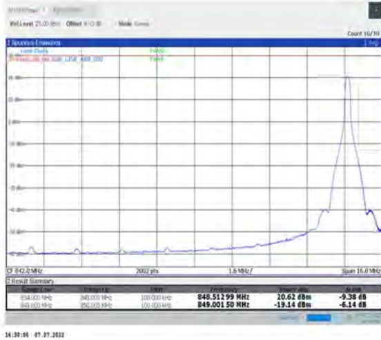
1-N26-824-849--15-15-H-2-DFT-PI2BPSK-Edge_1RB_Right-1@78-Ant1-seegraph-PASS-see graph
