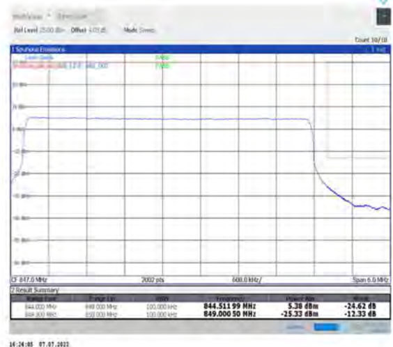
1-N26-824-849--15-5-H-6-CP-QPSK-Outer_Full-25@0-Ant1-seegraph-PASS-see graph
