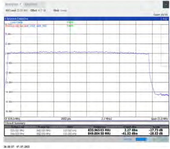
1-N26-824-849--15-20-H-3-DFT-PI2BPSK-Outer_Full-100@0-Ant1-seegraph-PASS-see graph
