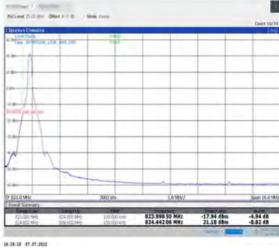
1-N26-824-849--15-15-L-1-DFT-PI2BPSK-Edge_1RB_Left-1@0-Ant1-seegraph-PASS-see graph
