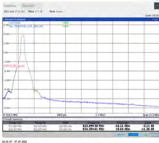
1-N26-824-849--15-10-L-4-CP-QPSK-Edge_1RB_Left-1@0-Ant1-seegraph-PASS-see graph
