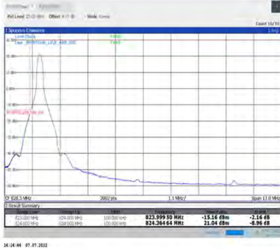
1-N26-824-849--15-10-L-1-DFT-PI2BPSK-Edge_1RB_Left-1@0-Ant1-seegraph-PASS-see graph
