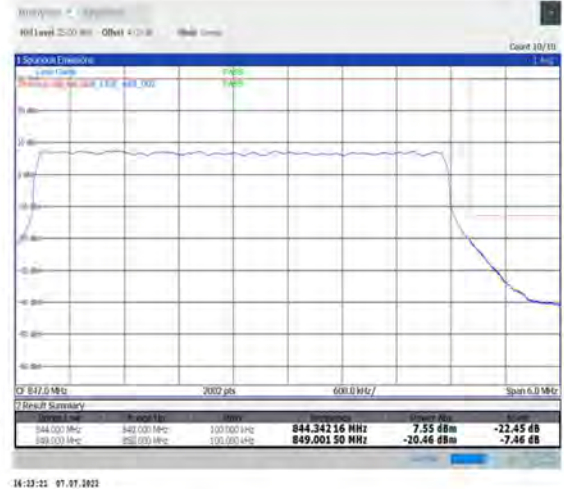
1-N26-824-849--15-5-H-3-DFT-PI2BPSK-Outer_Full-25@0-Ant1-seegraph-PASS-see graph
