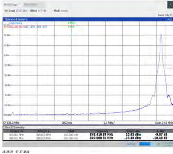
1-N26-824-849--15-20-H-2-DFT-PI2BPSK-Edge_1RB_Right-1@105-Ant1-seegraph-PASS-see graph
