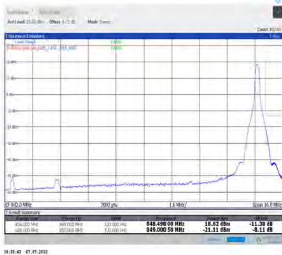
1-N26-824-849--15-15-H-5-CP-QPSK-Edge_1RB_Right-1@78-Ant1-seegraph-PASS-see graph
