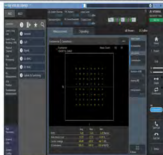
1-N26-824-849--15-20-M-8-CP-64QAM-Outer_Full-106@0-Ant1-see graph-PASS
