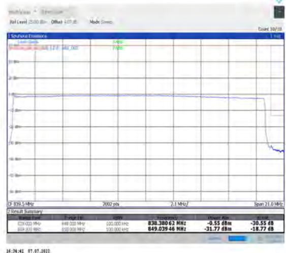
1-N26-824-849--15-20-H-6-CP-QPSK-Outer_Full-106@0-Ant1-seegraph-PASS-see graph
