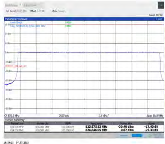
1-N26-824-849--15-15-L-6-CP-QPSK-Outer_Full-79@0-Ant1-seegraph-PASS-see graph
