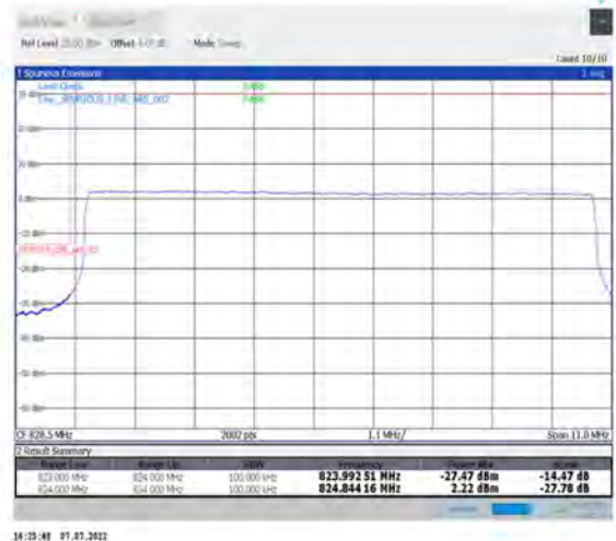
1-N26-824-849--15-10-L-6-CP-QPSK-Outer_Full-52@0-Ant1-seegraph-PASS-see graph
