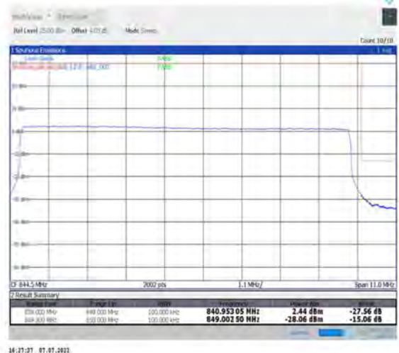
1-N26-824-849--15-10-H-6-CP-QPSK-Outer_Full-52@0-Ant1-seegraph-PASS-see graph
