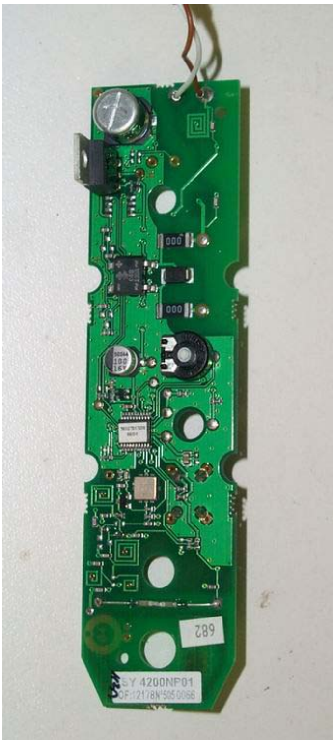
Component Side
