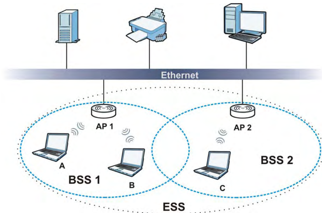
Figure 91 Infrastructure WLAN
