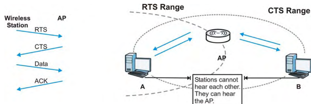
Figure 92 RTS/CTS
