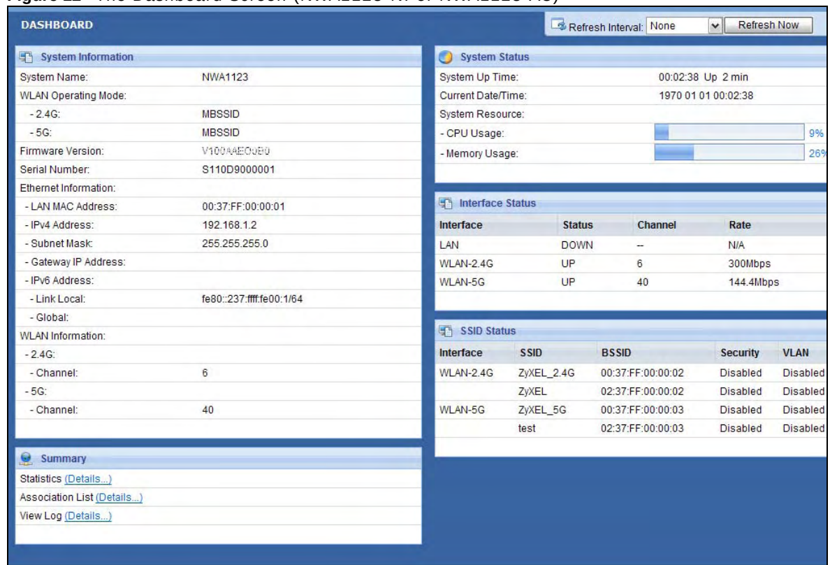
Figure 12 The Dashboard Screen (NWA1123-NI or NWA1123-AC)
