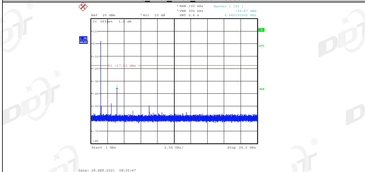
2DH5_Ant1_2402_0~Reference
