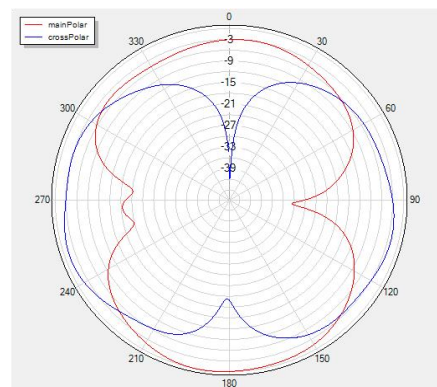
Theta=90 freq=5450MHz
