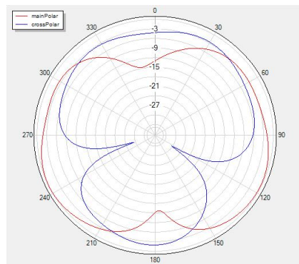
Theta=90 freq=2480MHz
