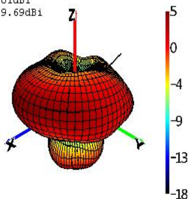
Phi=90 freq=5900MHz
