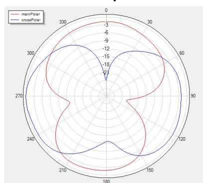
Theta=90 freq=5900MHz
