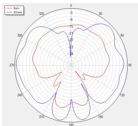
Phi=0 freq=7150MHz
