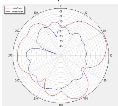
Phi=0 freq=5900MHz
