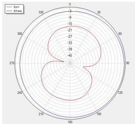
Theta=90 freq=7150MHz
