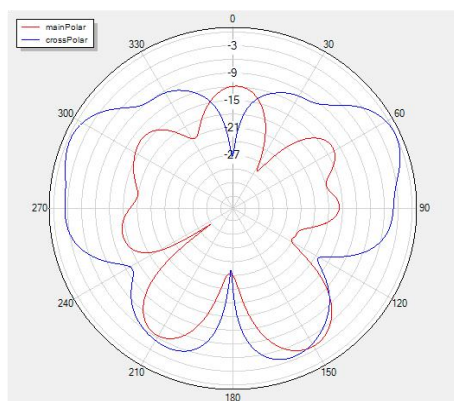
Phi=90 freq=5100MHz
