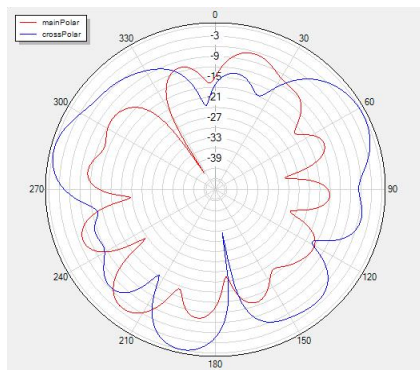
Phi=0 freq=2480MHz
