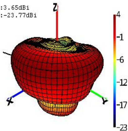
Phi=90 freq=5100MHz
