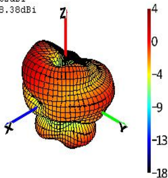
Phi=90 freq=2400MHz
