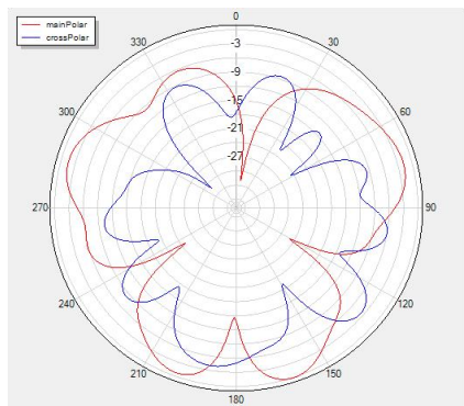
Phi=90 freq=2480MHz
