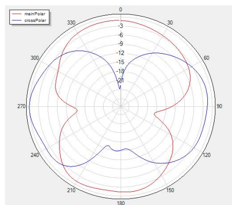
Theta=90 freq=5100MHz
