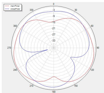
Theta=90 freq=2440MHz
