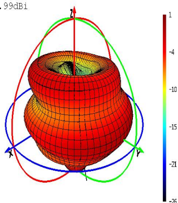
Phi=90 freq=7150MHz
