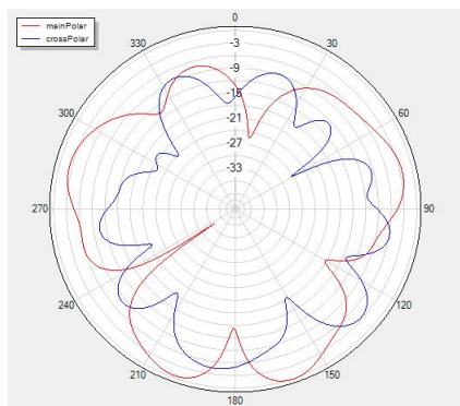
Phi=90 freq=2440MHz
