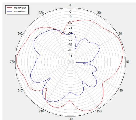
Phi=0 freq=5450MHz
