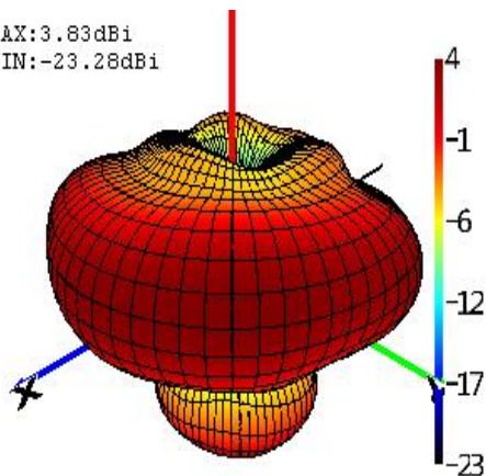
Phi=90 freq=5450MHz
