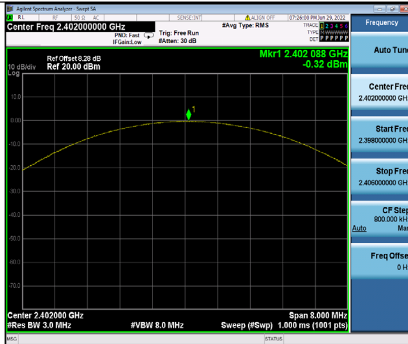
3DH5_Ant1_2402
