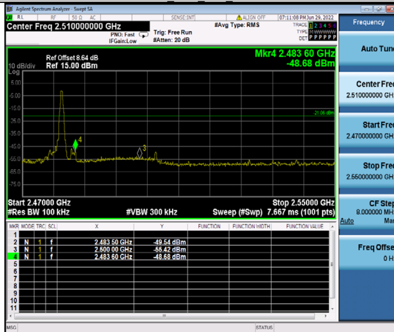
DH5_Ant1_High_2480
