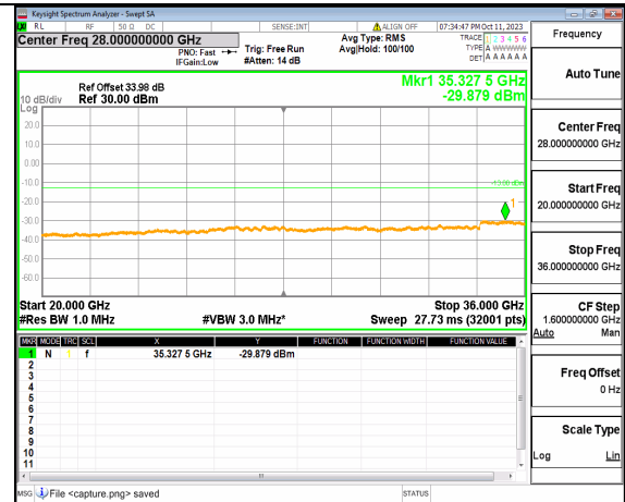
5A_n77(3450-3550MHz) (20GHz-36GHz) 30M DFT-s-OFDM QPSK Edge_1RB_Left Mid
