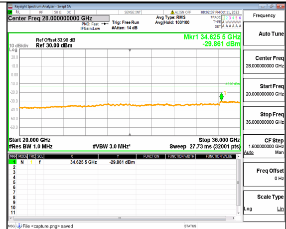
5A_n77(3450-3550MHz) (20GHz-36GHz) 40M DFT-s-OFDM BPSK Edge_1RB_Left High
