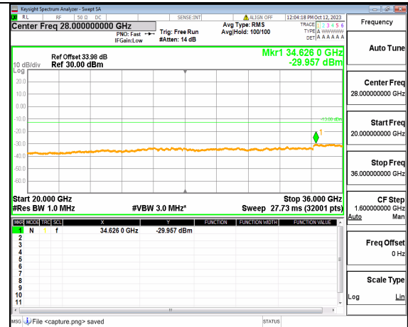
5A_n77(3450-3550MHz) (20GHz-36GHz) 60M DFT-s-OFDM QPSK Edge_1RB_Left High
