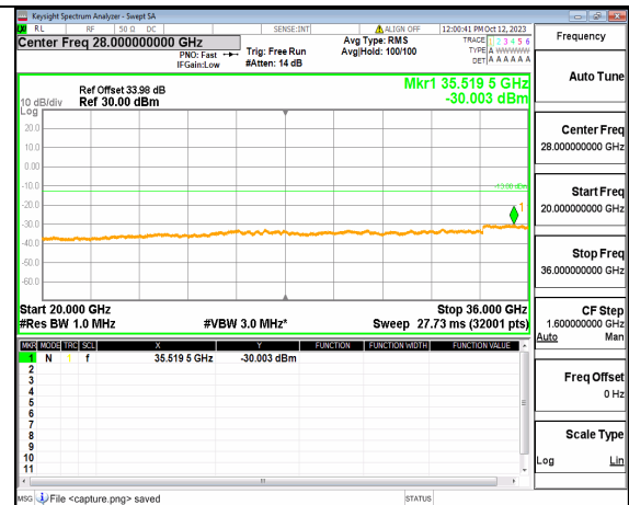
5A_n77(3450-3550MHz) (20GHz-36GHz) 60M DFT-s-OFDM BPSK Edge_1RB_Left High
