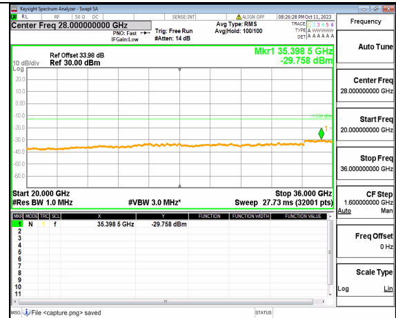
5A_n77(3450-3550MHz) (20GHz-36GHz) 50M DFT-s-OFDM BPSK Edge_1RB_Left High
