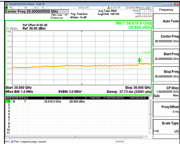
5A_n77(3450-3550MHz) (20GHz-36GHz) 30M DFT-s-OFDM BPSK Edge_1RB_Left Mid
