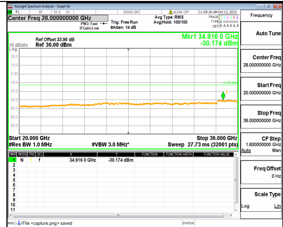
5A_n77(3450-3550MHz) (20GHz-36GHz) 60M DFT-s-OFDM BPSK Outer_Full High
