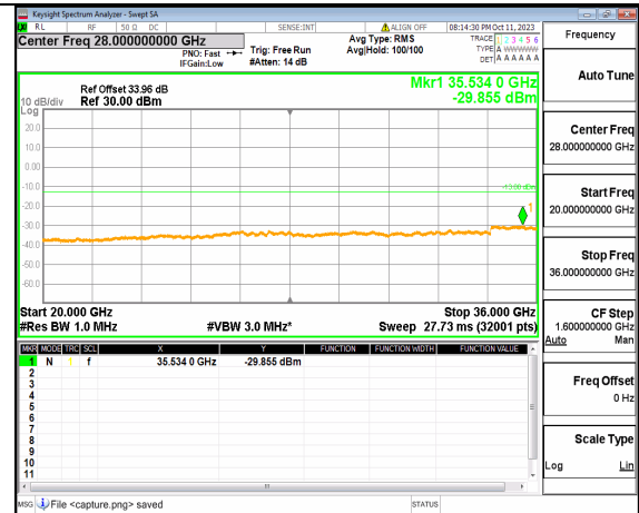
5A_n77(3450-3550MHz) (20GHz-36GHz) 50M DFT-s-OFDM QPSK Edge_1RB_Left Low
