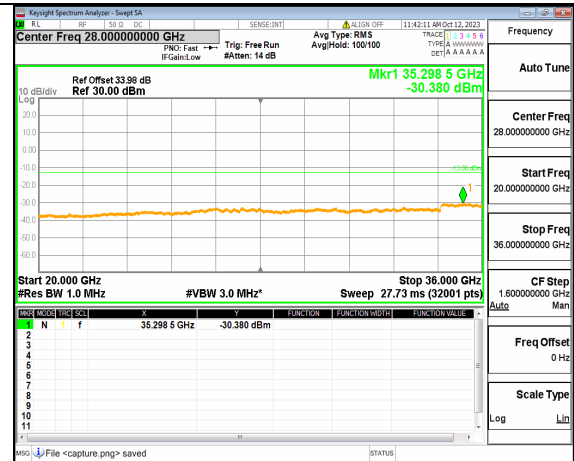
5A_n77(3450-3550MHz) (20GHz-36GHz) 50M DFT-s-OFDM QPSK Edge_1RB_Left High
