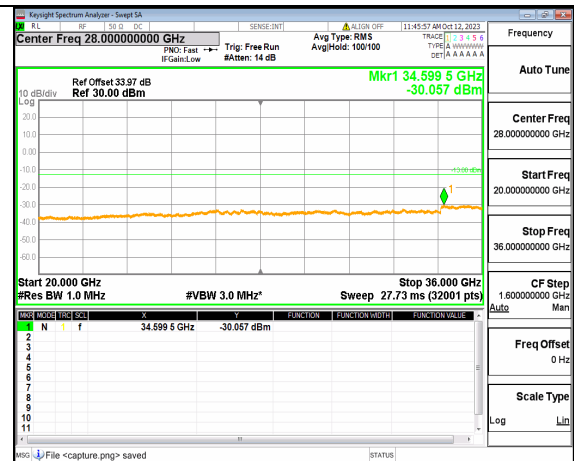
5A_n77(3450-3550MHz) (20GHz-36GHz) 60M DFT-s-OFDM BPSK Edge_1RB_Left Low
