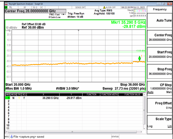
5A_n77(3450-3550MHz) (20GHz-36GHz) 50M DFT-s-OFDM QPSK Edge_1RB_Left Mid
