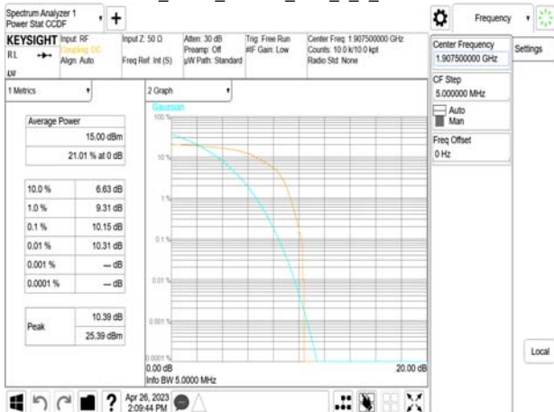
Band2_5MHz_16QAM_RB5_0_3_CH19175
