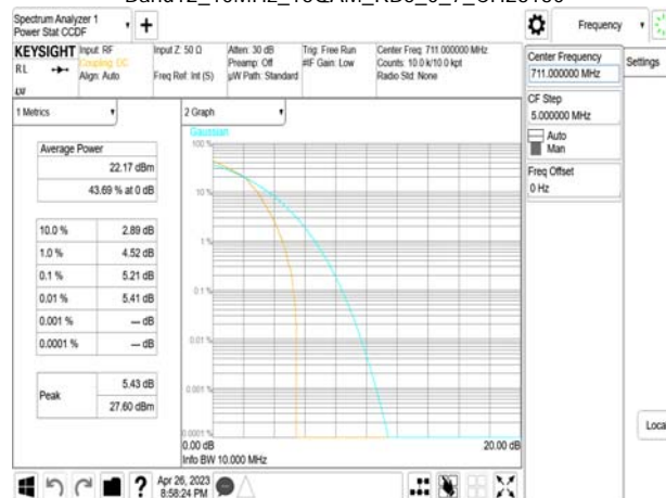
Band12_10MHz_16QAM_RB5_0_7_CH23130
