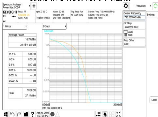
Band12_5MHz_16QAM_RB5_0_3_CH23155
