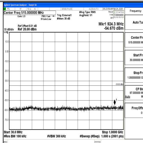
Band38_5MHz_16QAM_38000_1RB#0_30~1000_30~1000
