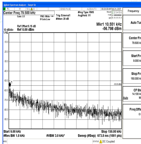
Band38_5MHz_16QAM_38000_1RB#0_0.009~0.15_0.009~0.15
