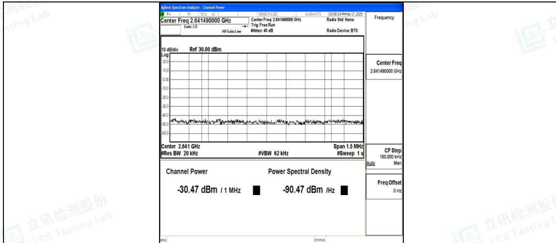
Band38_20MHz_QPSK_38150_100RB#0_Final1
