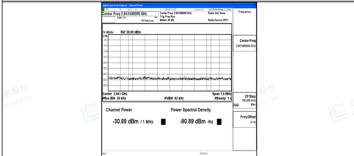
Band38_20MHz_16QAM_38150_100RB#0_Final1
