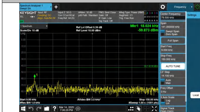
Band4-10MHz-QPSK-20175-1RB#0-0.009~0.15-PASS
