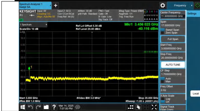
Band4-10MHz-QPSK-20175-1RB#0-3000~20000-PASS
