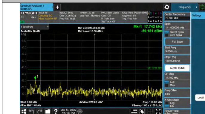
Band4-15MHz-QPSK-20325-1RB#0-0.009~0.15-PASS
