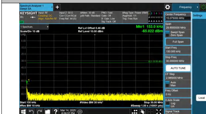
Band4-5MHz-QPSK-20375-1RB#24-0.15~30-PASS
