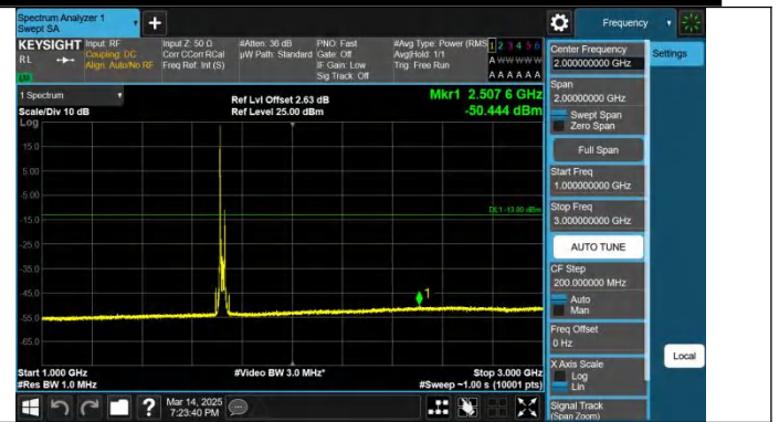
Band4-20MHz-QPSK-20050-1RB#0-1000~3000-PASS
