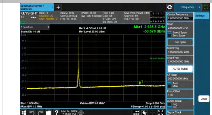
Band4-15MHz-QPSK-20325-1RB#0-1000~3000-PASS
