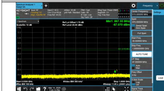
Band4-10MHz-QPSK-20000-1RB#0-30~1000-PASS
