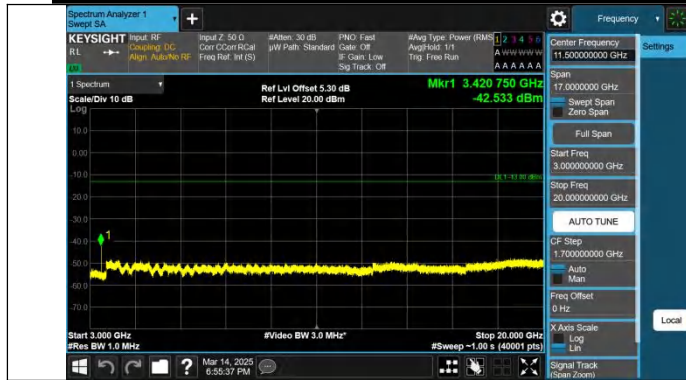
Band4-5MHz-QPSK-19975-1RB#0-3000~20000-PASS
