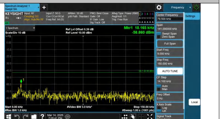
Band4-10MHz-QPSK-20000-1RB#49-0.009~0.15-PASS
