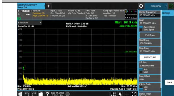
Band4-20MHz-QPSK-20175-1RB#99-0.15~30-PASS
