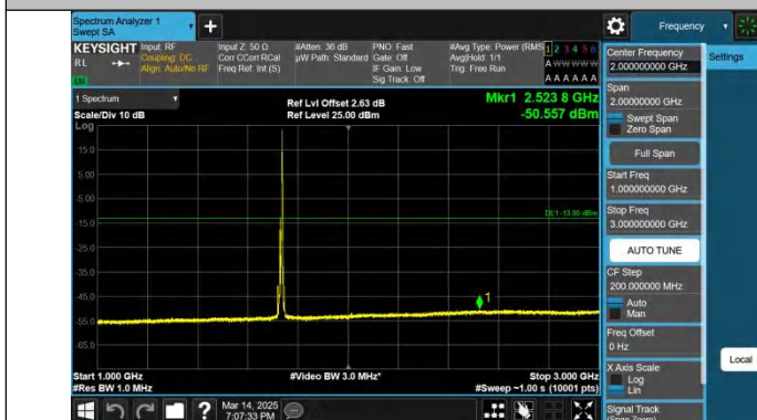
Band4-10MHz-QPSK-20175-1RB#49.1000~3000-PASS
