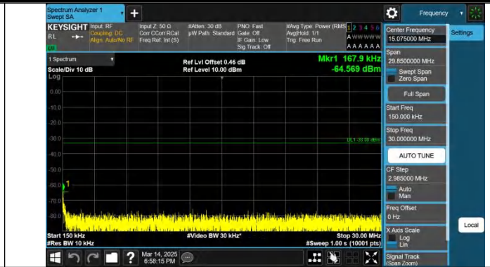
Band4-5MHz-QPSK-20375-1RB#0-0.15~30-PASS
