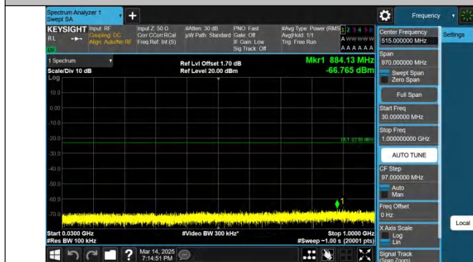
Band4-15MHz-QPSK-20025-1RB#0-30~1000-PASS
