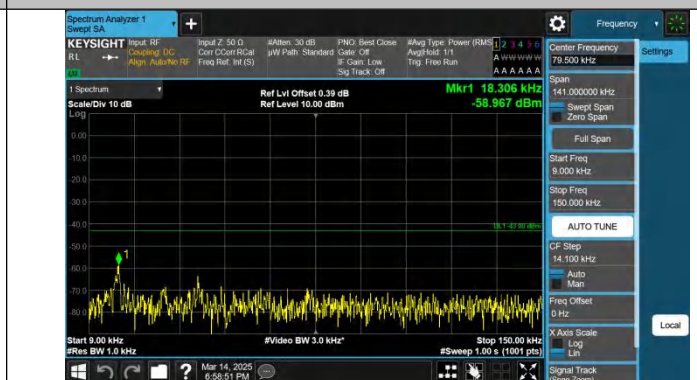
Band4-5MHz-QPSK-20375-1RB#24-0.009~0.15-PASS
