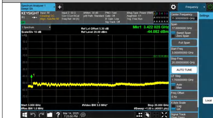
Band4-20MHz-QPSK-20050-1RB#0-3000~20000-PASS
