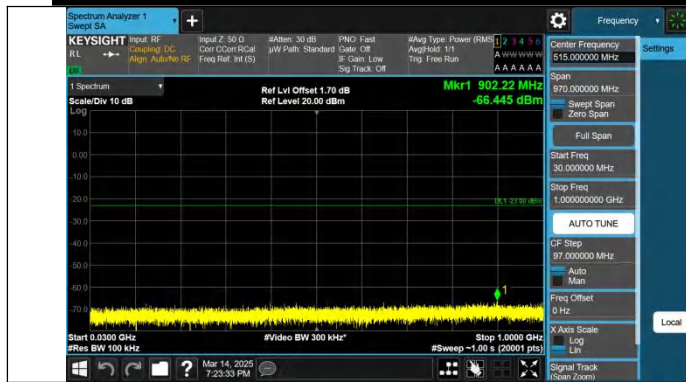
Band4-20MHz-QPSK-20050-1RB#0-30~1000-PASS
