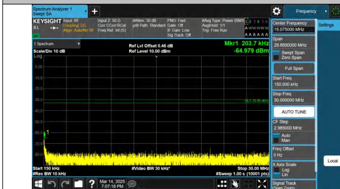
Band4-10MHz-QPSK-20175-1RB#49.0.15~30-PASS
