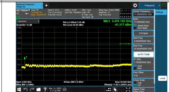
Band4-15MHz-QPSK-20175-1RB#74-3000~20000-PASS
