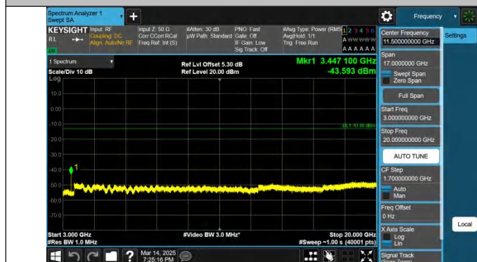
Band4-20MHz-QPSK-20175-1RB#0-3000~20000-PASS
