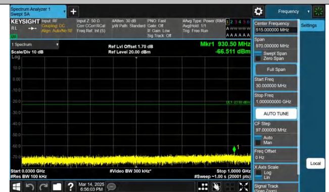
Band4-5MHz-QPSK-19975-1RB#24-30~1000-PASS
