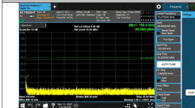
Band4-20MHz-QPSK-20050-1RB#99-0.15~30-PASS
