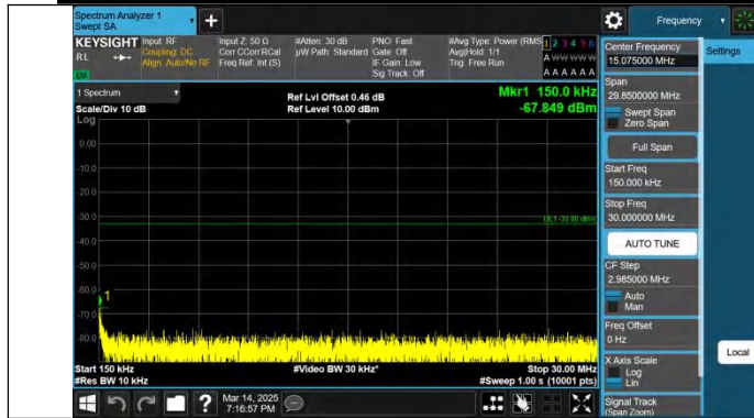
Band4-15MHz-QPSK-20175-1RB#74-0.15~30-PASS
