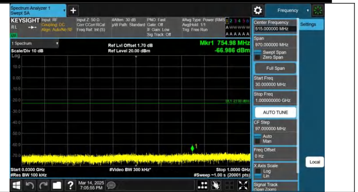
Band4-10MHz-QPSK-20000-1RB#49-30~1000-PASS
