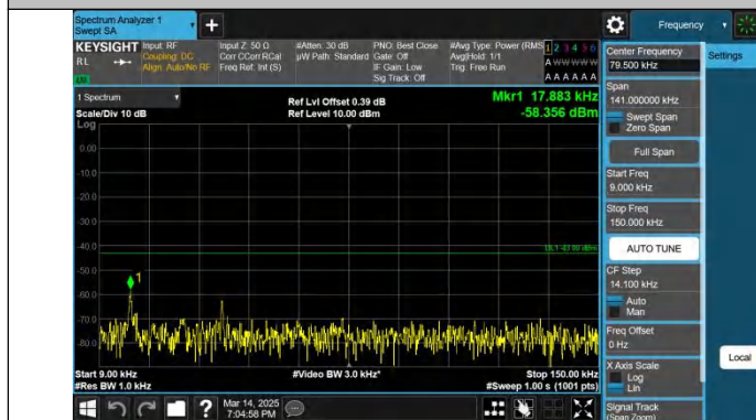
Band4-10MHz-QPSK-20000-1RB#0-0.009~0.15-PASS
