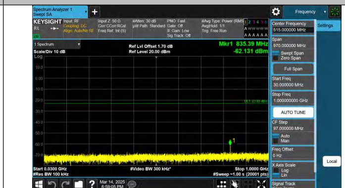
Band4-5MHz-QPSK-20375-1RB#24-30~1000-PASS
