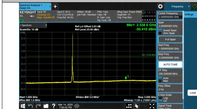
Band4-10MHz-QPSK-20000-1RB#49-1000~3000-PASS
