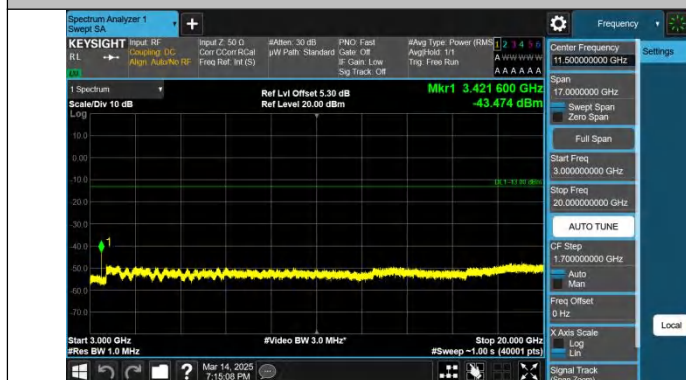
Band4-15MHz-QPSK-20025-1RB#0-3000~20000-PASS
