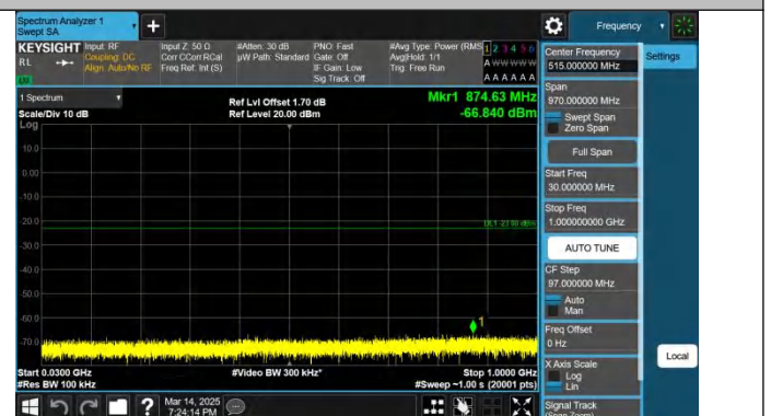
Band4-20MHz-QPSK-20050-1RB#99-30~1000-PASS
