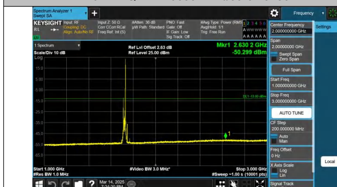
Band4-20MHz-QPSK-20050-1RB#99-1000~3000-PASS
