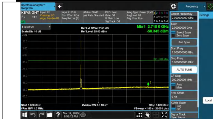
Band4-5MHz-QPSK-20375-1RB#24-1000~3000-PASS
