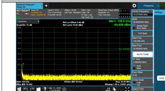
Band4-15MHz-QPSK-20025-1RB#74-0.15~30-PASS
