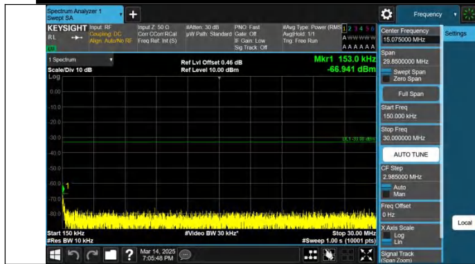
Band4-10MHz-QPSK-20000-1RB#49-0.15~30-PASS
