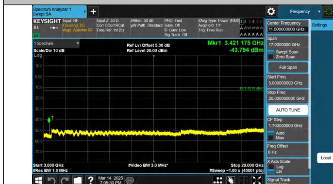
Band4-10MHz-QPSK-20000-1RB#0-3000~20000-PASS
