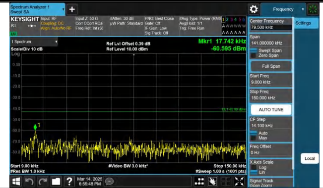
Band4-5MHz-QPSK-19975-1RB#24-0.009~0.15-PASS
