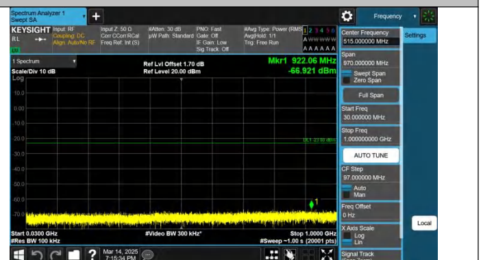
Band4-15MHz-QPSK-20025-1RB#74-30~1000-PASS
