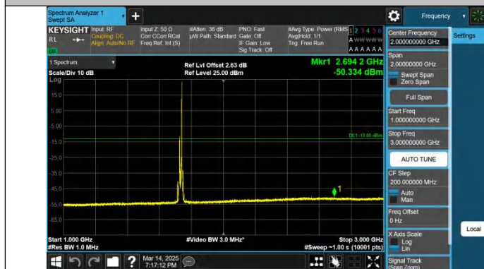
Band4-15MHz-QPSK-20175-1RB#74-1000~3000-PASS
