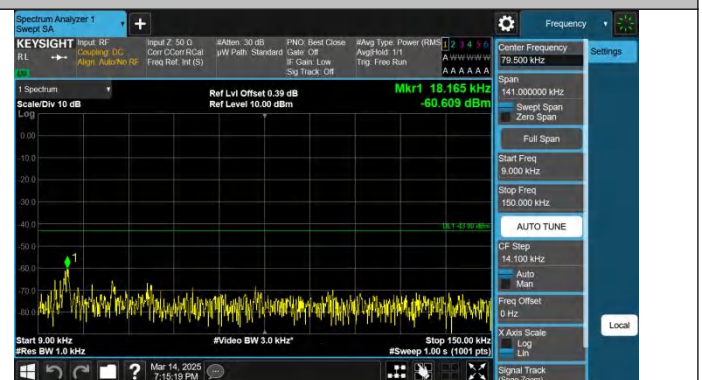
Band4-15MHz-QPSK-20025-1RB#74-0.009~0.15-PASS
