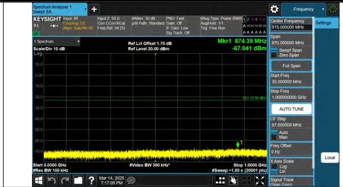
Band4-15MHz-QPSK-20175-1RB#74-30~1000-PASS
