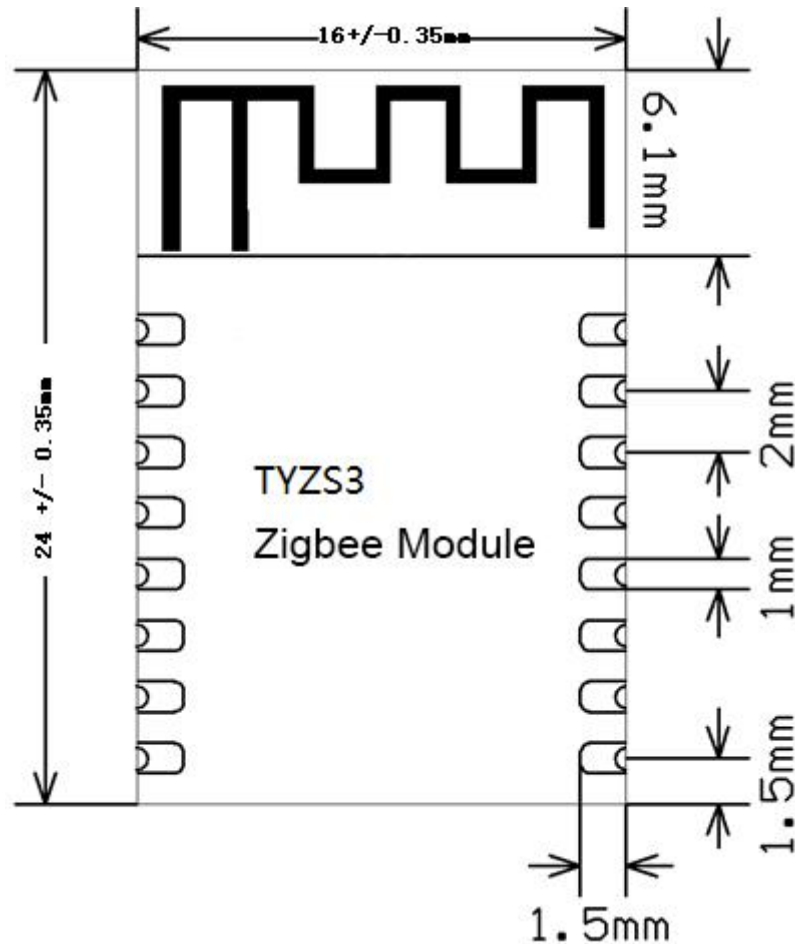
Figure 6-1 TYZS3 mechanical dimensions
