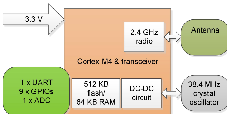
Figure 1-1 TYZS3 architecture
