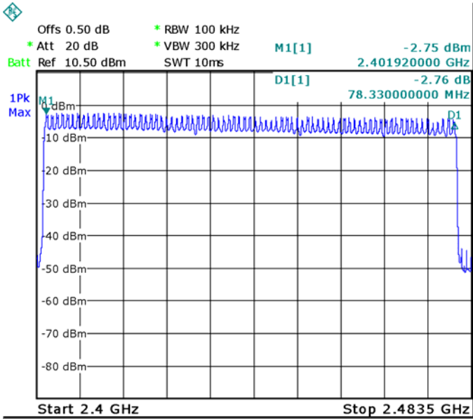
Modulation: 8DPSK
