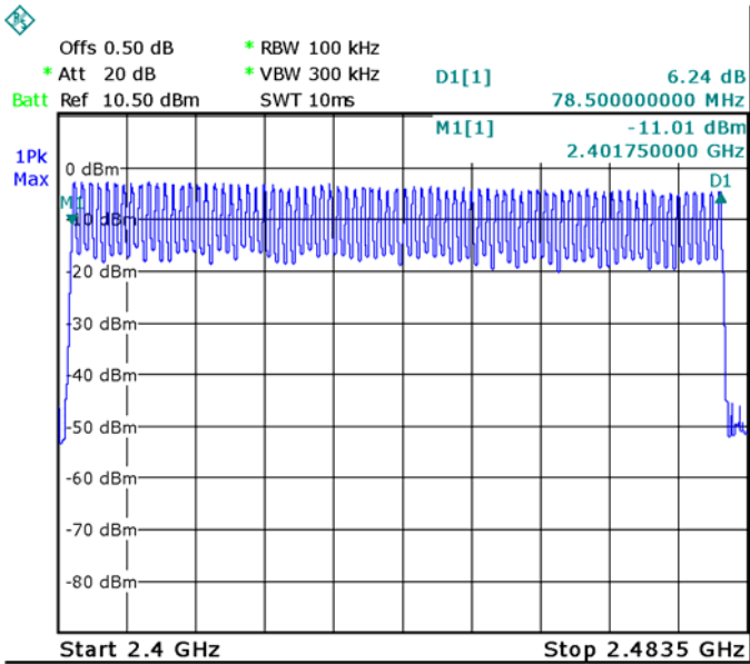
Modulation: GFSK
