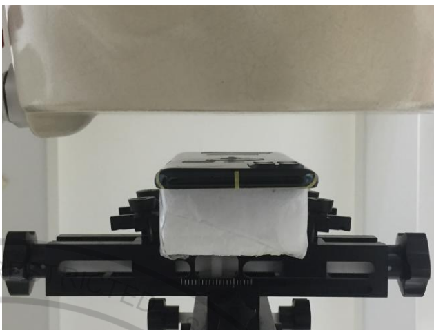
Back, Test Separation 28 mm
