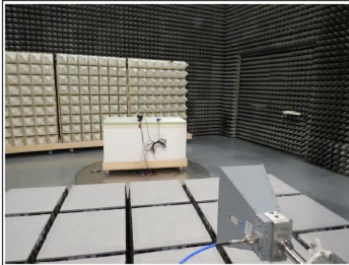
Test setup Helix antenna 1-17GHz
