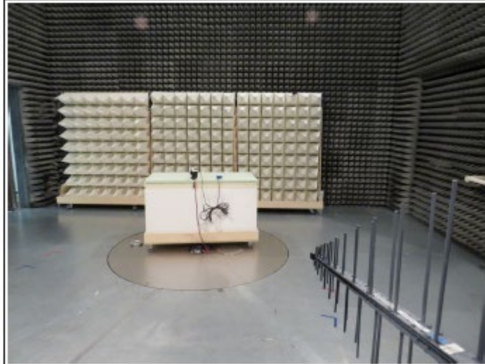
Test setup Helix antenna 200-1000MHz
