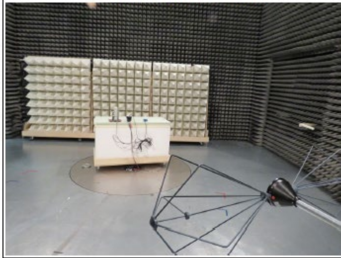
Test setup Wall antenna 30-200MHz
