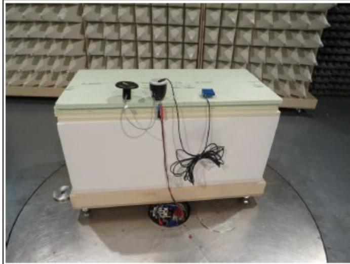
Test setup Pit antenna
