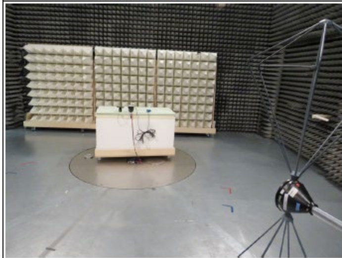
Test setup Pit antenna 30-200MHz
