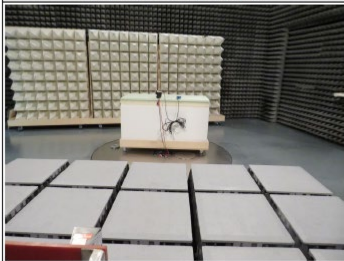
Test setup Helix antenna 17-19GHz
