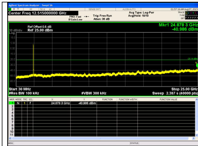
Spurious Emission IEEE 802.11ax_Channel 1_20MHz_Antenna 0_RU&Index 52RU37
