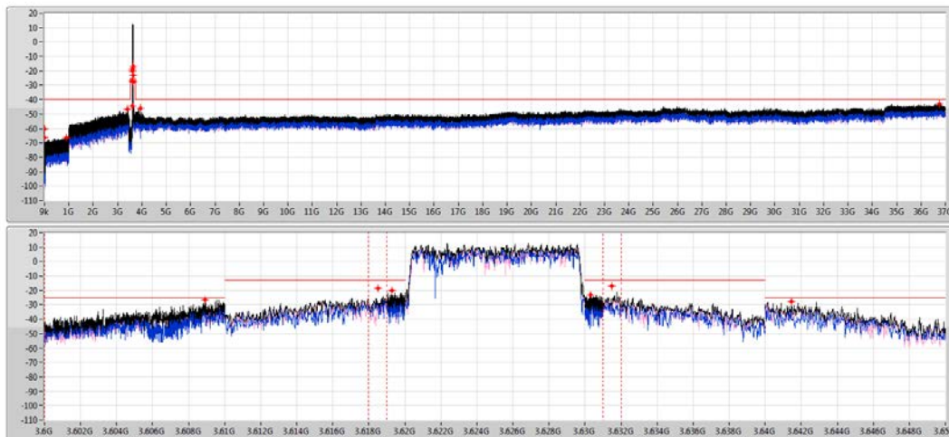
Band 48_10MHz_2TX 3625MHz_QPSK
