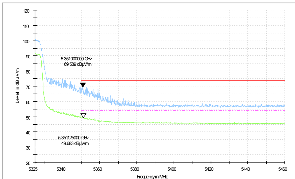
Fig. 18 Band Edges (802.11ac-HT40 Ch62, 5310MHz)
