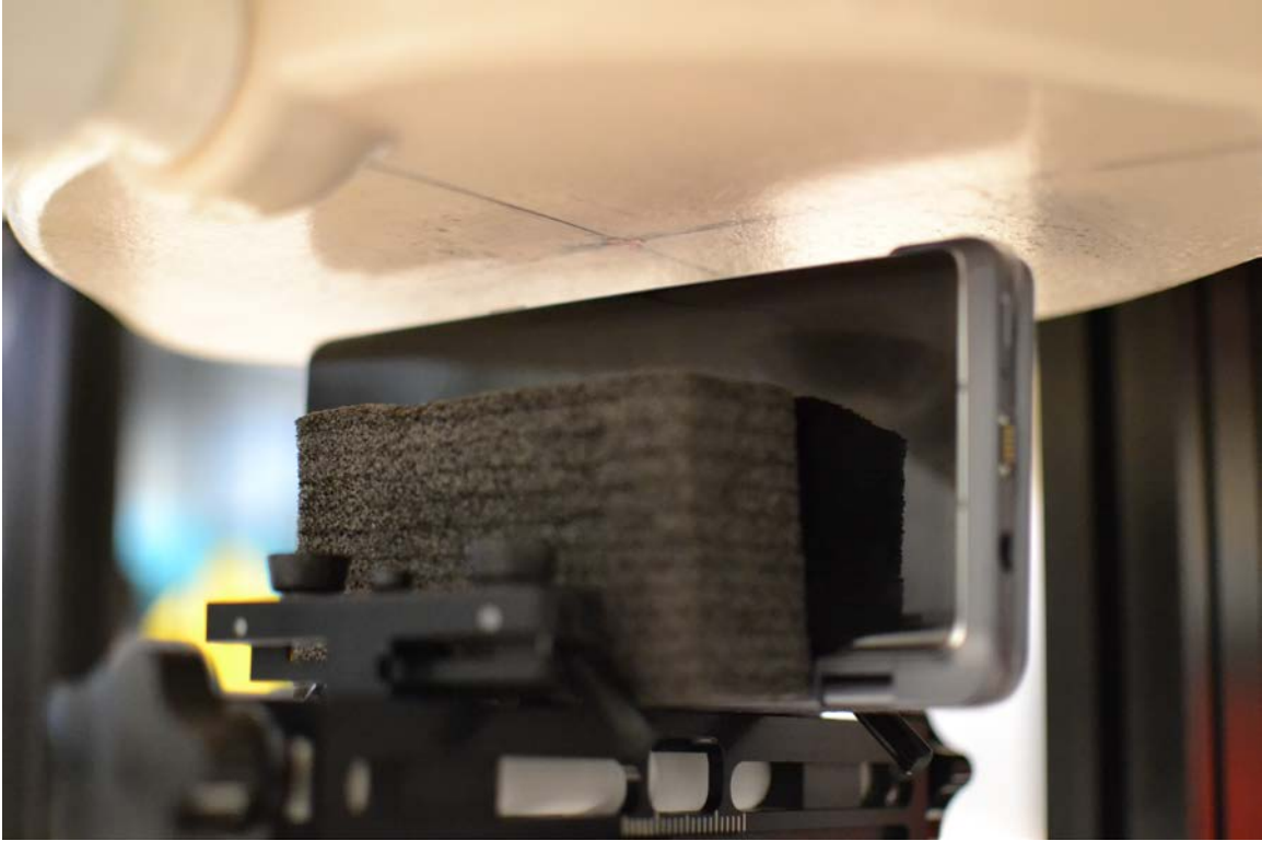
SAR Test Setup Photo 29 – Right Edge at 10 mm with Dual Display Accessory Position #3
