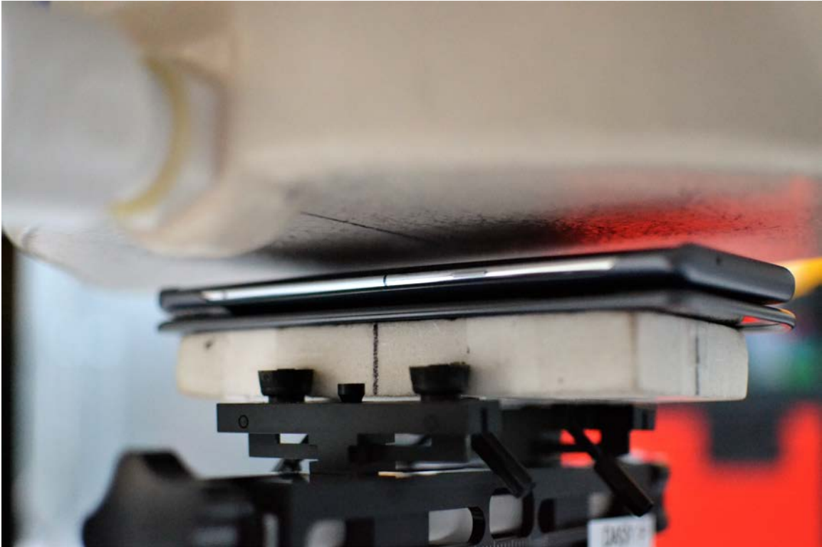
SAR Test Setup Photo 17 – Front Side with Dual Display Accessory Position #3 at 10 mm
