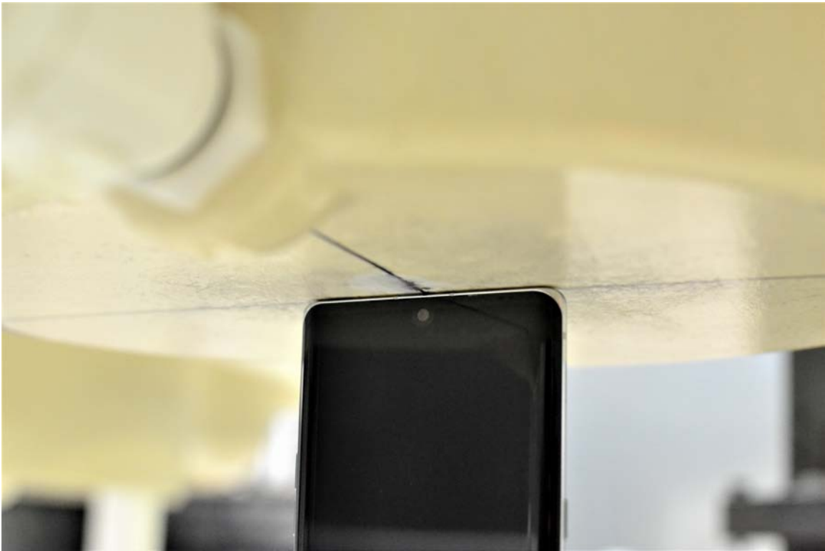
SAR Test Setup Photo 20 – Top Edge at 0 mm
