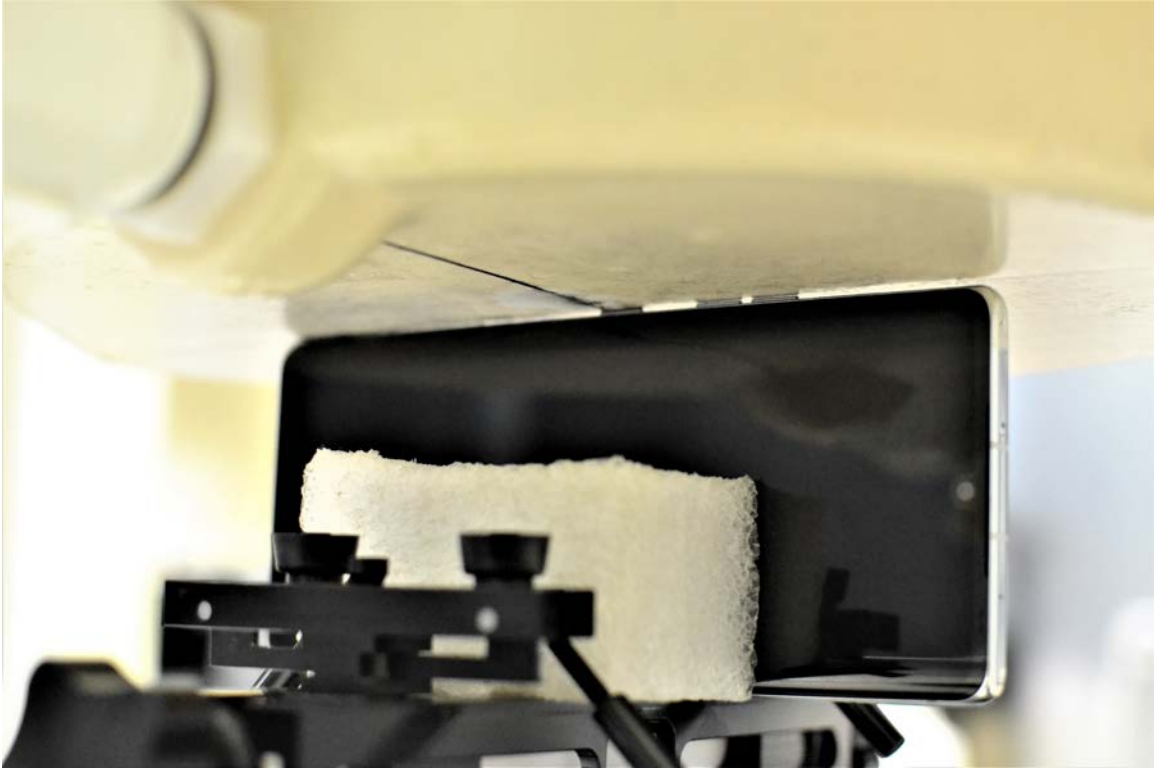
SAR Test Setup Photo 35 – Left Edge at 0 mm
