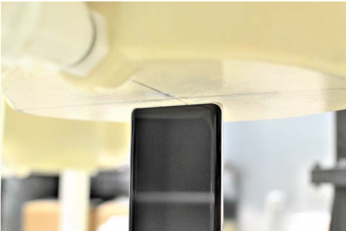
SAR Test Setup Photo 22 – Bottom Edge at 3 mm
