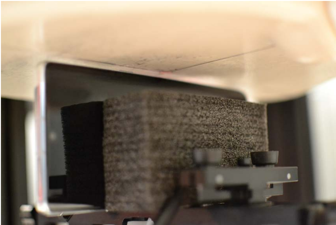
SAR Test Setup Photo 30 – Right Edge at 2 mm
