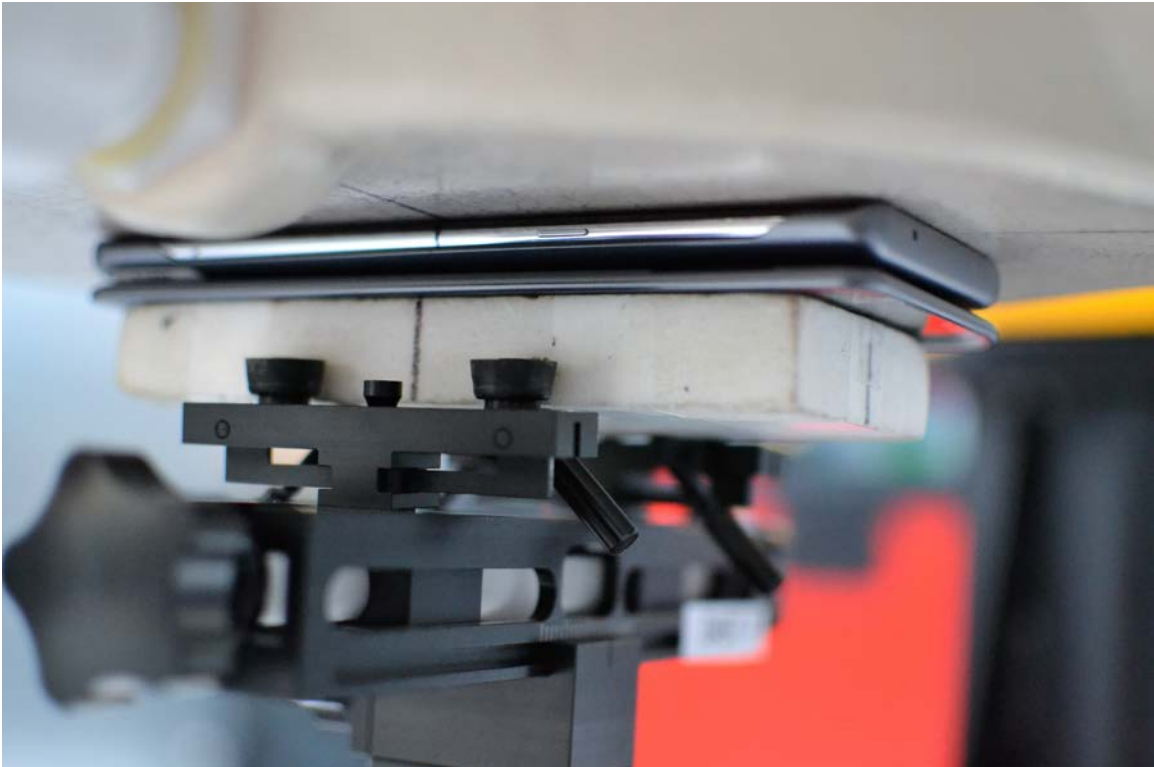
SAR Test Setup Photo 18 – Front Side with Dual Display Accessory Position #3 at 0 mm
