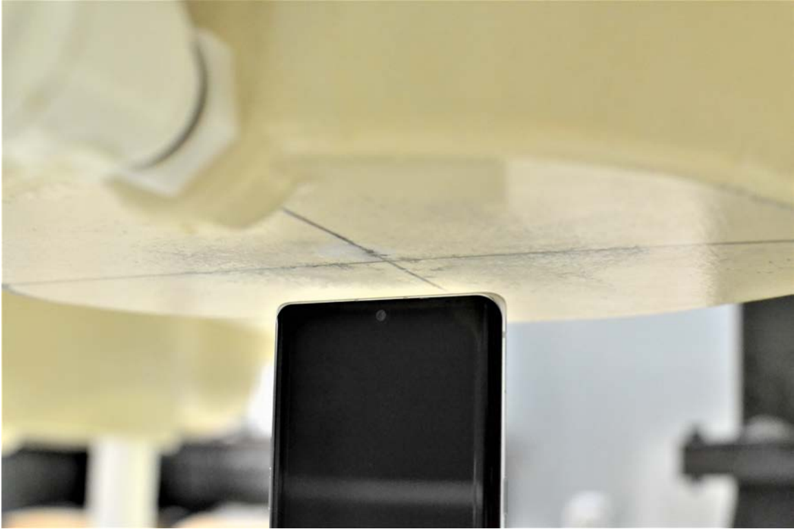
SAR Test Setup Photo 19 – Top Edge at 10 mm
