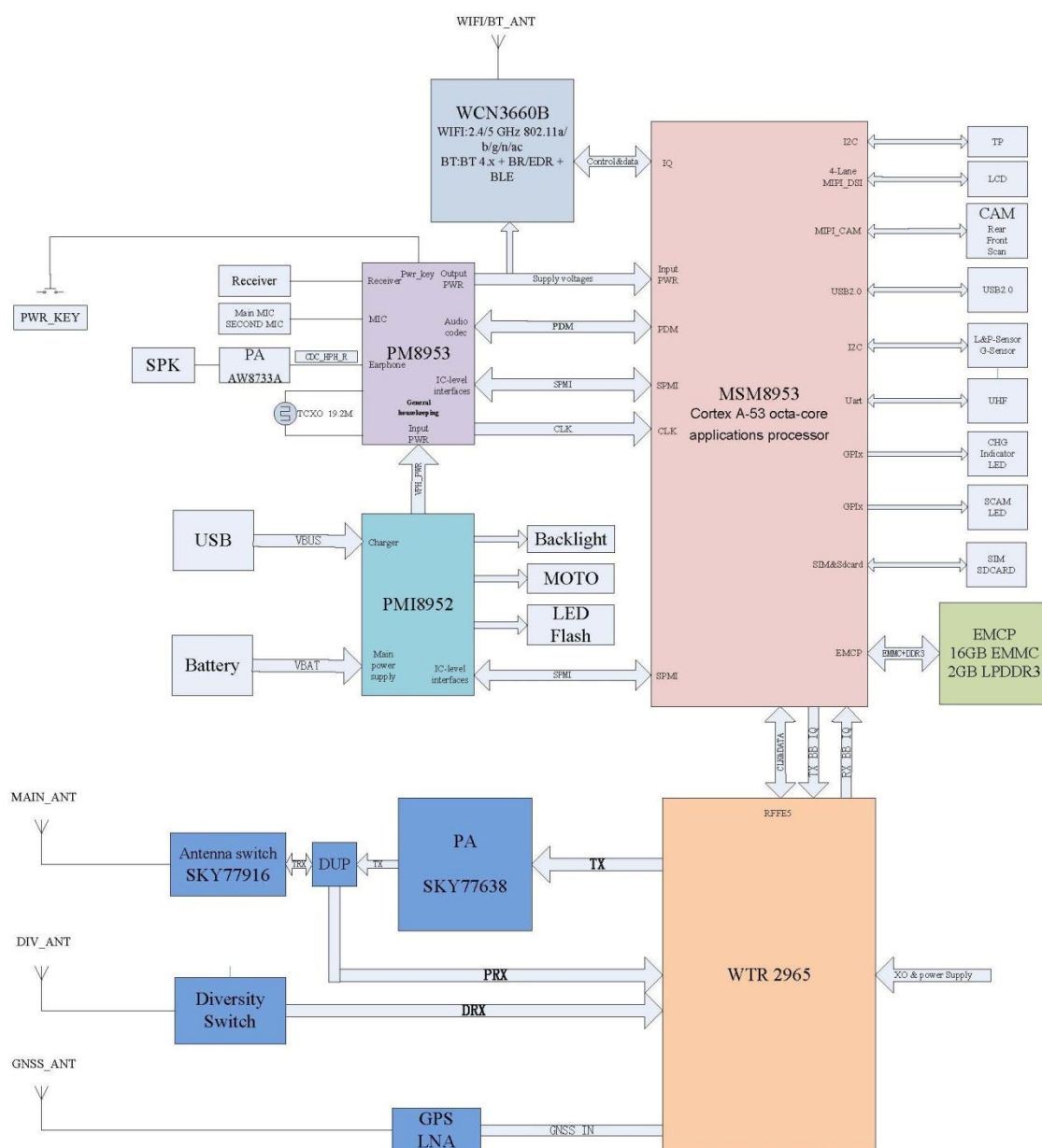
Figure 2.1: module function block diagram
