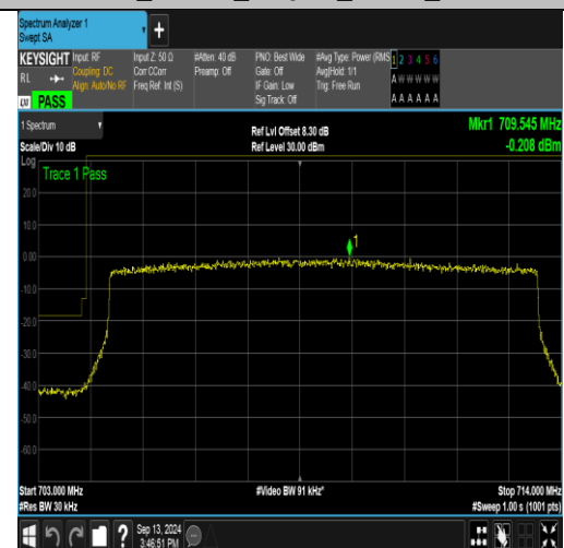
Band17_10MHz_16QAM_23780_50RB#0
