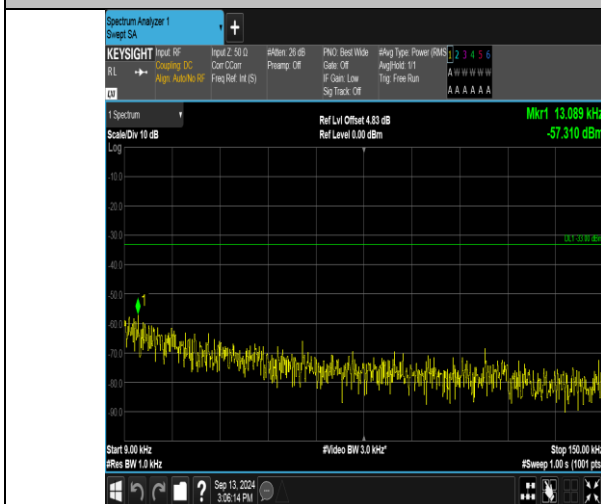
Band17_5MHz_QPSK_23755_1RB#24_0.009~0.15_0.009~0.15
