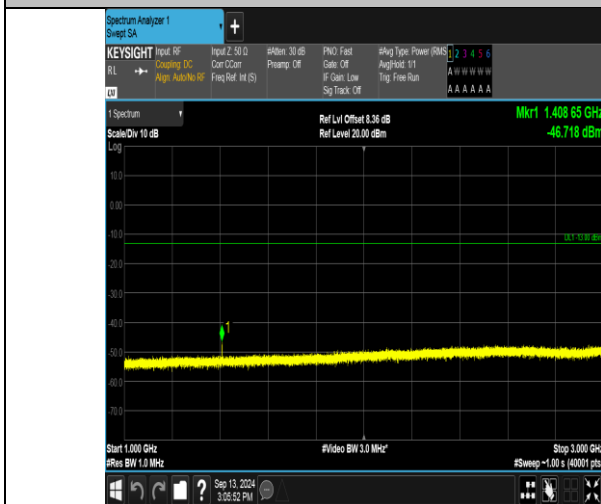
Band17_5MHz_16QAM_23755_1RB#0_1000~3000_1000~3000
