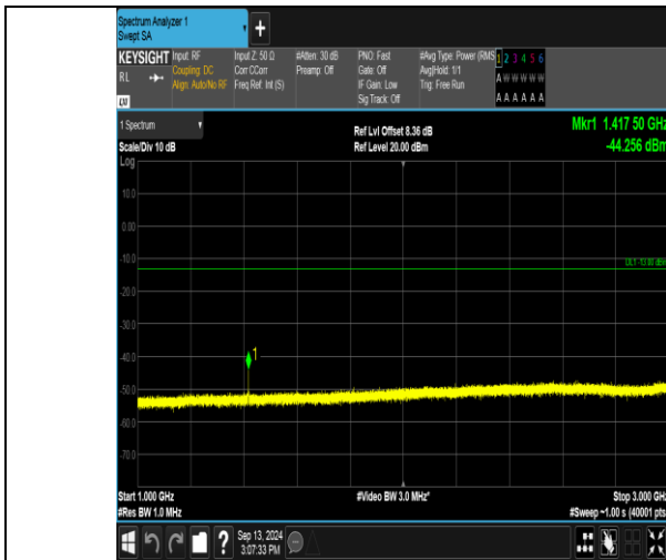
Band17_5MHz_16QAM_23755_1RB#24_1000~3000_1000~3000
