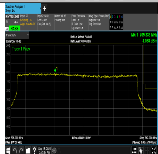
Band17_10MHz_16QAM_23800_50RB#0
