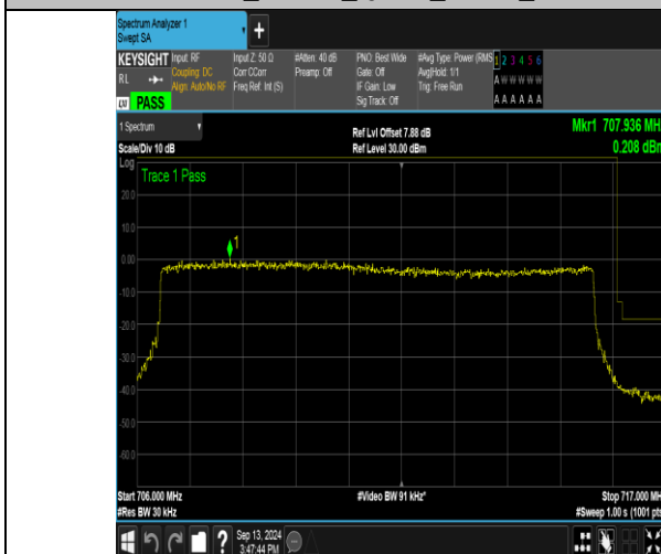
Band17_10MHz_QPSK_23800_50RB#0
