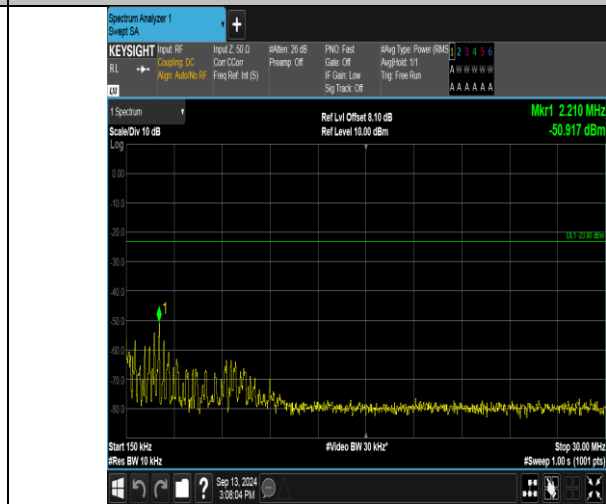
Band17_5MHz_QPSK_23755_25RB#0_0.15~30_0.15~30
