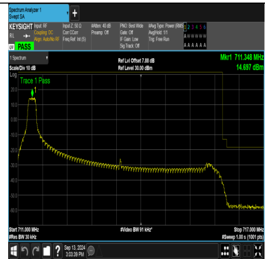
Band17_5MHz_16QAM_23825_1RB#0
