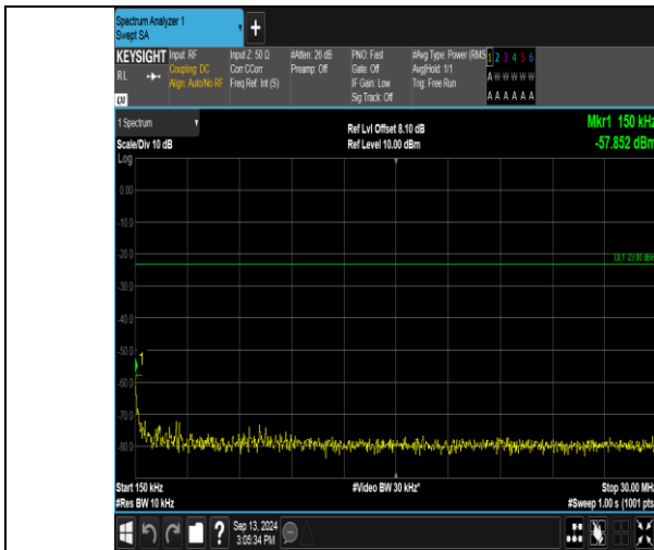
Band17_5MHz_16QAM_23755_1RB#0_0.15~30_0.15~30
