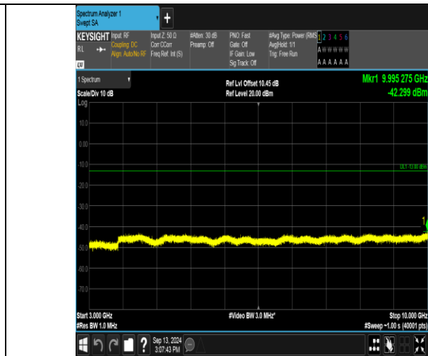
Band17_5MHz_16QAM_23755_1RB#24_3000~10000_3000~10000
