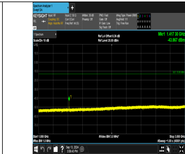
Band17_5MHz_QPSK_23755_1RB#24_1000~3000_1000~3000
