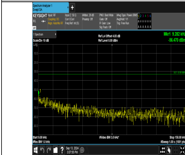
Band17_5MHz_QPSK_23755_25RB#0_0.009~0.15_0.009~0.15
