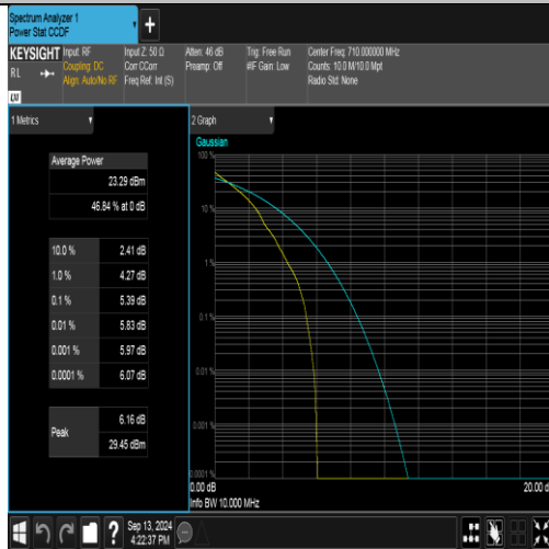
Band17-10MHz-QPSK-23790-1RB#0-PASS
