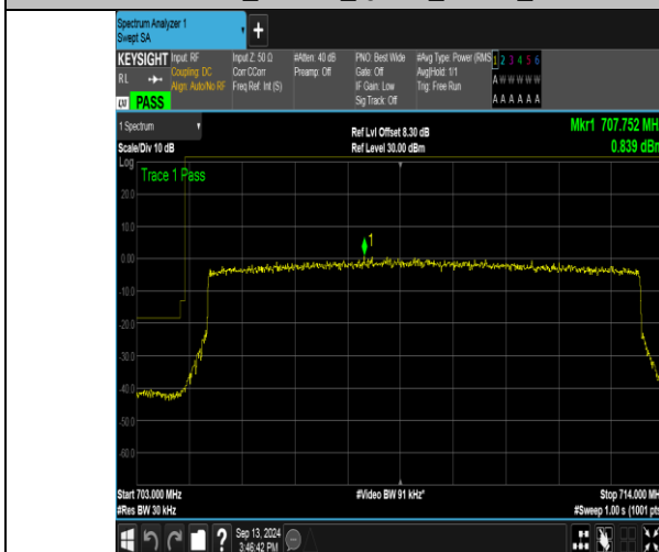
Band17_10MHz_QPSK_23780_50RB#0
