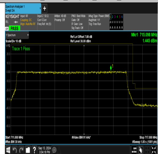
Band17_5MHz_16QAM_23825_25RB#0
