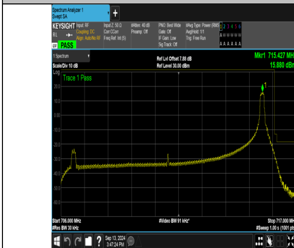
Band17_10MHz_QPSK_23800_1RB#49
