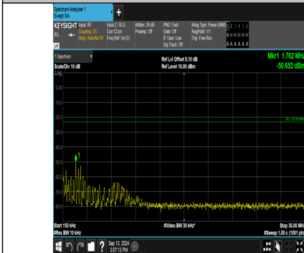
Band17_5MHz_16QAM_23755_1RB#24_0.15~30_0.15~30
