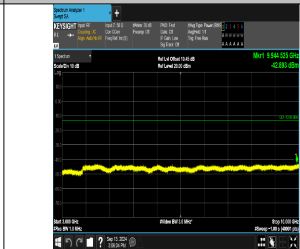
Band17_5MHz_16QAM_23755_1RB#0_3000~10000_3000~10000
