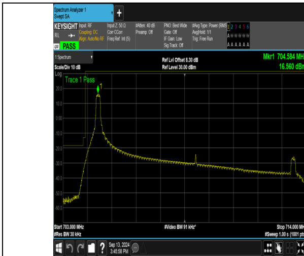
Band17_10MHz_QPSK_23780_1RB#0
