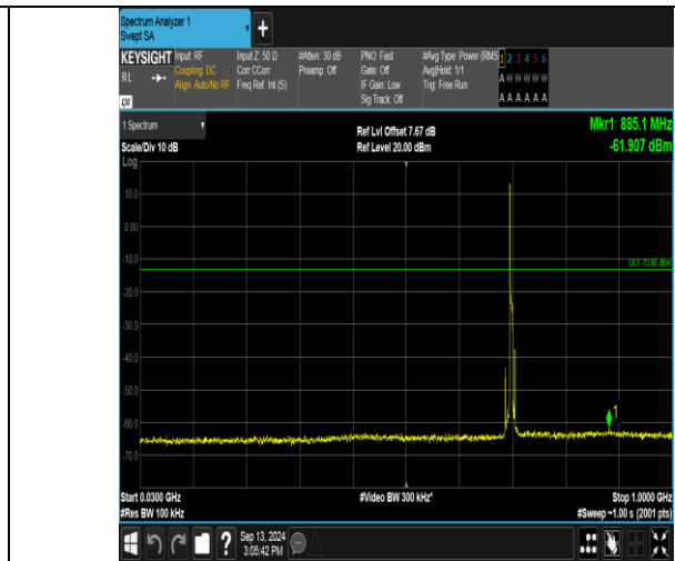
Band17_5MHz_16QAM_23755_1RB#0_30~1000_30~1000
