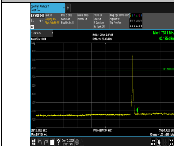
Band17_5MHz_QPSK_23755_25RB#0_30~1000_30~1000
