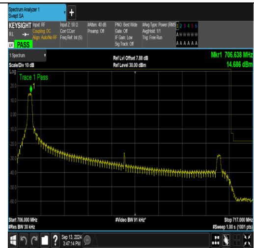
Band17_10MHz_16QAM_23800_1RB#0
