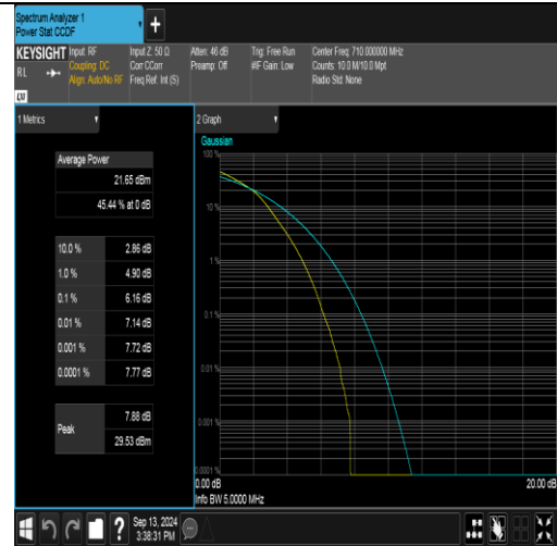
Band17-5MHz-16QAM-23790-25RB#0-PASS
