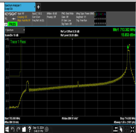
Band17_10MHz_16QAM_23780_1RB#49
