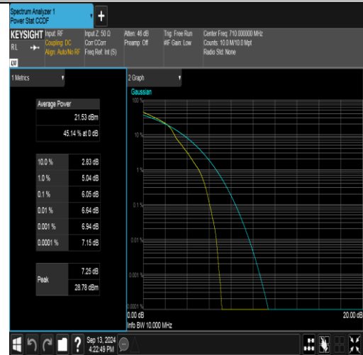
Band17-10MHz-16QAM-23790-1RB#0-PASS
