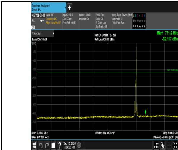
Band17_5MHz_QPSK_23755_1RB#24_30~1000_30~1000
