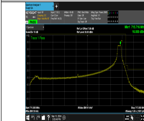
Band17_5MHz_QPSK_23825_1RB#24
