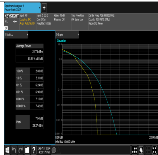
Band17-10MHz-16QAM-23780-1RB#0-PASS
