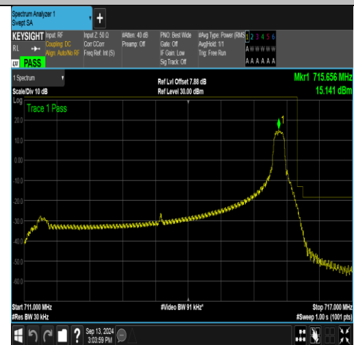
Band17_5MHz_16QAM_23825_1RB#24
