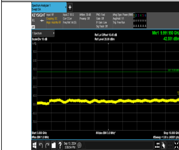
Band17_5MHz_QPSK_23755_1RB#24_3000~10000_3000~10000
