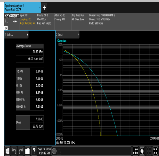
Band17-10MHz-16QAM-23780-50RB#0-PASS
