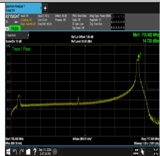
Band17_10MHz_16QAM_23800_1RB#49
