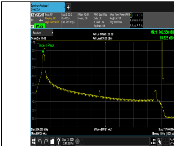
Band17_10MHz_QPSK_23800_1RB#0
