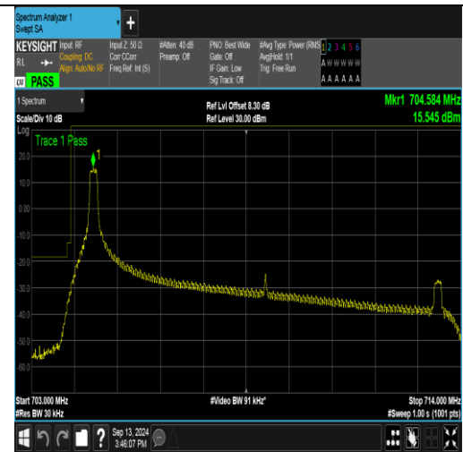
Band17_10MHz_16QAM_23780_1RB#0
