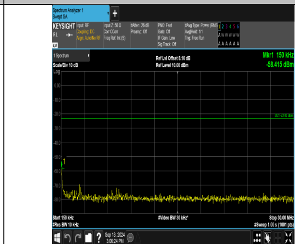
Band17_5MHz_QPSK_23755_1RB#24_0.15~30_0.15~30
