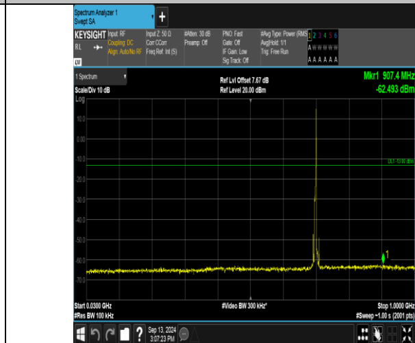
Band17_5MHz_16QAM_23755_1RB#24_30~1000_30~1000
