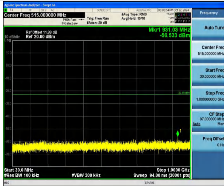
DH5-Ant1-2441-30~1000-PASS
