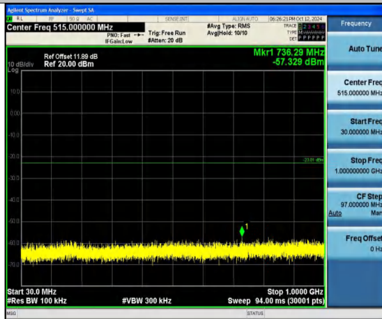
3DH5-Ant1-2402-30~1000-PASS
