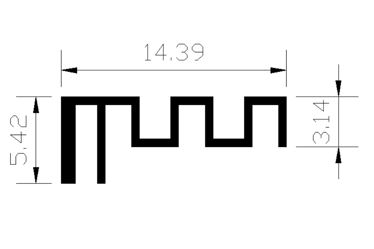
Antenna Photo & Length(mm)
