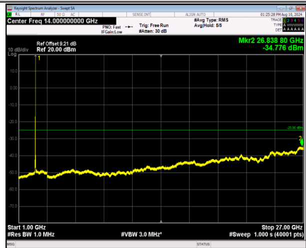
7-7-20MHz-10MHz-16QAM-16QAM-21051-21195-1RB#99- ORB#0-1000~27000MHz-PASS
