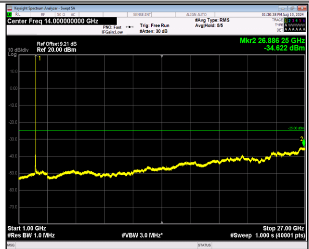
7-7-20MHz-10MHz-16QAM-16QAM-21251-21395-1RB#99- ORB#0-1000~27000MHz-PASS
