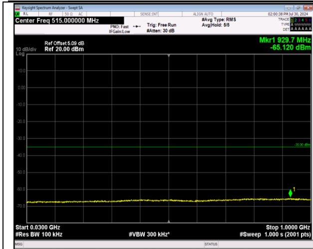
7-7-20MHz-10MHz-64QAM-64QAM-20850-20994-1RB#9 9-0RB#0-30~1000MHz-PASS
