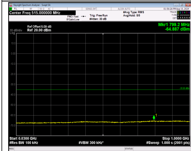
7-7-20MHz-20MHz-QPSK-QPSK-20850-21048-100RB#0- -100RB#0-30~1000MHz-PASS
