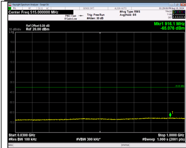
7-7-20MHz-10MHz-16QAM-16QAM-21251-21395-1RB#0 -ORB#0-30~1000MHz-PASS
