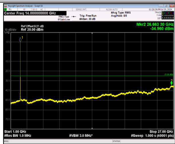
7-7-10MHz-20MHz-64QAM-64QAM-21206-21350-50RB#0- 100RB#0-1000~27000MHz-PASS
