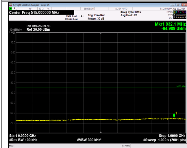
7-7-20MHz-10MHz-16QAM-16QAM-20850-20994-1RB#9 9-ORB#0-30~1000MHz-PASS
