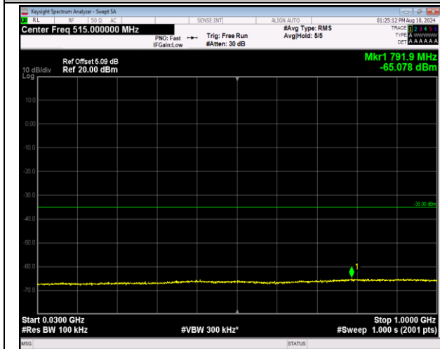
7-7-20MHz-10MHz-16QAM-16QAM-21051-21195-1RB#9 9-ORB#0-30~1000MHz-PASS
