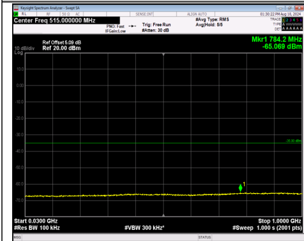
7-7-20MHz-10MHz-16QAM-16QAM-21251-21395-1RB#9 9-ORB#0-30~1000MHz-PASS
