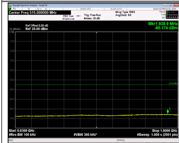
7-7-20MHz-10MHz-64QAM-64QAM-20850-20994-100RB #0-50RB#0-30~1000MHz-PASS
