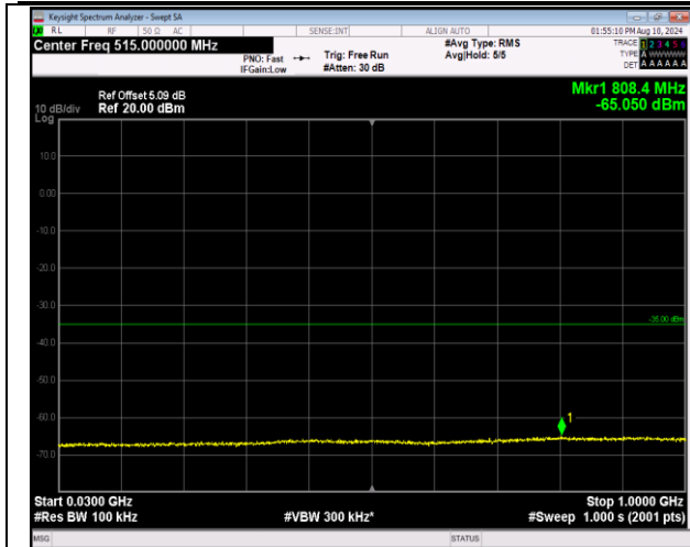
7-7-20MHz-20MHz-QPSK-QPSK-20850-21048-1RB#0-1 RB#99-30~1000MHz-PASS
