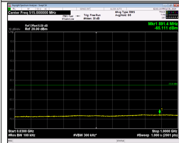
7-7-20MHz-10MHz-64QAM-64QAM-20850-20994-1RB#0 -1RB#49-30~1000MHz-PASS
