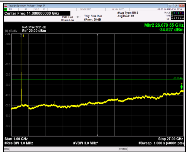
7-7-20MHz-10MHz-64QAM-64QAM-20850-20994-1RB#0-0 RB#0-1000~27000MHz-PASS
