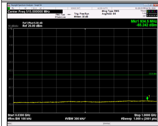
7-7-10MHz-20MHz-64QAM-64QAM-21206-21350-50RB#- 0-100RB#0-30~1000MHz-PASS
