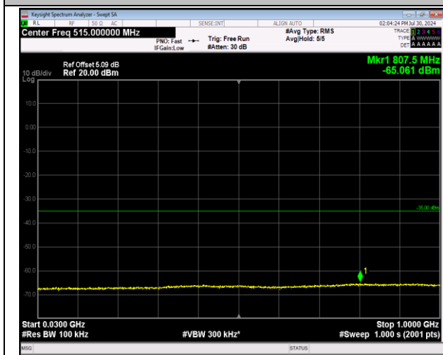
7-7-20MHz-10MHz-64QAM-64QAM-21051-21195-100RB #0-50RB#0-30~1000MHz-PASS
