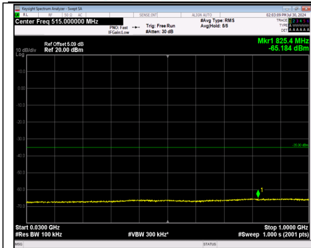
7-7-20MHz-10MHz-64QAM-64QAM-21051-21195-1RB#9 9-0RB#0-30~1000MHz-PASS
