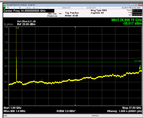
7-7-20MHz-20MHz-64QAM-64QAM-20850-21048-1RB#0-0 RB#0-1000~27000MHz-PASS
