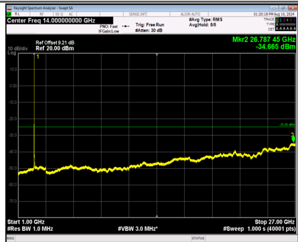
7-7-20MHz-10MHz-16QAM-16QAM-20850-20994-1RB#99- ORB#0-1000~27000MHz-PASS
