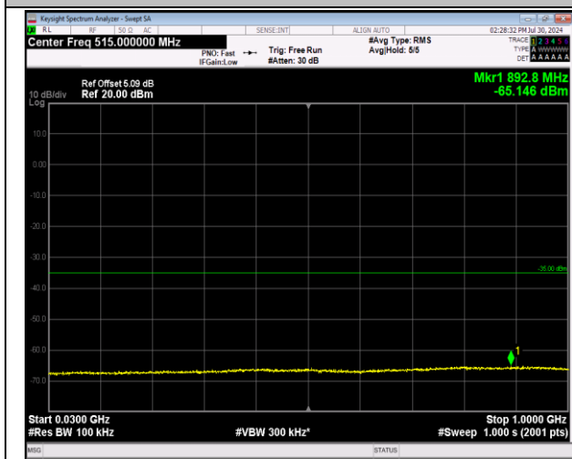
7-7-20MHz-20MHz-64QAM-64QAM-20850-21048-1RB#0 -0RB#0-30~1000MHz-PASS
