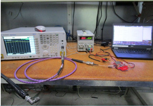
Conducted RF
