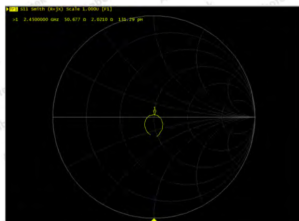
Impedance Test-Body
