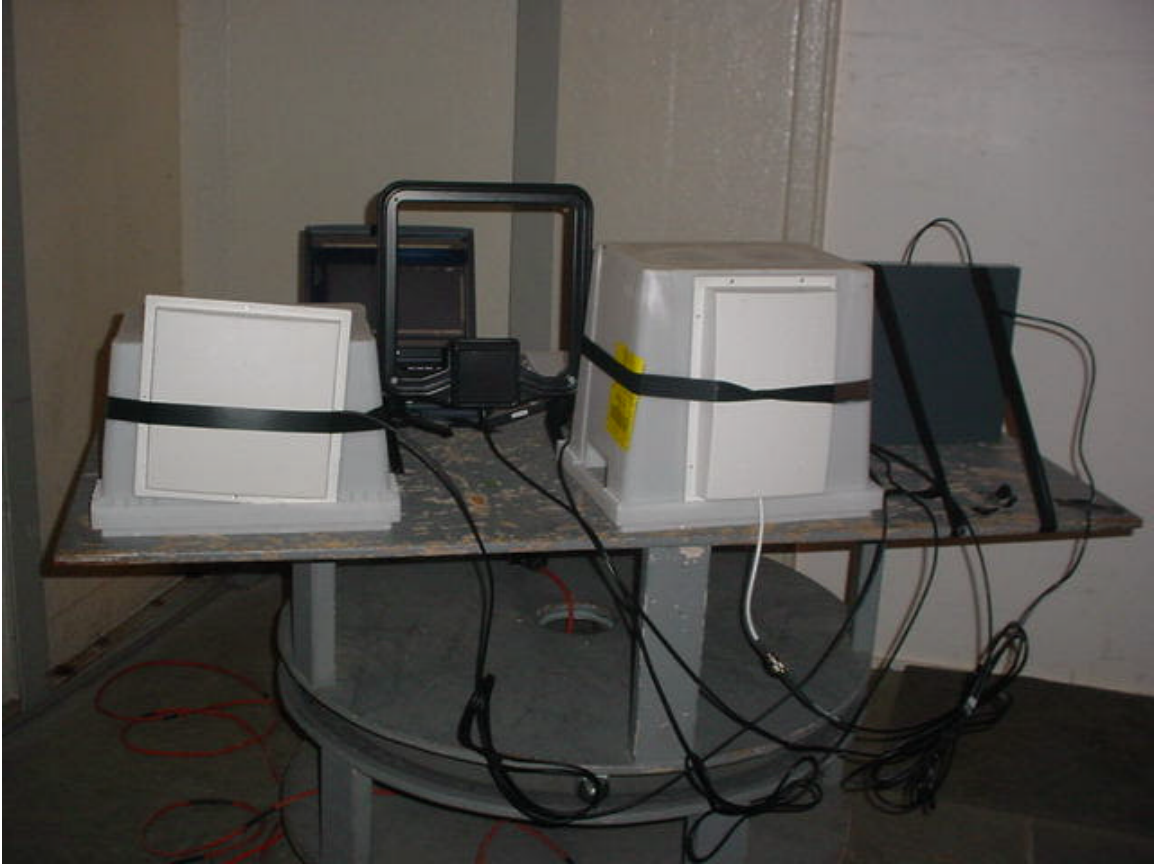
Radiated EMI
