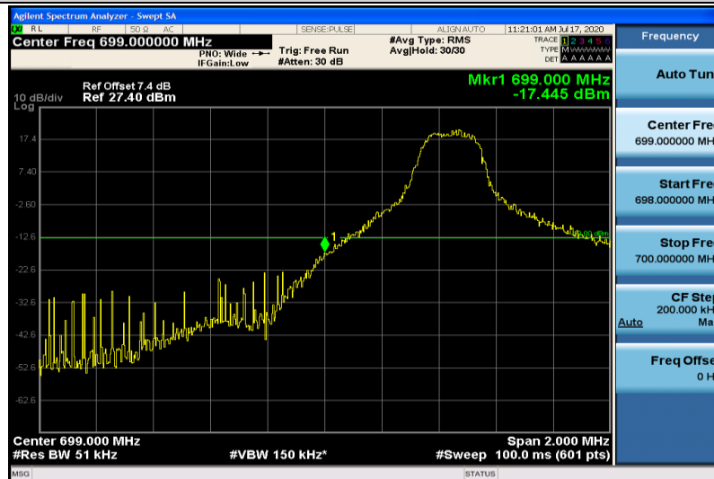
Band12-5MHz-16QAM-23035-1RB#0
