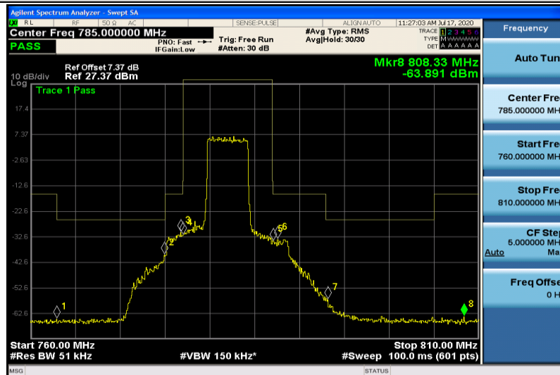
Band13-5MHz-QPSK-23230-25RB#0
