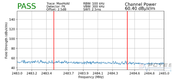
Plot 7-76. Radiated Restricted Upper Band Edge Measurement MIMO (Peak – 242 Tones)
