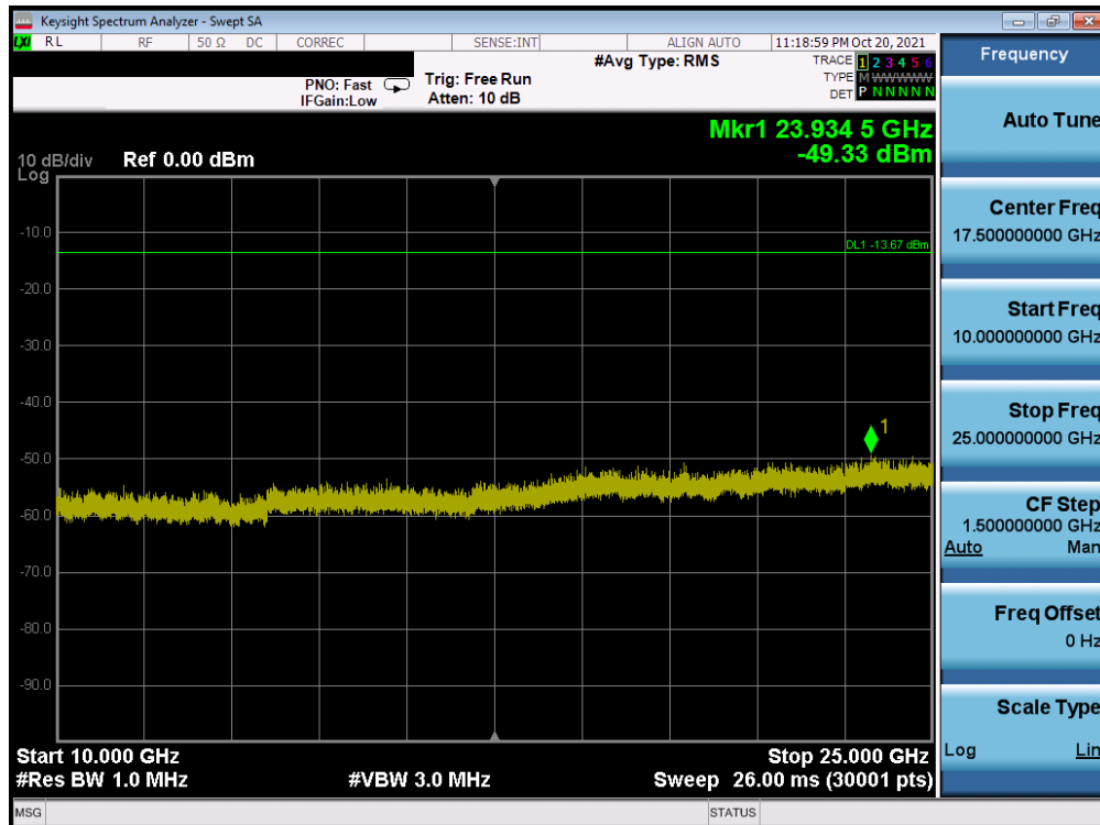
Plot 7-44. Conducted Spurious Plot MIMO ANT1 (802.11ax OFDMA – 242 Tones – Ch. 6)
