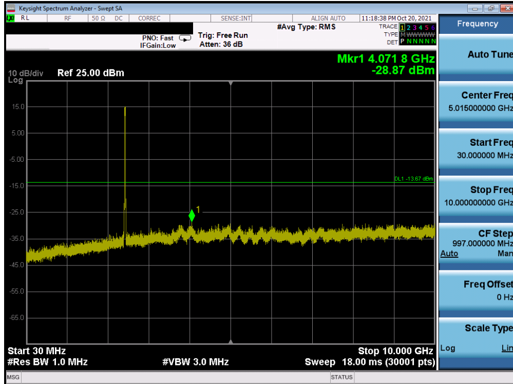
Plot 7-43. Conducted Spurious Plot MIMO ANT1 (802.11ax OFDMA – 242 Tones – Ch. 6)
