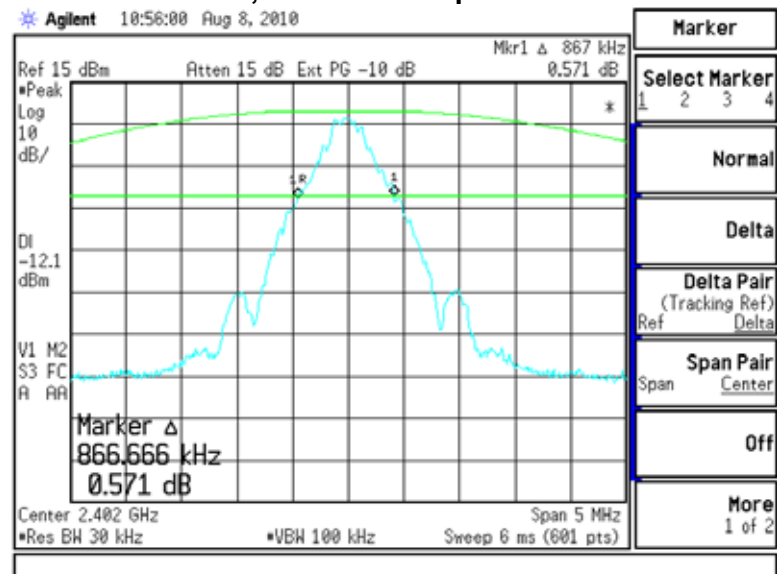
Channel 1, -20 dBc Occupied Bandwidth
