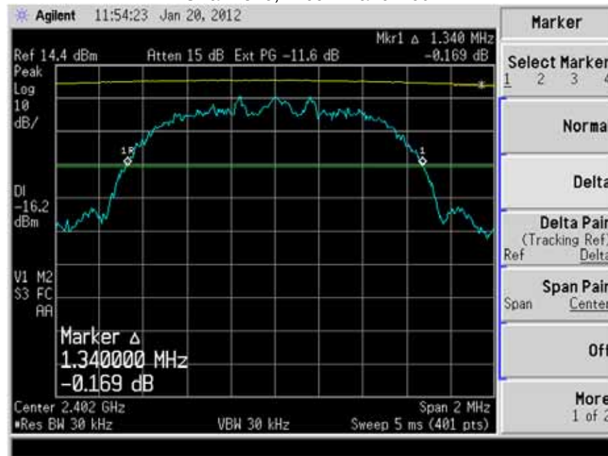
Channel 0, -26dB Bandwidth
