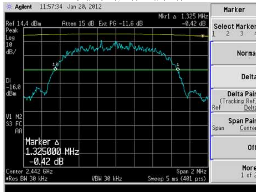
Channel 20, -26dB Bandwidth
