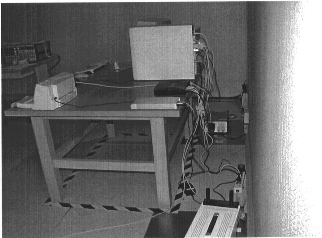
Back View of Conducted Test ( Mode 1)
