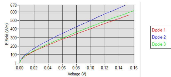
Calibration curves
