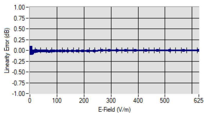
Linearity
