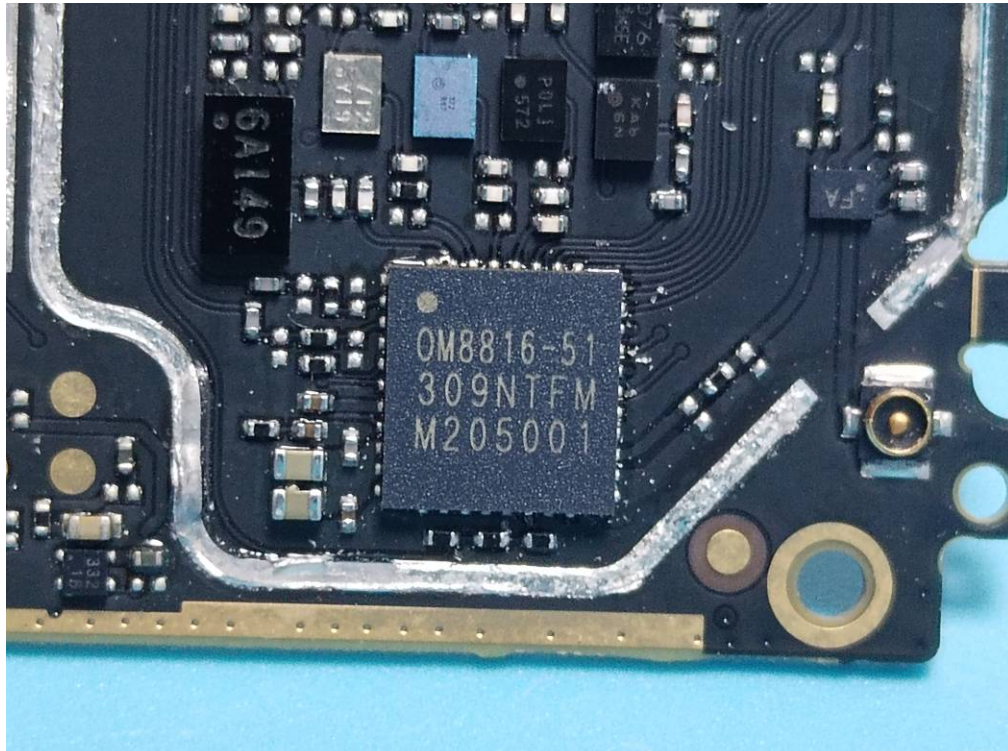
Main ANT (GSM850/WCDMA B5/LTE B5/B7/B12/B41 transmit on Main antenna)
