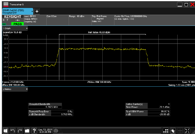
n7_10MHz_15kHz_2535MHz_CP-OFDM 256 QAM_RB52@0
