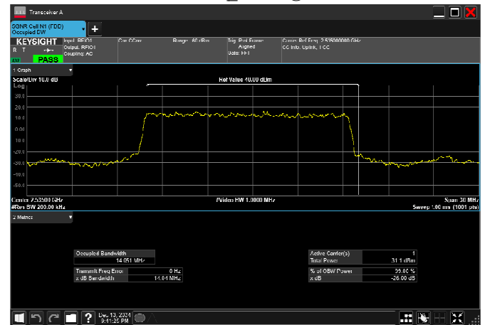
n7_15MHz_15kHz_2535MHz_DFT-s-OFDM 16 QAM_RB75@0
