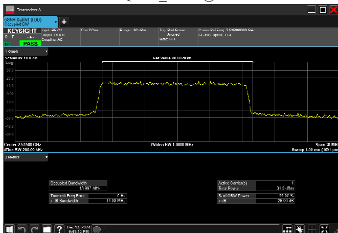
n7_15MHz_15kHz_2535MHz_DFT-s-OFDM QPSK_RB75@0
