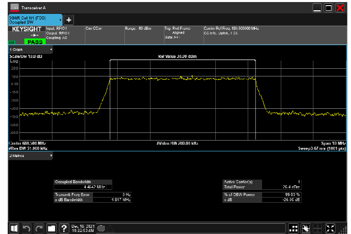
n71_5MHz_15kHz_680.5MHz_CP-OFDM 16 QAM_RB25@0
