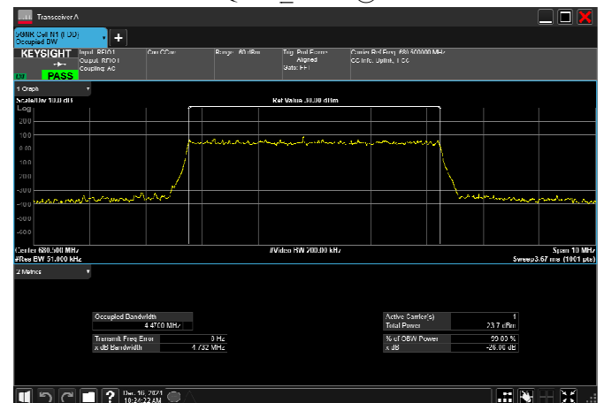
n71_5MHz_15kHz_680.5MHz_CP-OFDM 256 QAM_RB25@0
