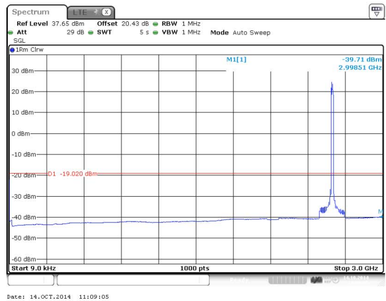
Figure 221 Spurious Emissions (9kHz – 3GHz) – 16QAM (2593.0 MHz) (20MHz Channel BW)
