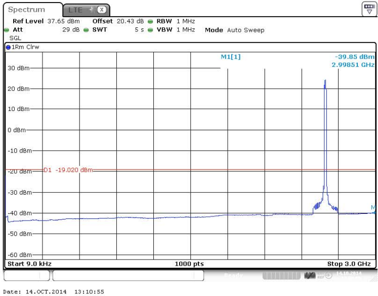
Figure 213 Spurious Emissions (9kHz – 3GHz) – 64QAM (2593.0 MHz) (20MHz Channel BW)
