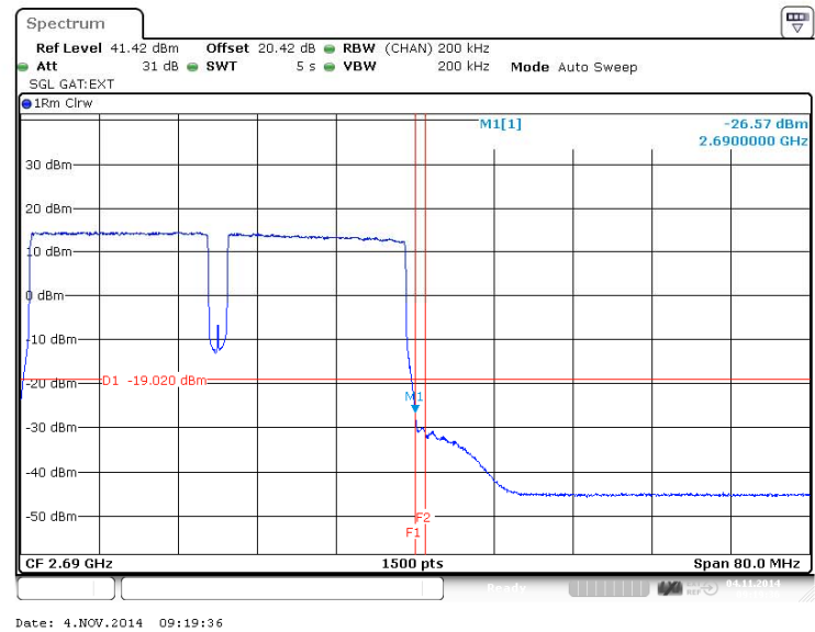
Figure 248 Spurious Emissions (Upper Band Edge) – 64QAM (2660.0/2680.0 MHz) (20MHz Channel BW)
