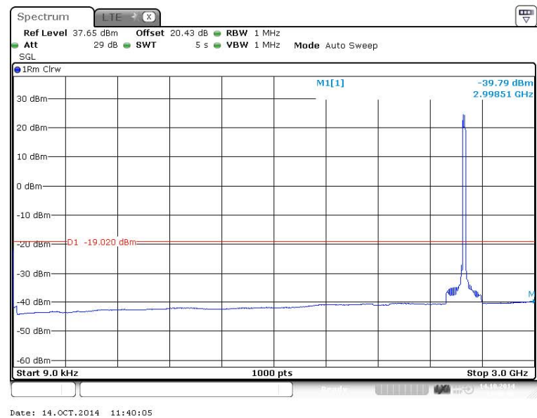
Figure 217 Spurious Emissions (9kHz – 3GHz) - QPSK (2593.0 MHz) (20MHz Channel BW)
