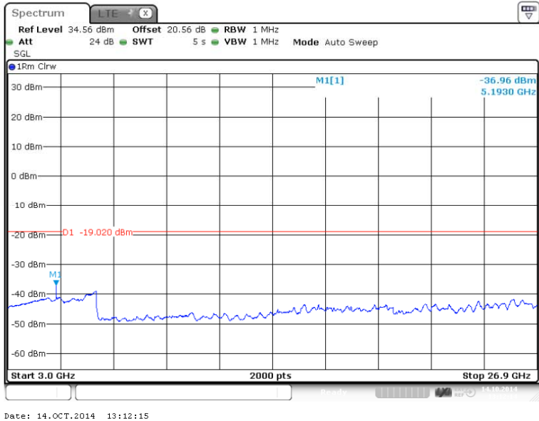
Figure 214 Spurious Emissions (3GHz – 26.900GHz) – 64QAM (2593.0 MHz) (20MHz Channel BW)
