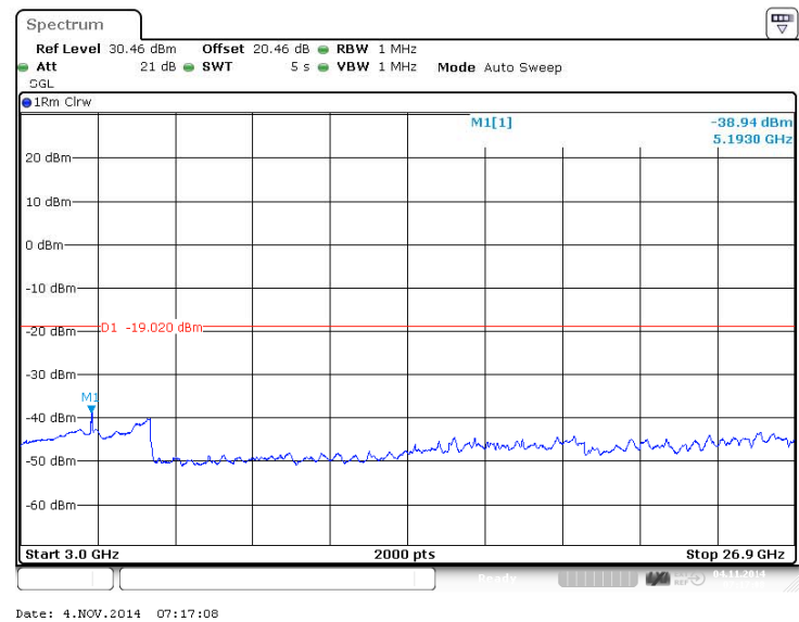
Figure 258 Spurious Emissions (3GHz – 26.900GHz) – 16QAM (2583.0/2603.0 MHz) (20MHz Channel BW)
