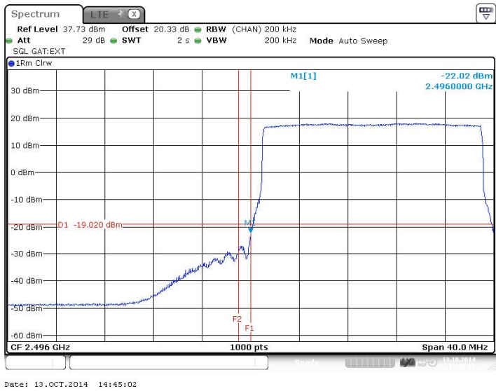
Figure 215 Spurious Emissions (Lower Band Edge) – QPSK (2506.0 MHz) (20MHz Channel BW)
