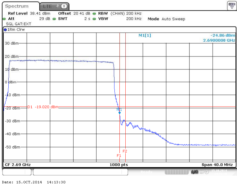
Figure 212 Spurious Emissions (Upper Band Edge) – 64QAM (2680.0 MHz) (20MHz Channel BW)
