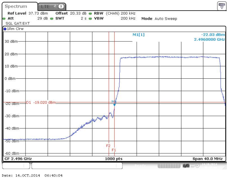
Figure 235 Spurious Emissions (Lower Band Edge) – 64QAM (2506.0 MHz) (20MHz Channel BW)
