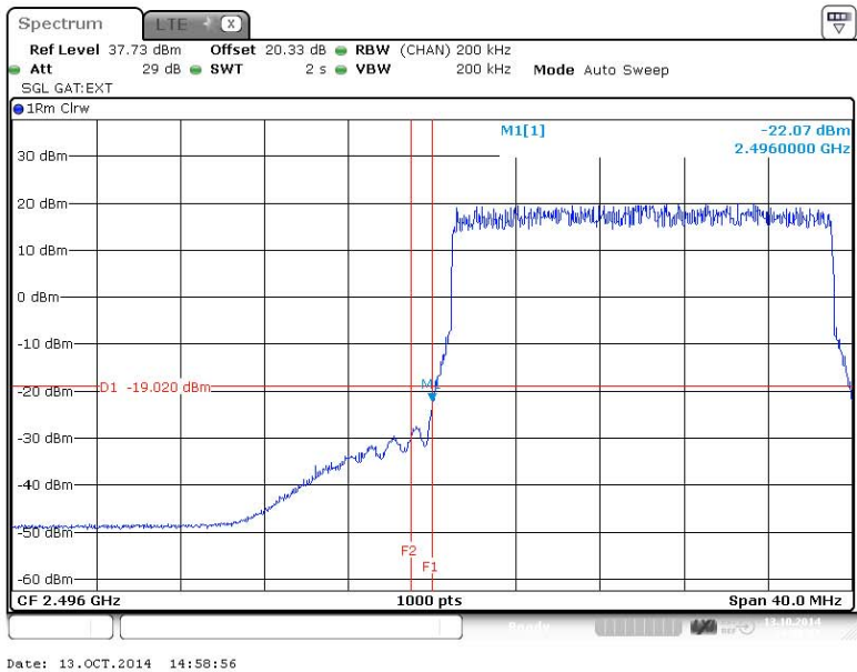
Figure 219 Spurious Emissions (Lower Band Edge) – 16QAM (2506.0 MHz) (20MHz Channel BW)
