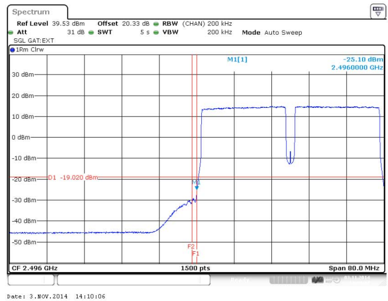
Figure 247 Spurious Emissions (Lower Band Edge) – 64QAM (2506.0/2526.0 MHz) (20MHz Channel BW)
