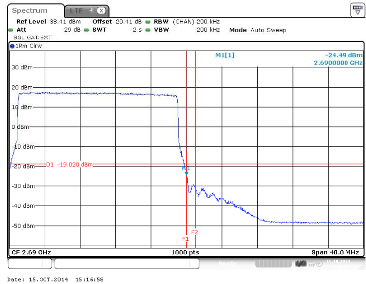
Figure 224 Spurious Emissions (Upper Band Edge) – 64QAM (2680.0 MHz) (20MHz Channel BW)
