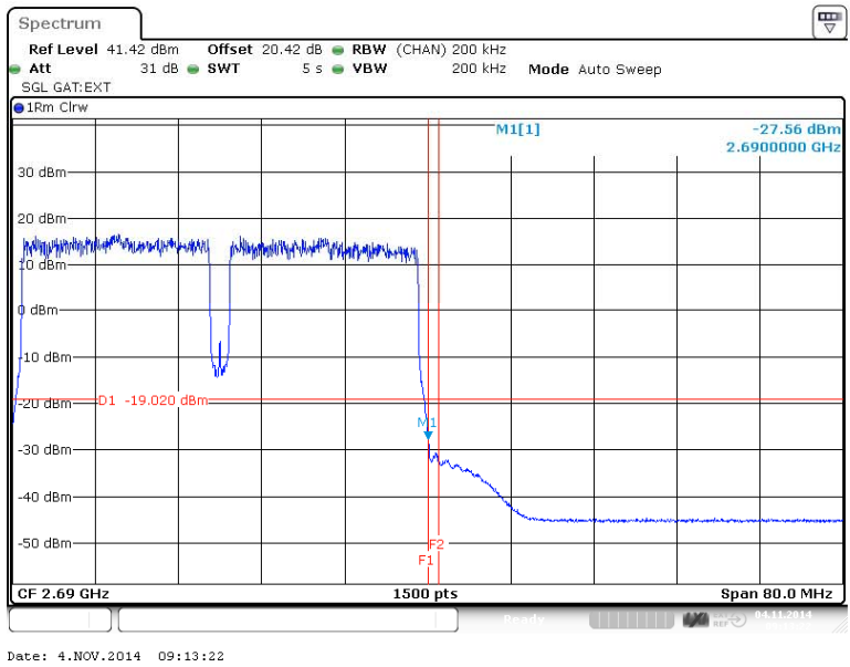
Figure 244 Spurious Emissions (Upper Band Edge) – 16QAM (2660.0/2680.0 MHz) (20MHz Channel BW)
