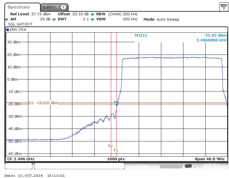
Figure 223 Spurious Emissions (Lower Band Edge) – 64QAM (2506.0 MHz) (20MHz Channel BW)
