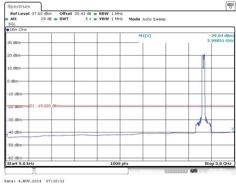
Figure 253 Spurious Emissions (9kHz – 3GHz) - QPSK (2583.0/2603.0 MHz) (20MHz Channel BW)
