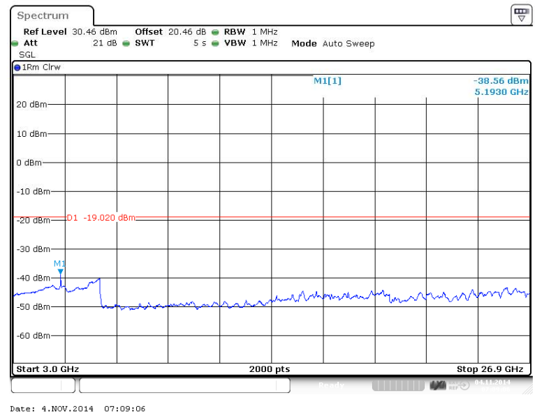
Figure 254 Spurious Emissions (3GHz – 26.900GHz) – QPSK (2583.0/2603.0 MHz) (20MHz Channel BW)
