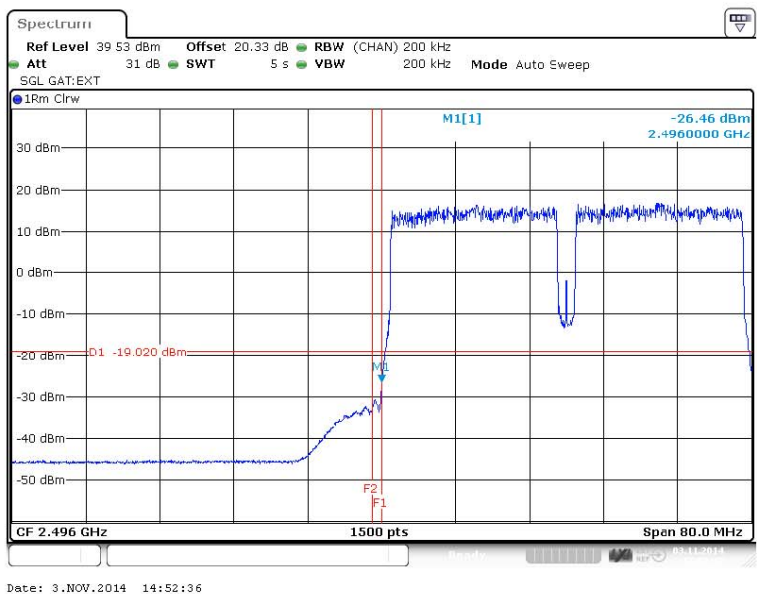
Figure 255 Spurious Emissions (Lower Band Edge) – 16QAM (2506.0/2526.0 MHz) (20MHz Channel BW)
