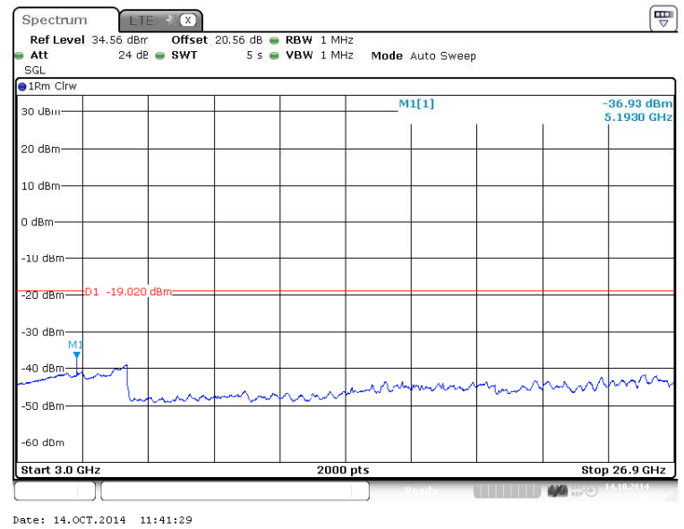
Figure 218 Spurious Emissions (3GHz – 26.900GHz) – QPSK (2593.0 MHz) (20MHz Channel BW)
