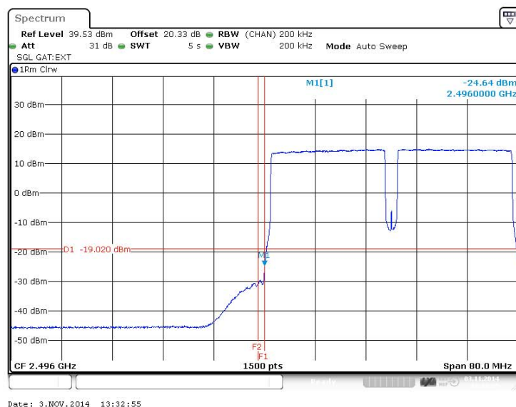
Figure 239 Spurious Emissions (Lower Band Edge) – QPSK (2506.0/2526.0 MHz) (20MHz Channel BW)
