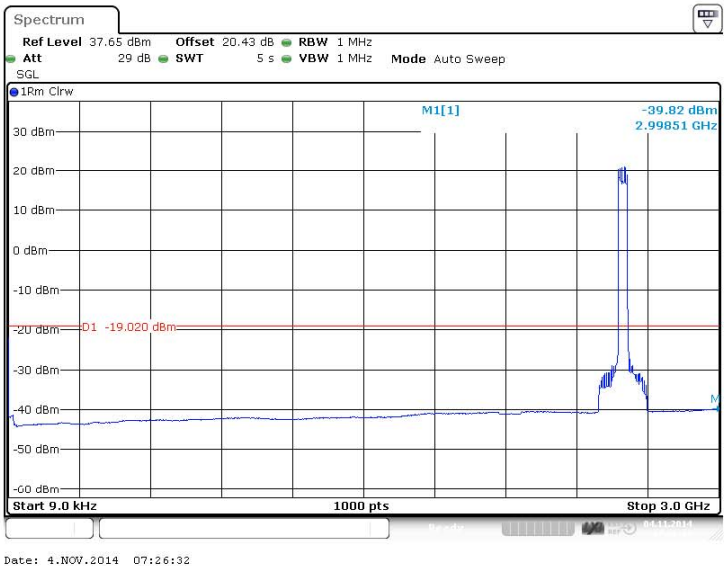
Figure 261 Spurious Emissions (9kHz – 3GHz) – 64QAM (2583.0/2603.0 MHz) (20MHz Channel BW)
