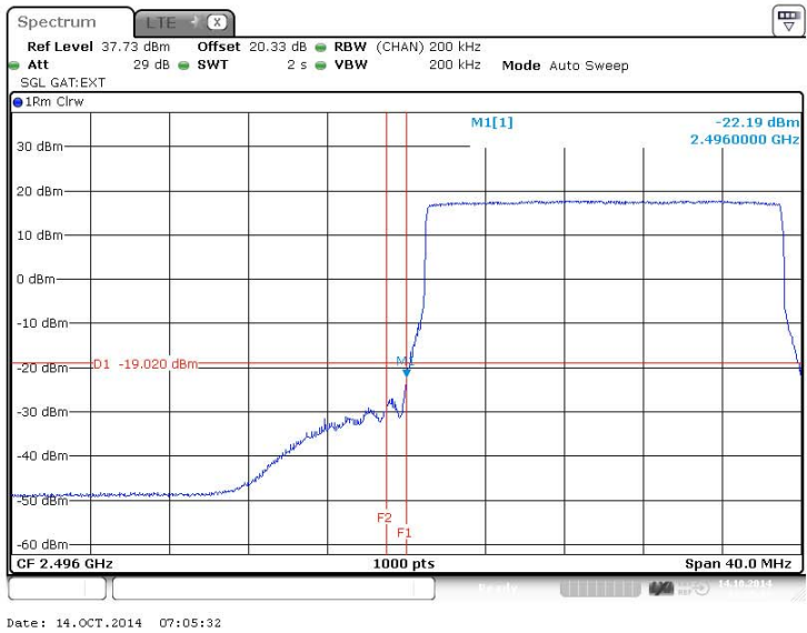
Figure 227 Spurious Emissions (Lower Band Edge) – QPSK (2506.0 MHz) (20MHz Channel BW)
