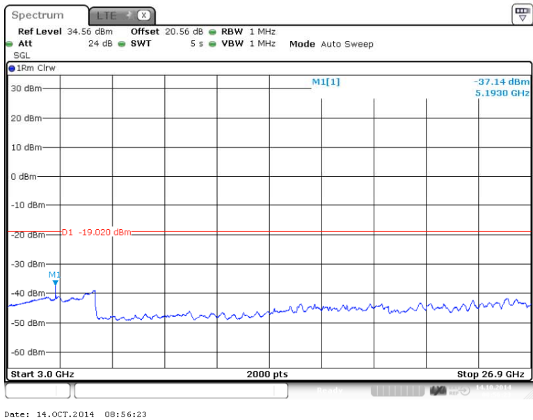
Figure 234 Spurious Emissions (3GHz – 26.900GHz) – 16QAM (2593.0 MHz) (20MHz Channel BW)
