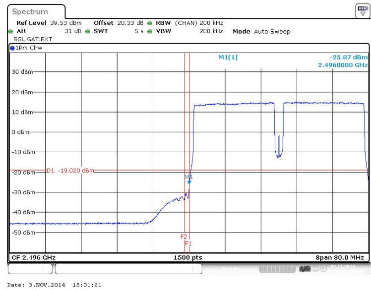
Figure 259 Spurious Emissions (Lower Band Edge) – 64QAM (2506.0/2526.0 MHz) (20MHz Channel BW)
