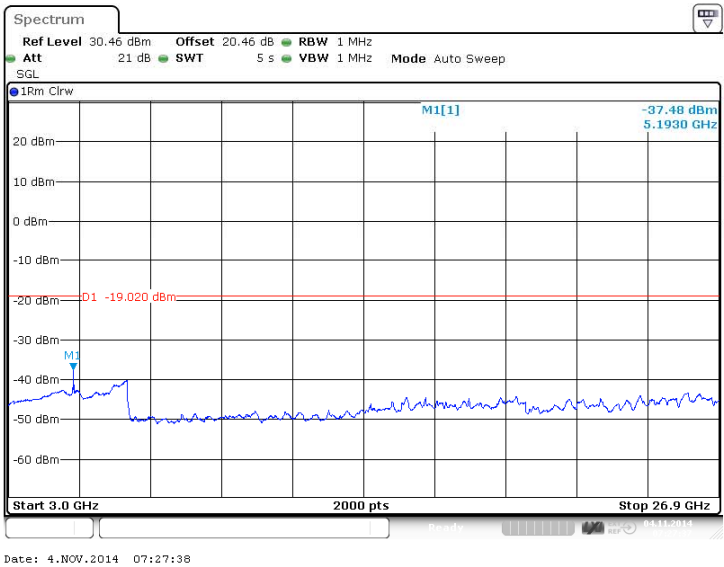
Figure 262 Spurious Emissions (3GHz – 26.900GHz) – 64QAM (2583.0/2603.0 MHz) (20MHz Channel BW)
