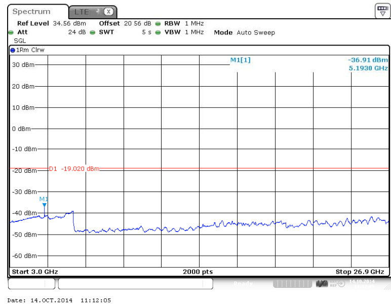
Figure 222 Spurious Emissions (3GHz – 26.900GHz) – 16QAM (2593.0 MHz) (20MHz Channel BW)
