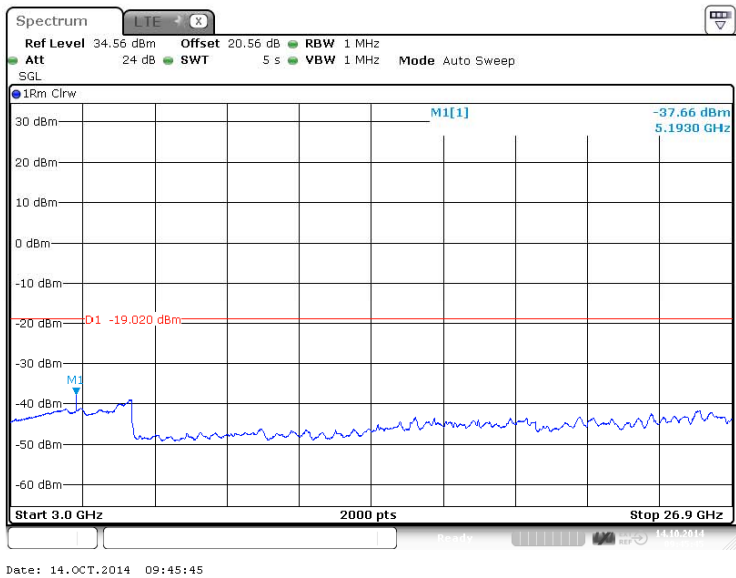
Figure 226 Spurious Emissions (3GHz – 26.900GHz) – 64QAM (2593.0 MHz) (20MHz Channel BW)
