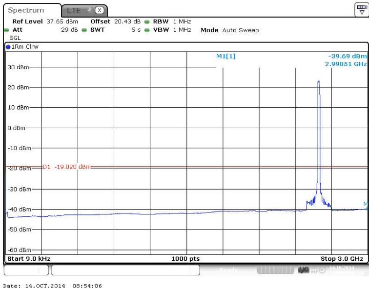
Figure 233 Spurious Emissions (9kHz – 3GHz) – 16QAM (2593.0 MHz) (20MHz Channel BW)
