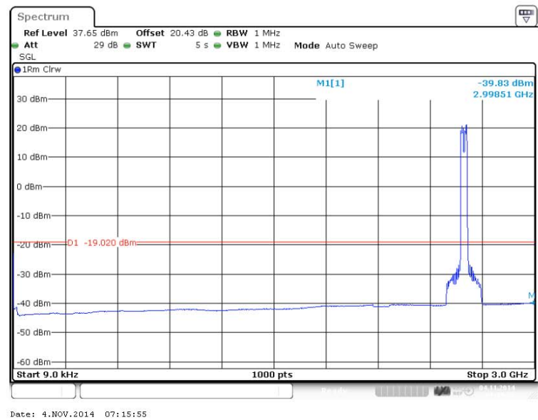
Figure 257 Spurious Emissions (9kHz – 3GHz) – 16QAM (2583.0/2603.0 MHz) (20MHz Channel BW)
