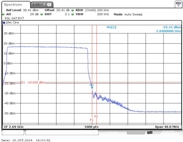
Figure 228 Spurious Emissions (Upper Band Edge) – QPSK (2680.0 MHz) (20MHz Channel BW)
