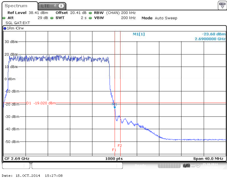
Figure 220 Spurious Emissions (Upper Band Edge) – 16QAM (2680.0 MHz) (20MHz Channel BW)
