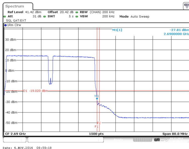
Figure 240 Spurious Emissions (Upper Band Edge) – QPSK (2660.0/2680.0 MHz) (20MHz Channel BW)
