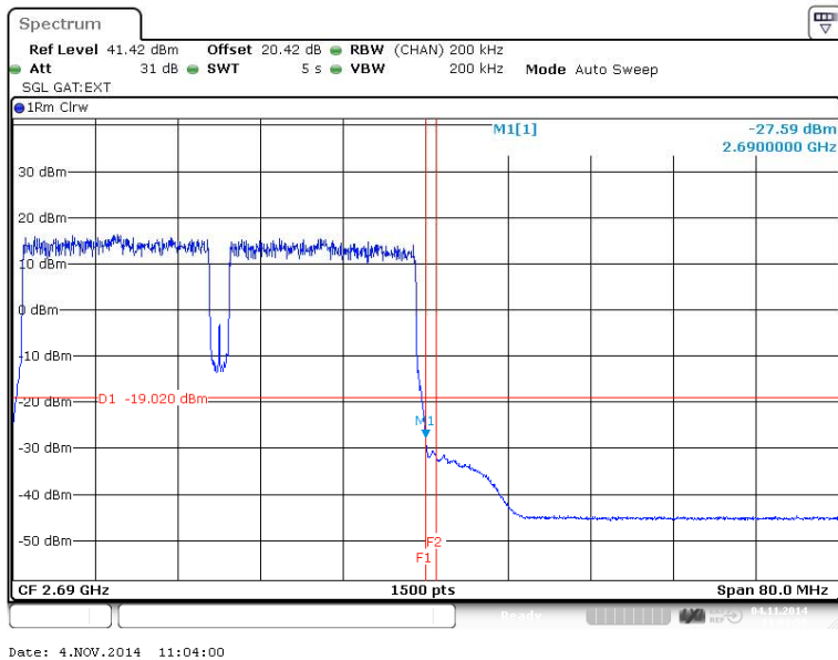
Figure 256 Spurious Emissions (Upper Band Edge) – 16QAM (2660.0/2680.0 MHz) (20MHz Channel BW)
