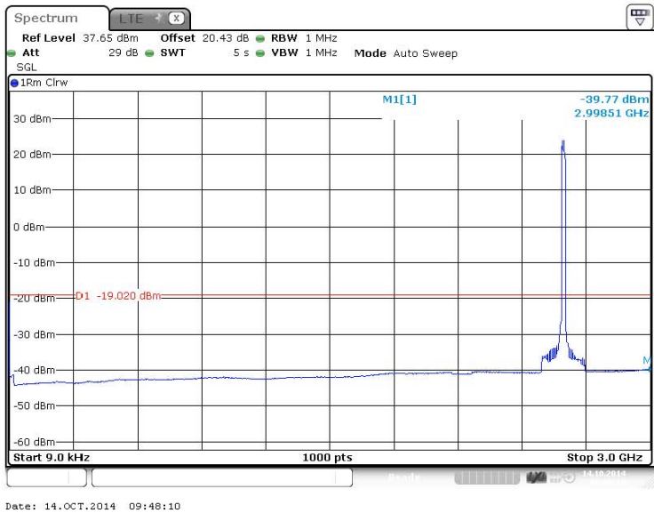
Figure 225 Spurious Emissions (9kHz – 3GHz) – 64QAM (2593.0 MHz) (20MHz Channel BW)
