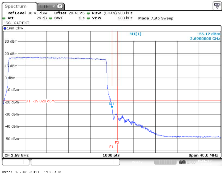
Figure 236 Spurious Emissions (Upper Band Edge) – 64QAM (2680.0 MHz) (20MHz Channel BW)
