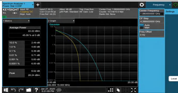
Band2-15MHz-QPSK-18900-75RB#0-PASS
