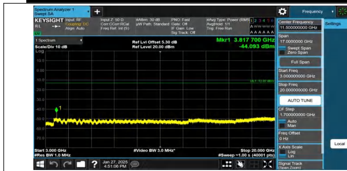
Band2-1.4MHz-QPSK-19193-1RB#0-3000~20000-PASS
