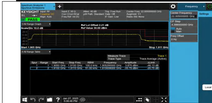
Band2-5MHz-QPSK-19175-25RB#0-PASS
