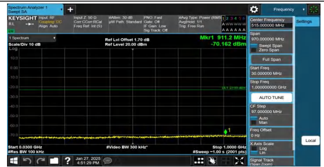
Band2-1.4MHz-QPSK-19193-1RB#5-30~1000-PASS
