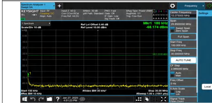
Band2-1.4MHz-QPSK-19193-1RB#5-0.15~30-PASS
