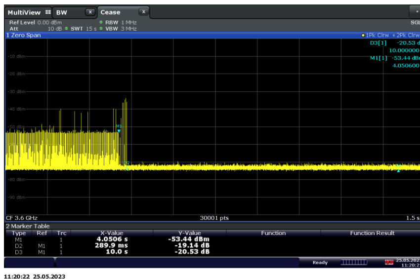
Plot 7-69. Run#1 End User Device Discontinues Operations within 10s
