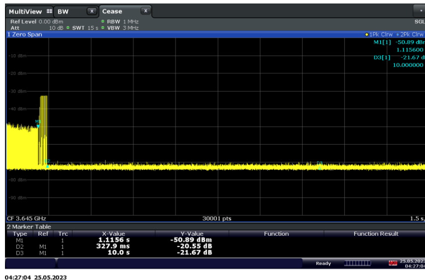
Plot 7-71. Run#2 End User Device Discontinues Operations within 10s
