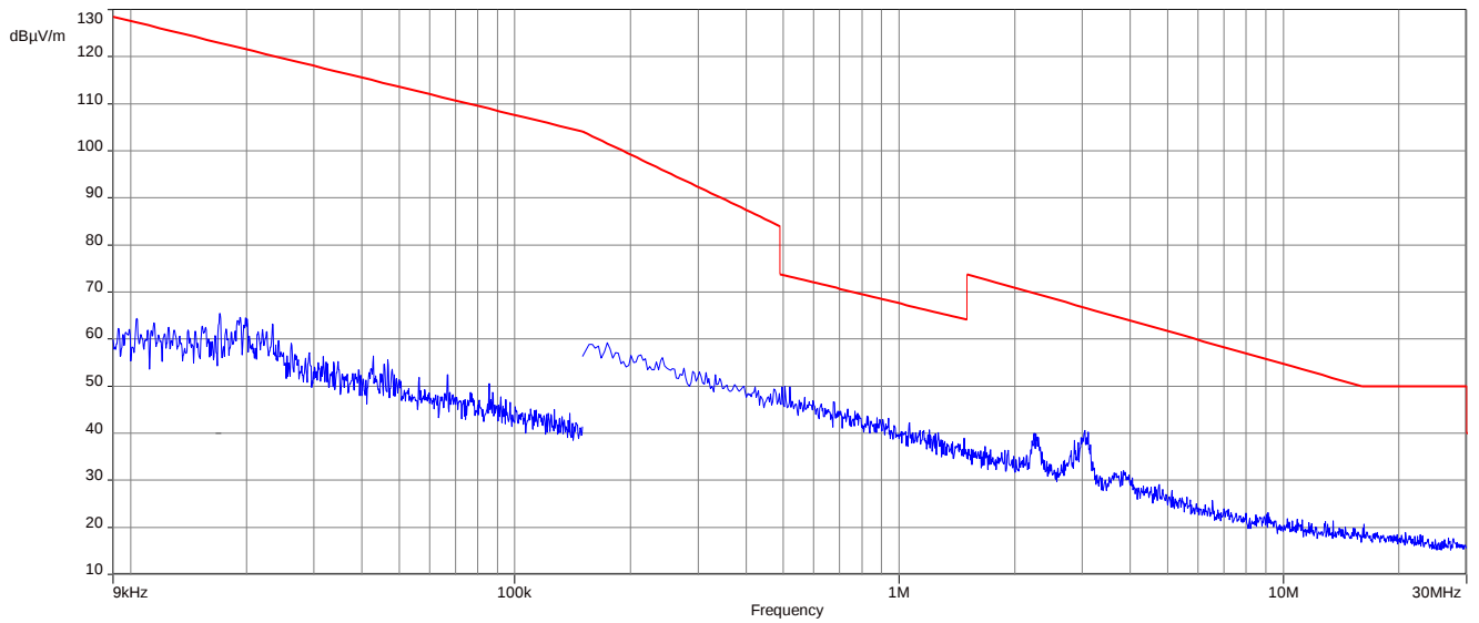
Plot 27: 9 kHz to 30 MHz, U-NII-2A; lowest channel
