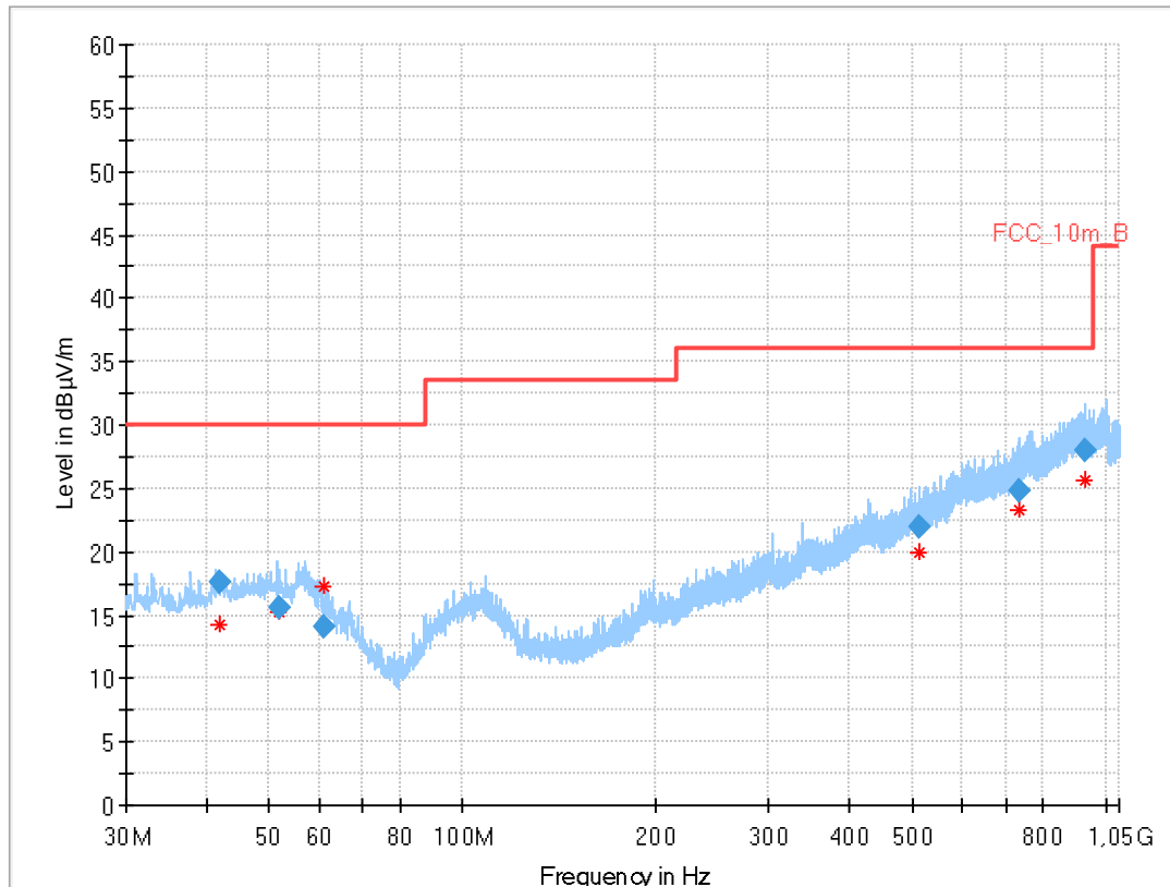
Plot 10: 30 MHz to 1 GHz; vertical & horizontal polarization; U-NII-3; lowest channel
