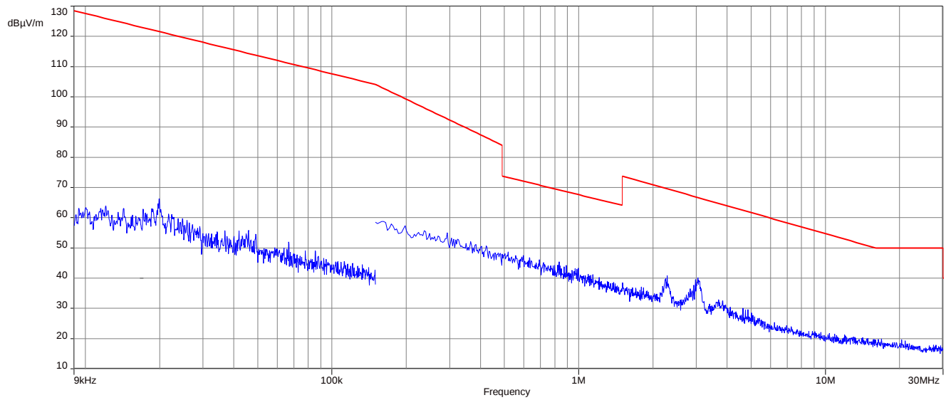
Plot 31: 9 kHz to 30 MHz, U-NII-2C; highest channel
