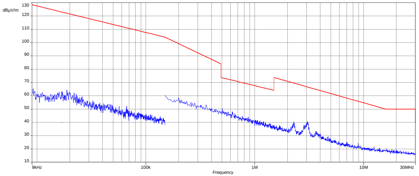
Plot 41: 9 kHz to 30 MHz, U-NII-2C; highest channel
