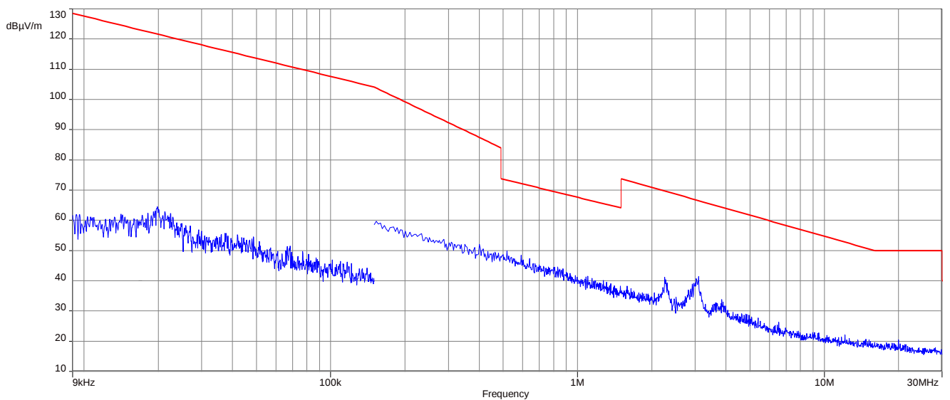
Plot 47: 9 kHz to 30 MHz, U-NII-2C; highest channel
