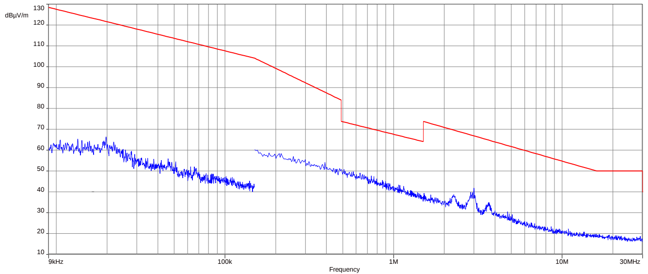
Plot 17: 9 kHz to 30 MHz, U-NII-2C; highest channel
