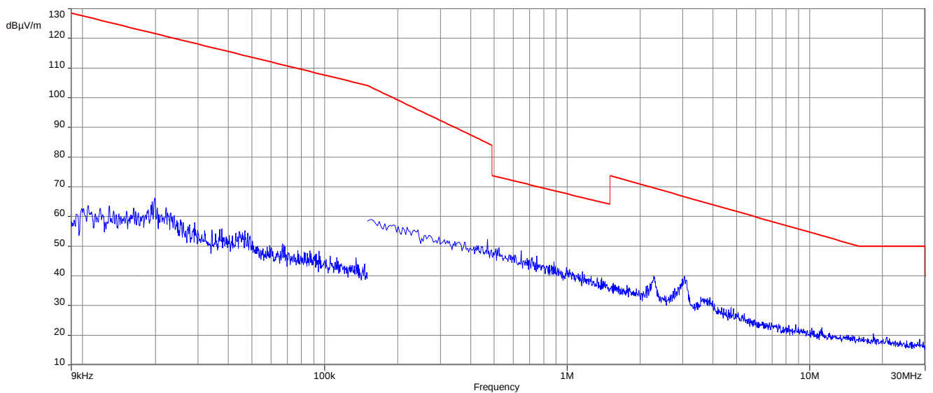
Plot 34: 9 kHz to 30 MHz, U-NII-3; highest channel
