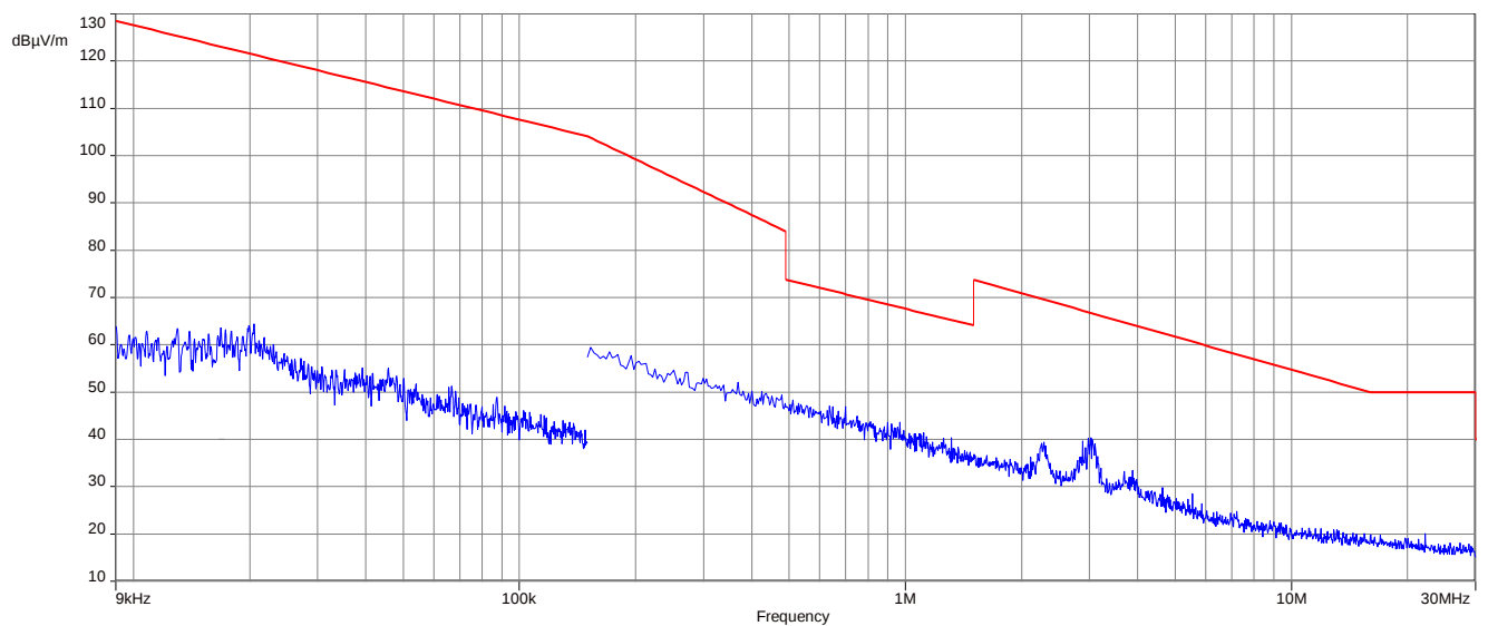
Plot 32: 9 kHz to 30 MHz, U-NII-3; lowest channel
