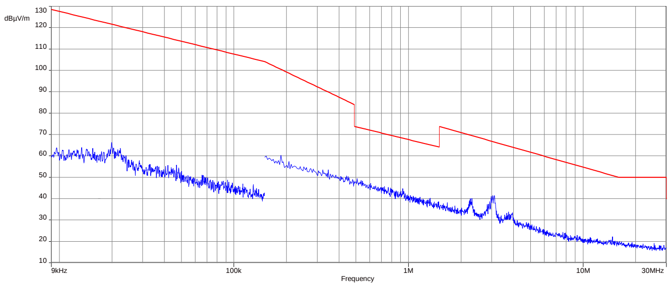
Plot 28: 9 kHz to 30 MHz, U-NII-2A; highest channel
