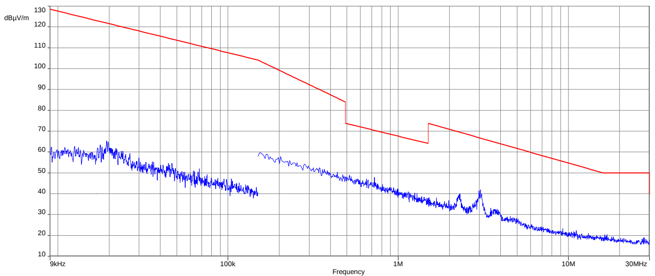
Plot 42: 9 kHz to 30 MHz, U-NII-3; lowest channel
