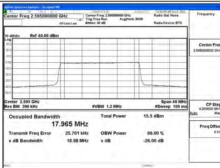
Band38-20MHz-16QAM-38150-100RB#0
