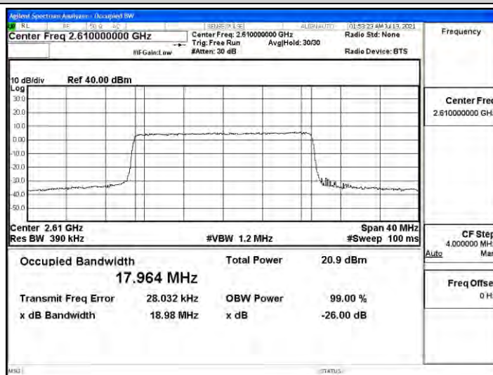
Band38-20MHz-16QAM-38150-100RB#0
