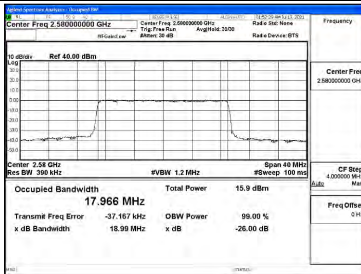
Band38-20MHz-16QAM-38000-100RB#0
