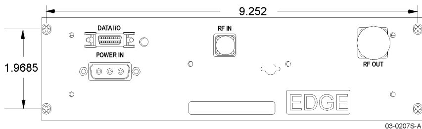
Figure 1-1. SCA9323-30C Amplifier
