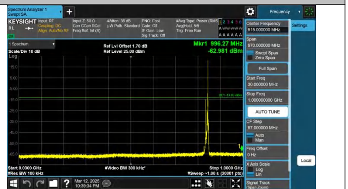
Band5-10MHz-QPSK-20600-1RB#49-30~1000-PASS
