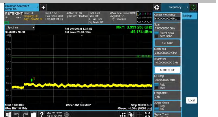
Band5-5MHz-QPSK-20525-1RB#24-3000~10000-PASS
