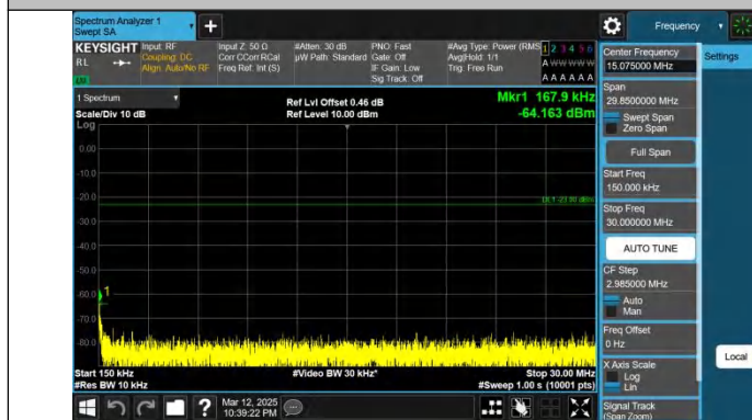
Band5-10MHz-QPSK-20600-1RB#49-0.15~30-PASS
