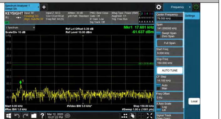
Band5-5MHz-QPSK-20525-1RB#24-0.009~0.15-PASS
