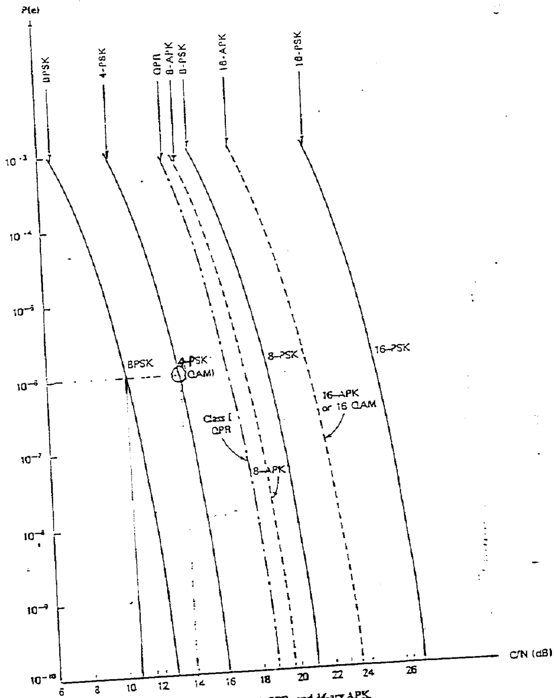
Fig. 3.11. P(e) performance of M -ary PSK, QAM, QPSK, and M -ary APK coherent systems. The rms C/N is specified in the double-sided Nyquist bandwidth.
